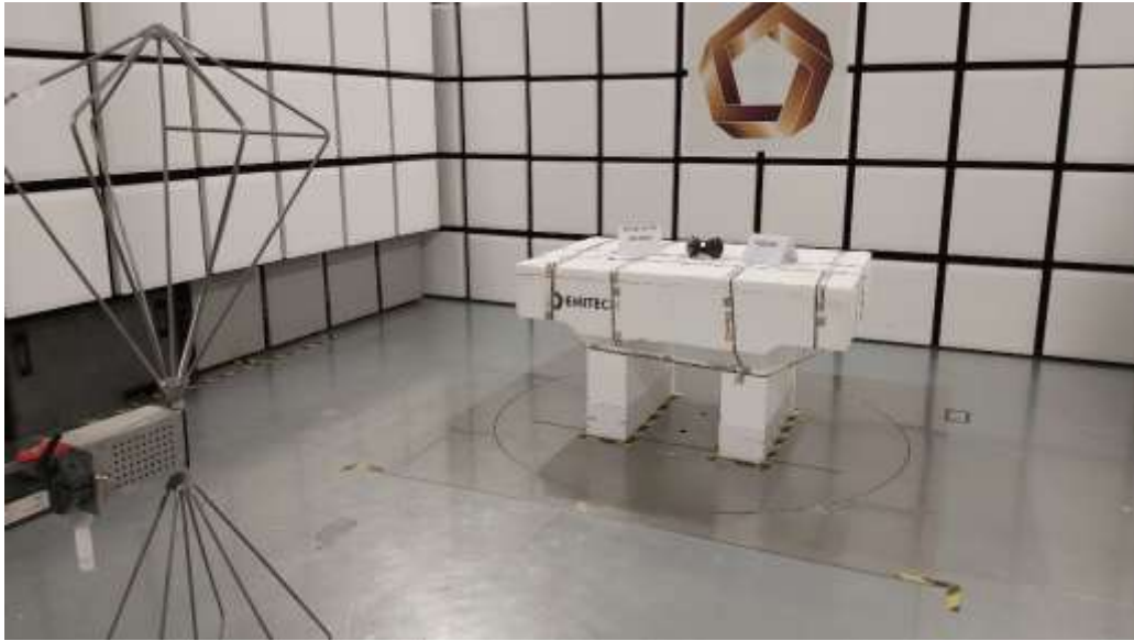
TEST SETUP PHOTO(S) – RX MODE – 30MHZ TO 200MHZ
