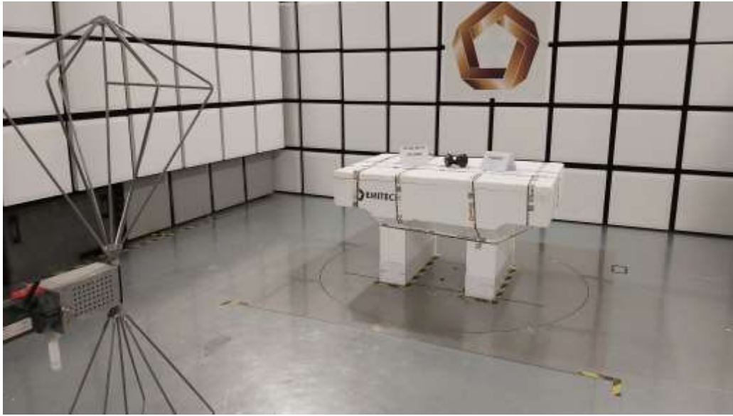
TEST SETUP PHOTO(S) – TX MODE – 30MHZ TO 200MHZ
