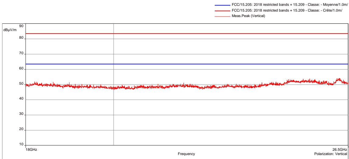
Charging + Tx mode / All Positions / Low channel / 18GHz to 26.5GHz - 7283
