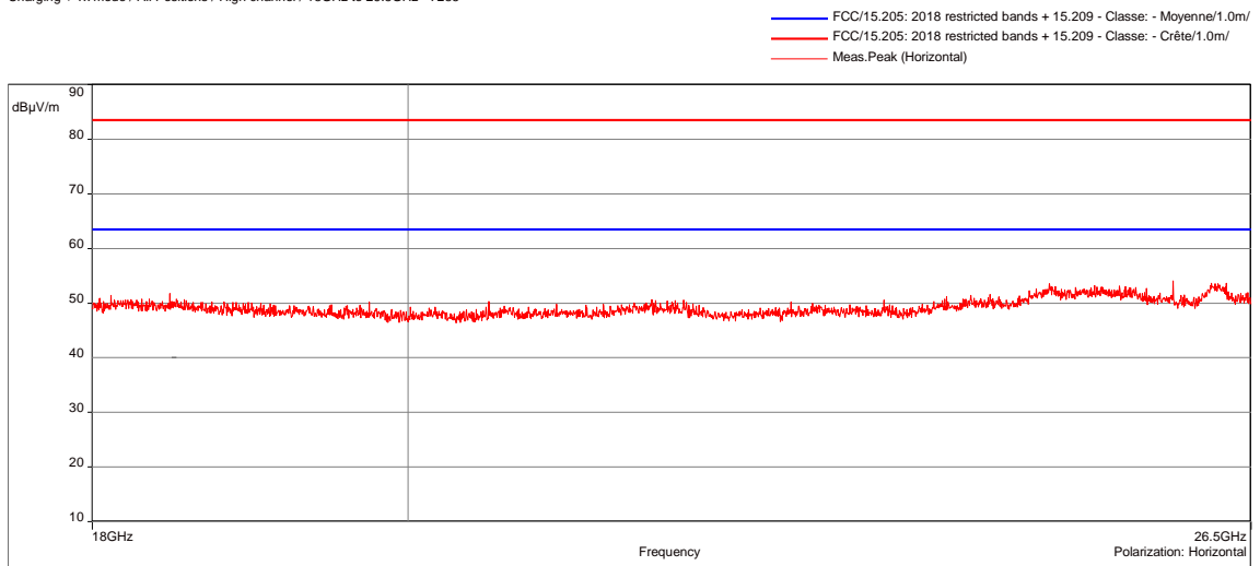
Charging + Tx mode / All Positions / High channel / 18GHz to 26.5GHz - 7285
