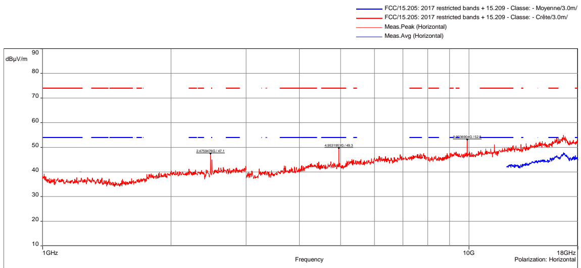
Tx mode / All Positions / High channel / 1GHz to 18GHz - 7192
