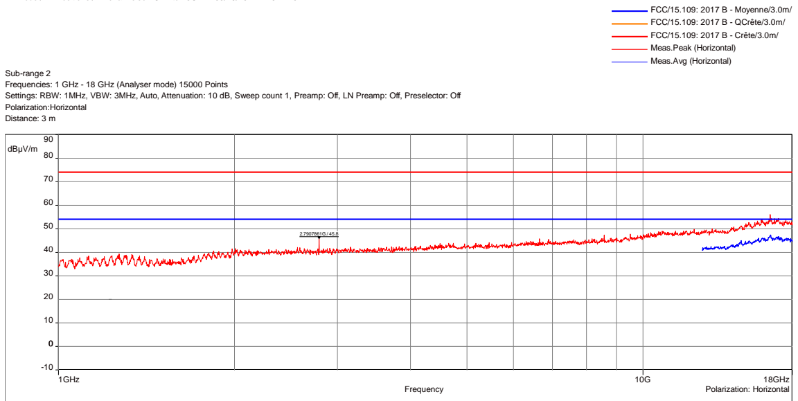
Rx mode / All Positions / All channels / 1GHz to 18GHz - 03/26/2021 11:52 - 7071
