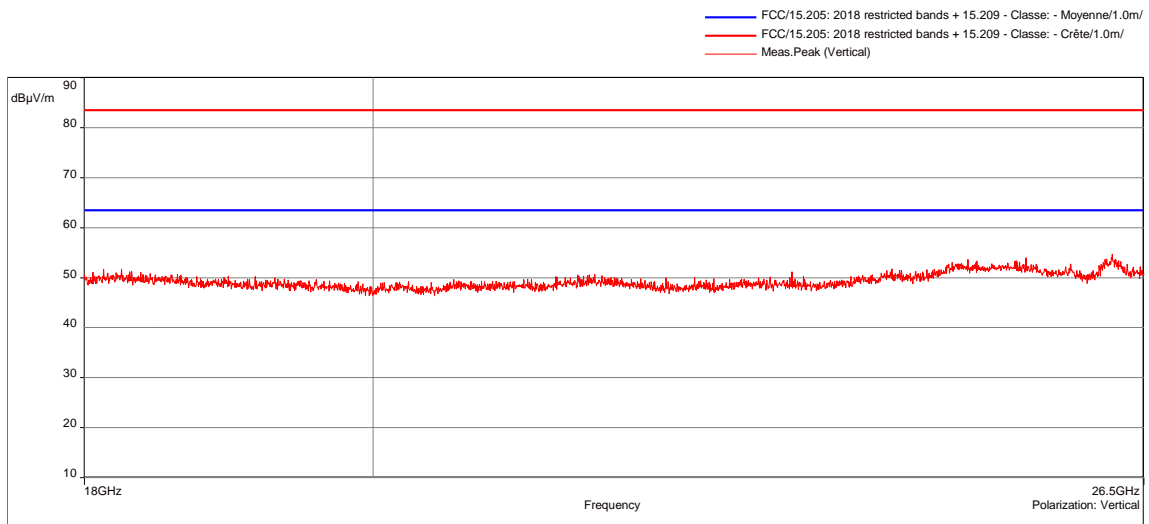
Tx mode / All Positions / High channel / 18GHz to 26.5GHz - 7244
