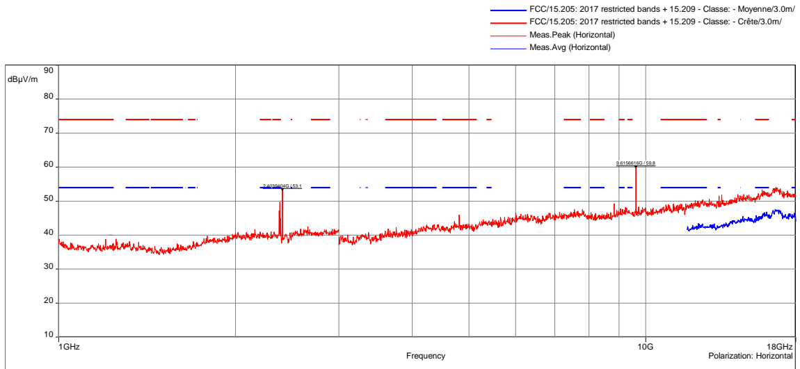
Tx mode / All Positions / Low channel / 1GHz to 18GHz - 7190
