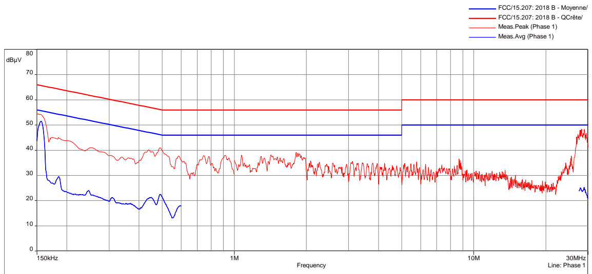
120Vac/60Hz power supply / All channels - 05/05/2021 09:03 - 7577
