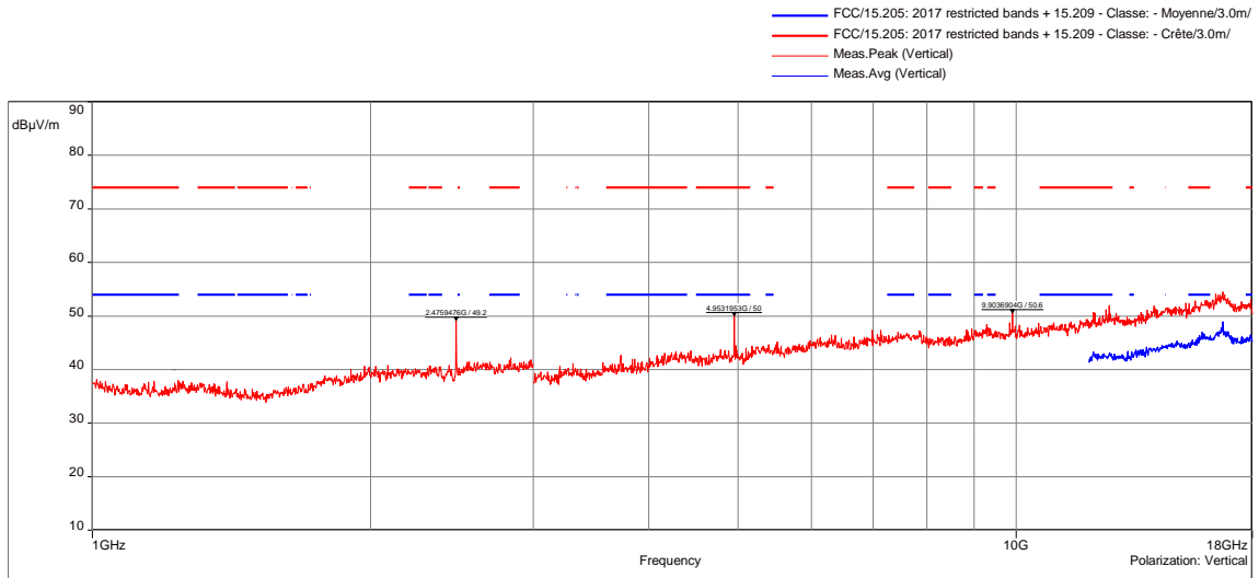
Tx mode / All Positions / High channel / 1GHz to 18GHz - 7192
