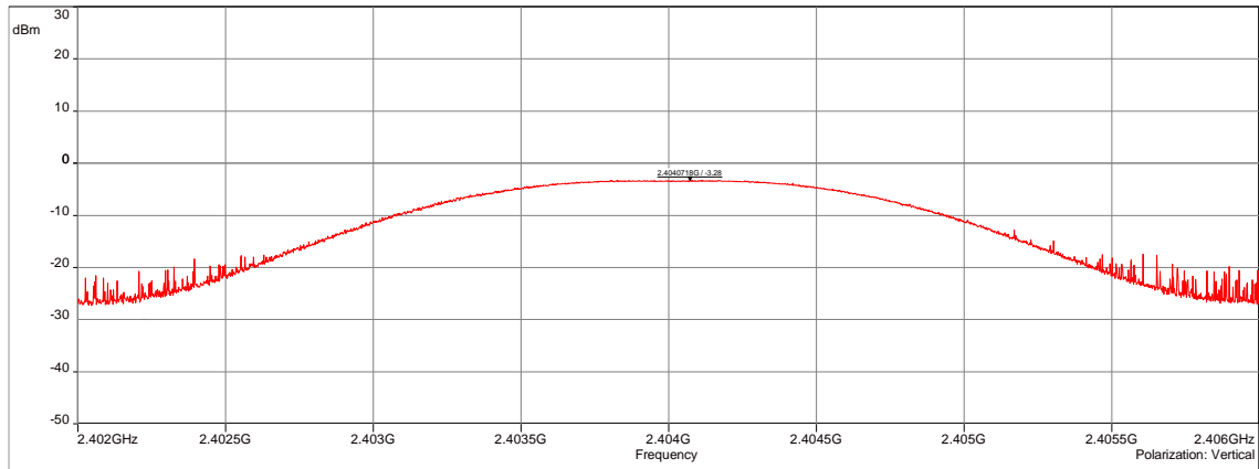
EIRP / All Positions / Low channel - 02/23/2021 09:12 - 6671
