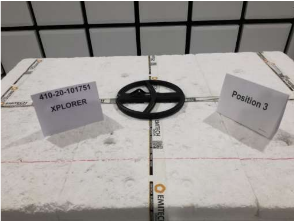
TEST SETUP PHOTO(S) - TX MODE - POSITION 3
