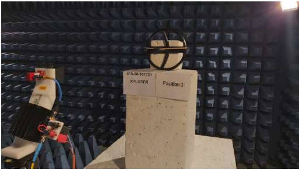
TEST SETUP PHOTO(S) - TX MODE / 18GHZ TO 26.5GHZ
