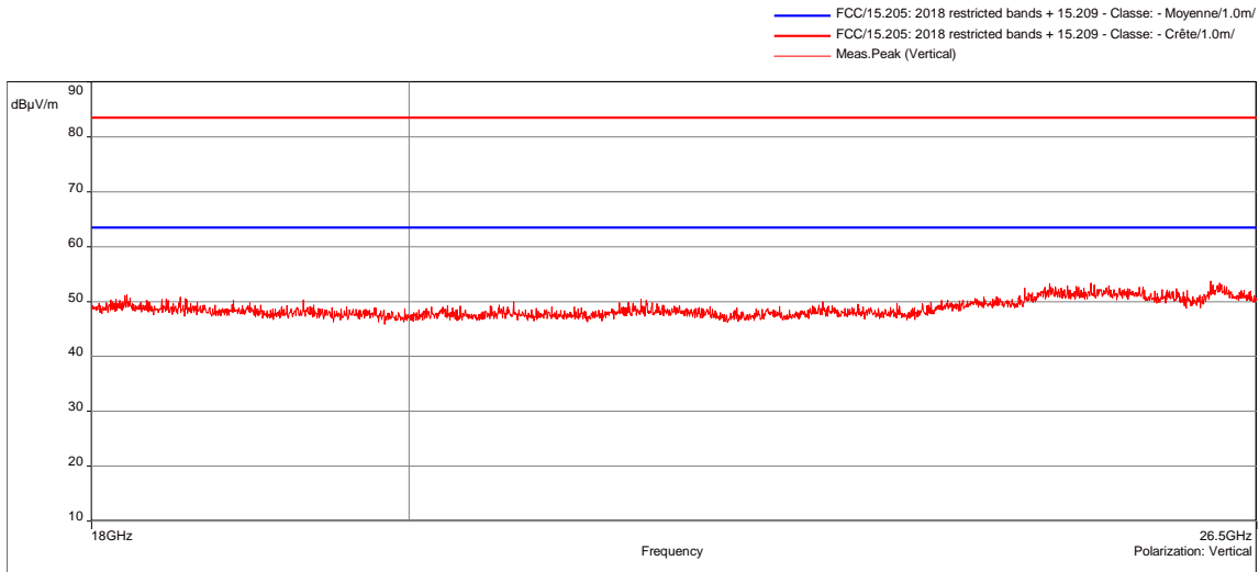
Charging + Tx mode / All Positions / High channel / 18GHz to 26.5GHz - 7276
