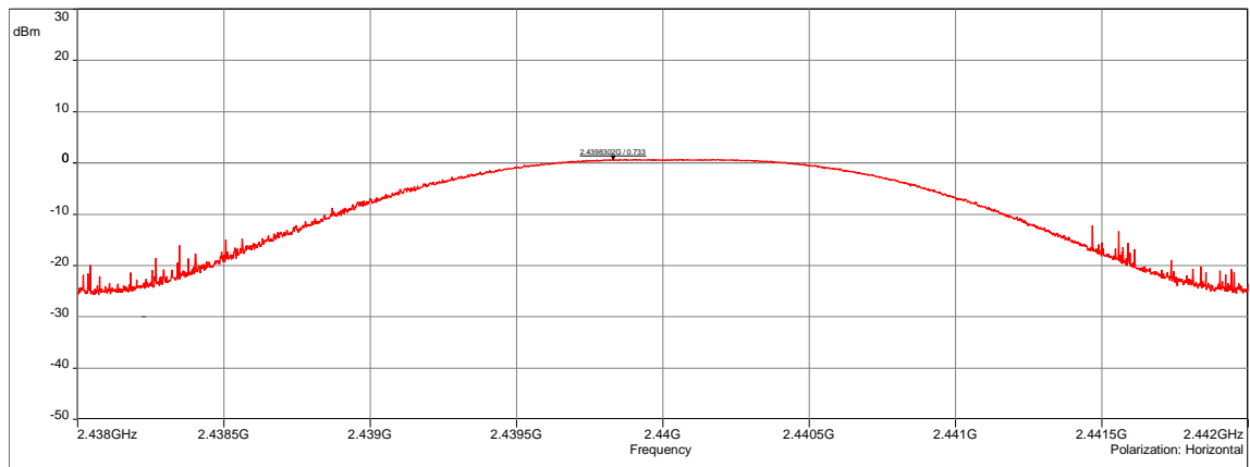
EIRP / All Positions / Mid channel - 03/03/2021 10:58 - 6693
