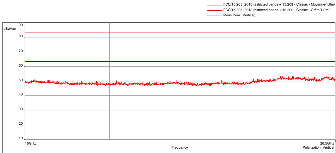
Charging + Tx mode / All Positions / Mid channel / 18GHz to 26.5GHz - 7275
