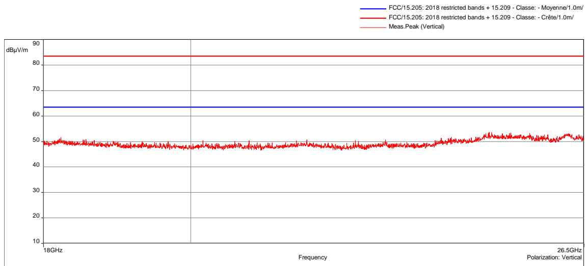
Tx mode / All Positions / Mid channel / 18GHz to 26.5GHz - 6775
