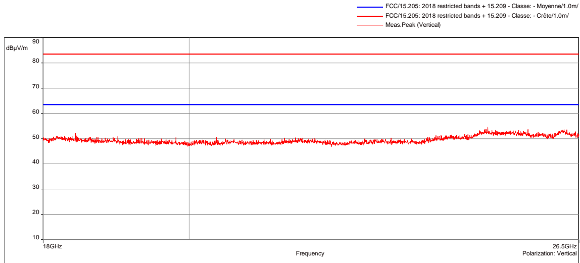
Tx mode / All Positions / Low channel / 18GHz to 26.5GHz - 6772
