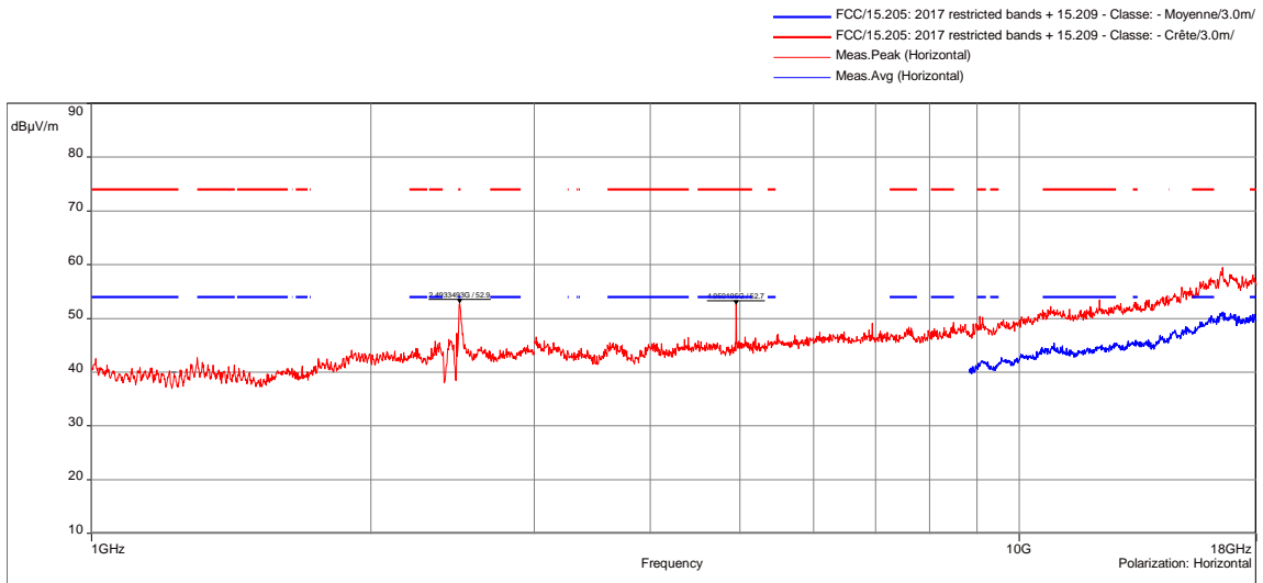
Tx mode / All Positions / High channel / 1GHz to 18GHz - 6751
