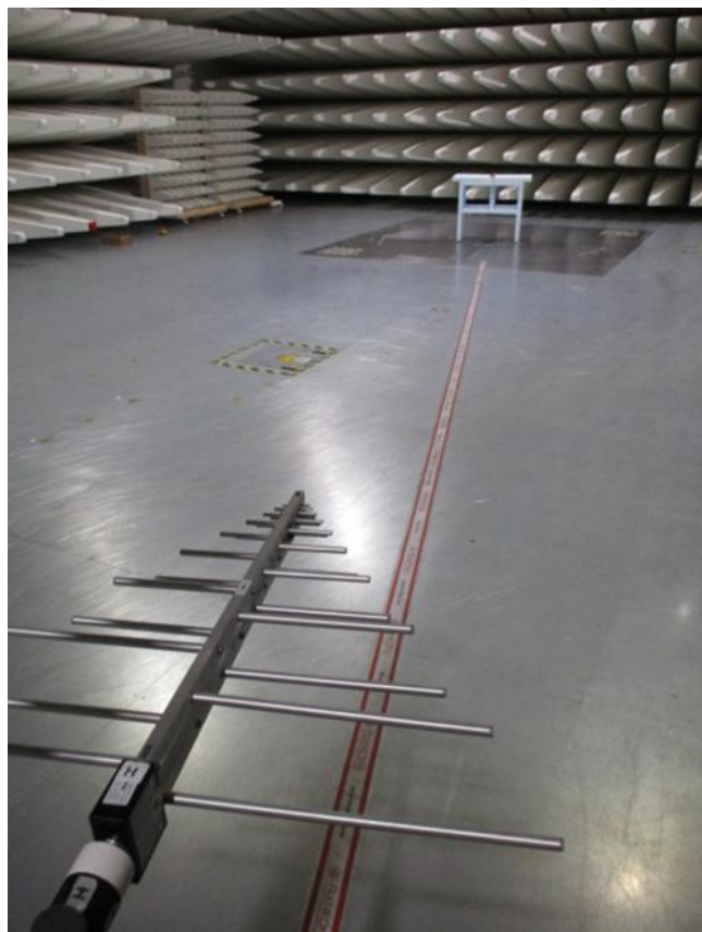
Spurious Radiated Emissions and Emission bandwidth test set-up in frequency range 230-1000 MHz
