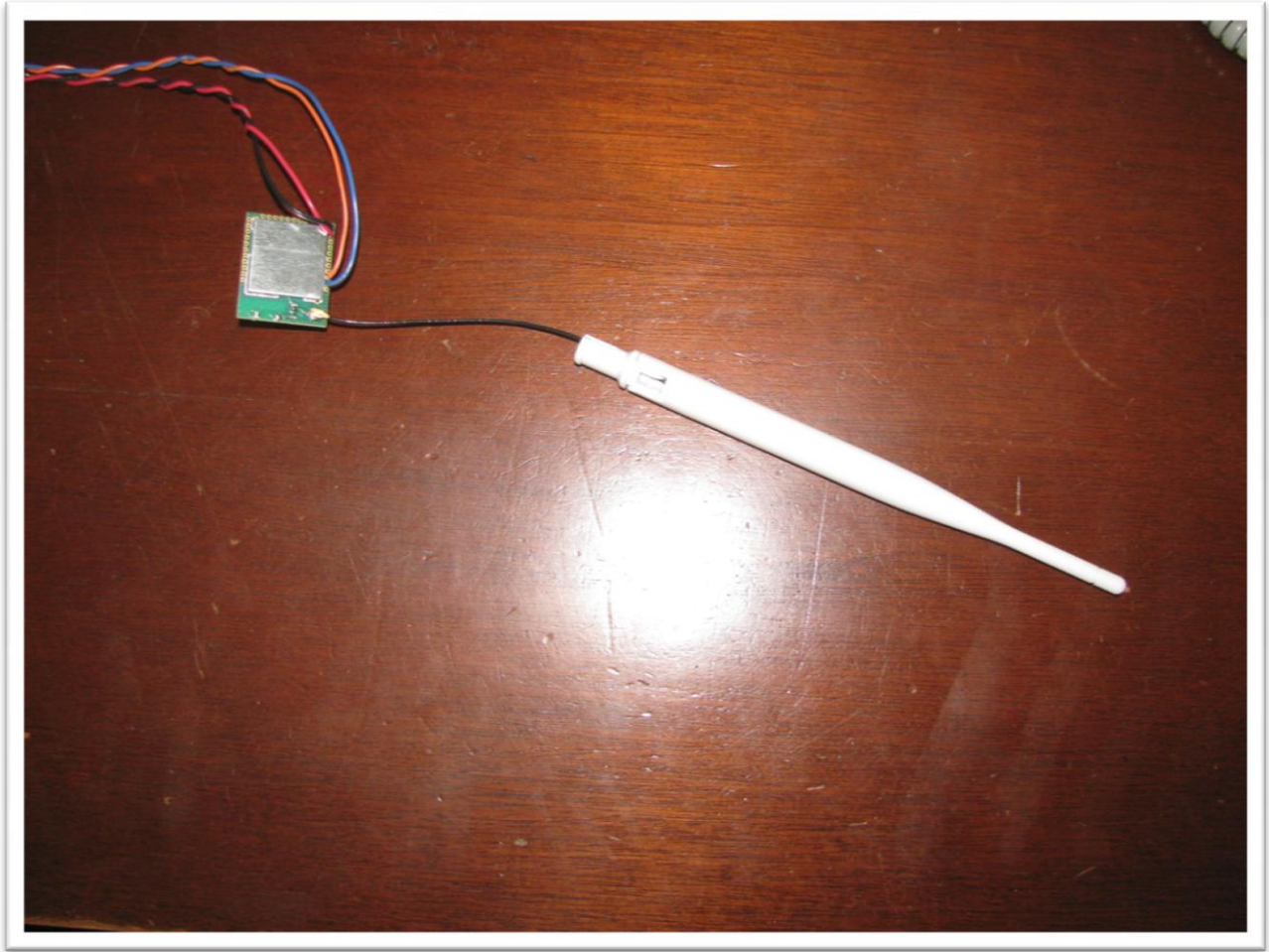
Figure 2 – EUT with External whip antenna
