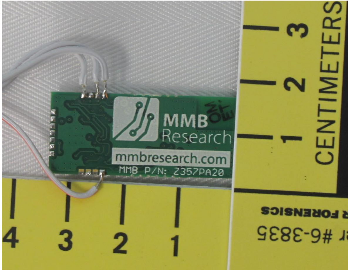
Illustration 2: EUT rear view
