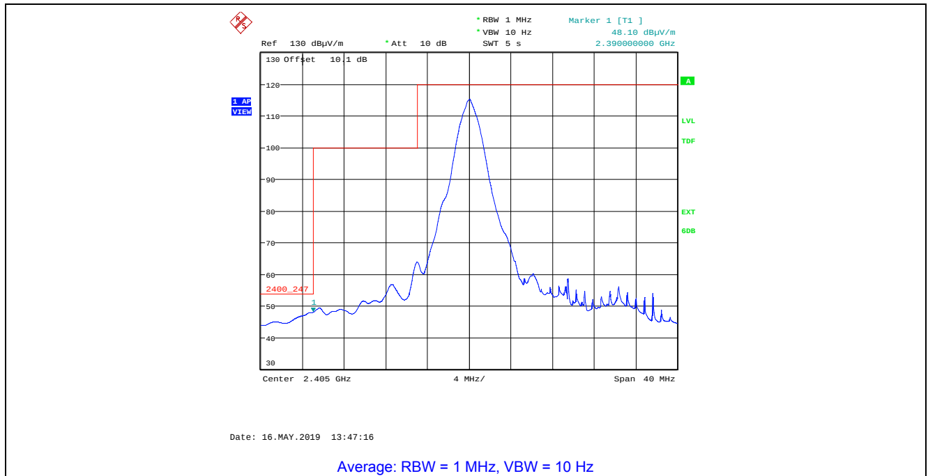
Plot 5.4.4.2.4. Band-Edge Radiated Emissions, Lower Band- edge Rx Antenna in Horizontal Polarization, O-QPSK Modulation, Power Setting 15, Ch 11, 2405 MHz
