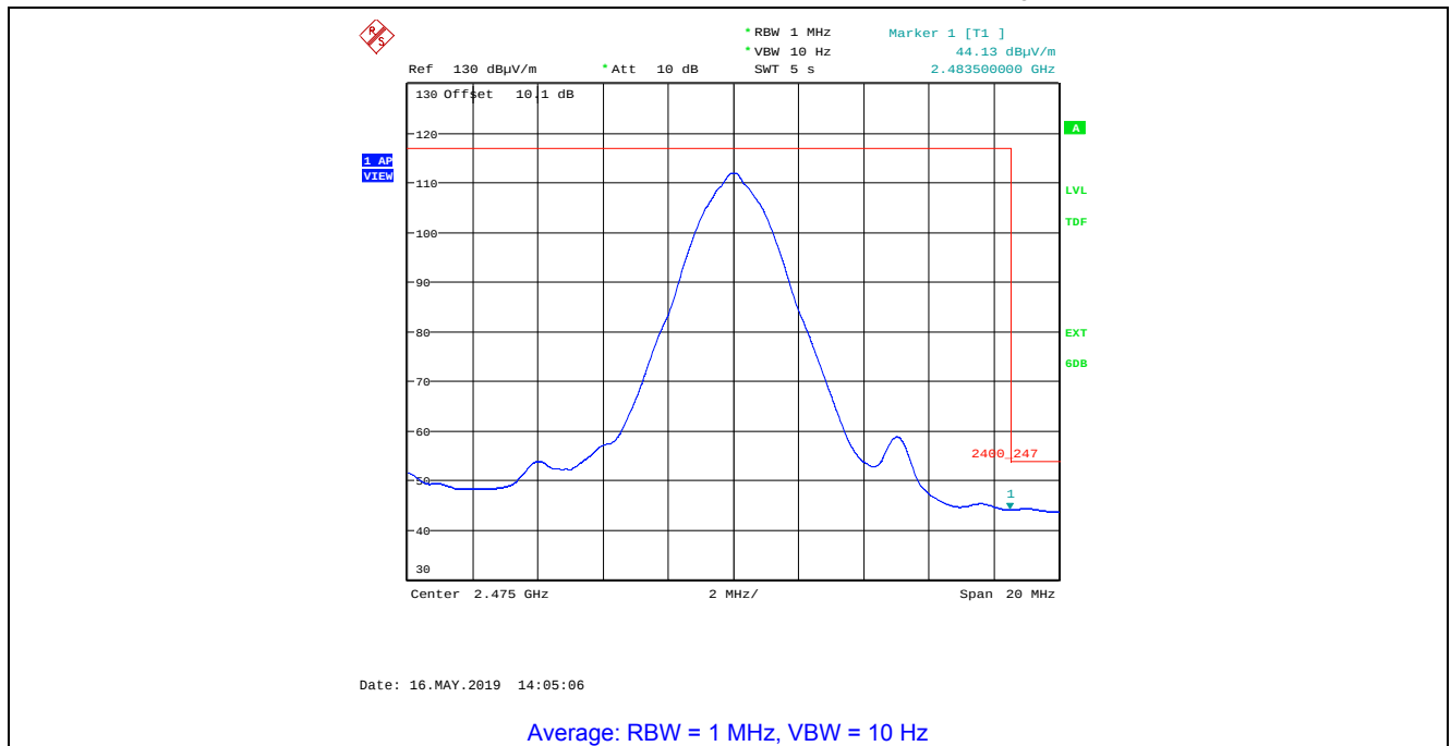
Plot 5.4.4.2.8. Band-Edge Radiated Emissions, Higher Band-edge Rx Antenna in Horizontal Polarization, O-QPSK Modulation, Power Setting 15, Ch 25, 2475 MHz
