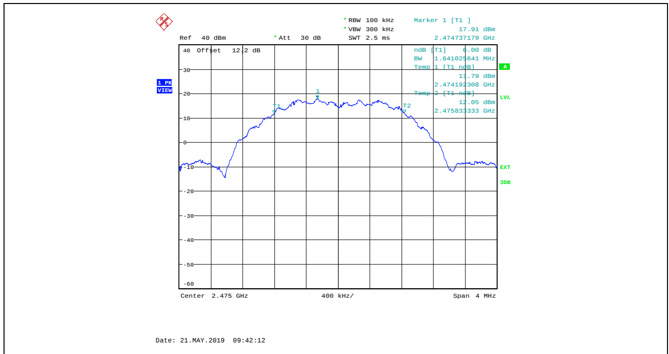
Plot 5.2.4.3. 6 dB Bandwidth, O-QPSK Modulation, Power Setting at 15, Channel 25, 2475 MHz
