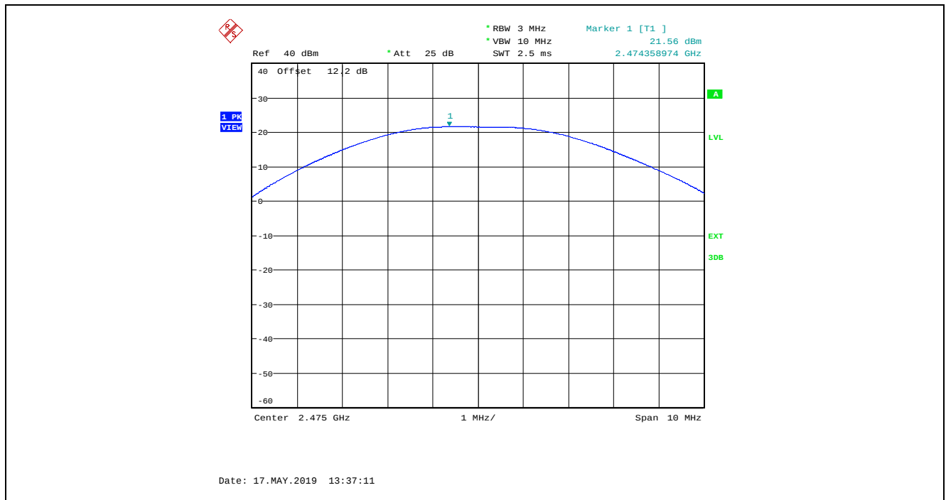
Plot 5.3.4.3. Maximum Peak Conducted Output Power, O-QPSK Modulation, Power Setting 15, Ch 25, 2475 MHz
