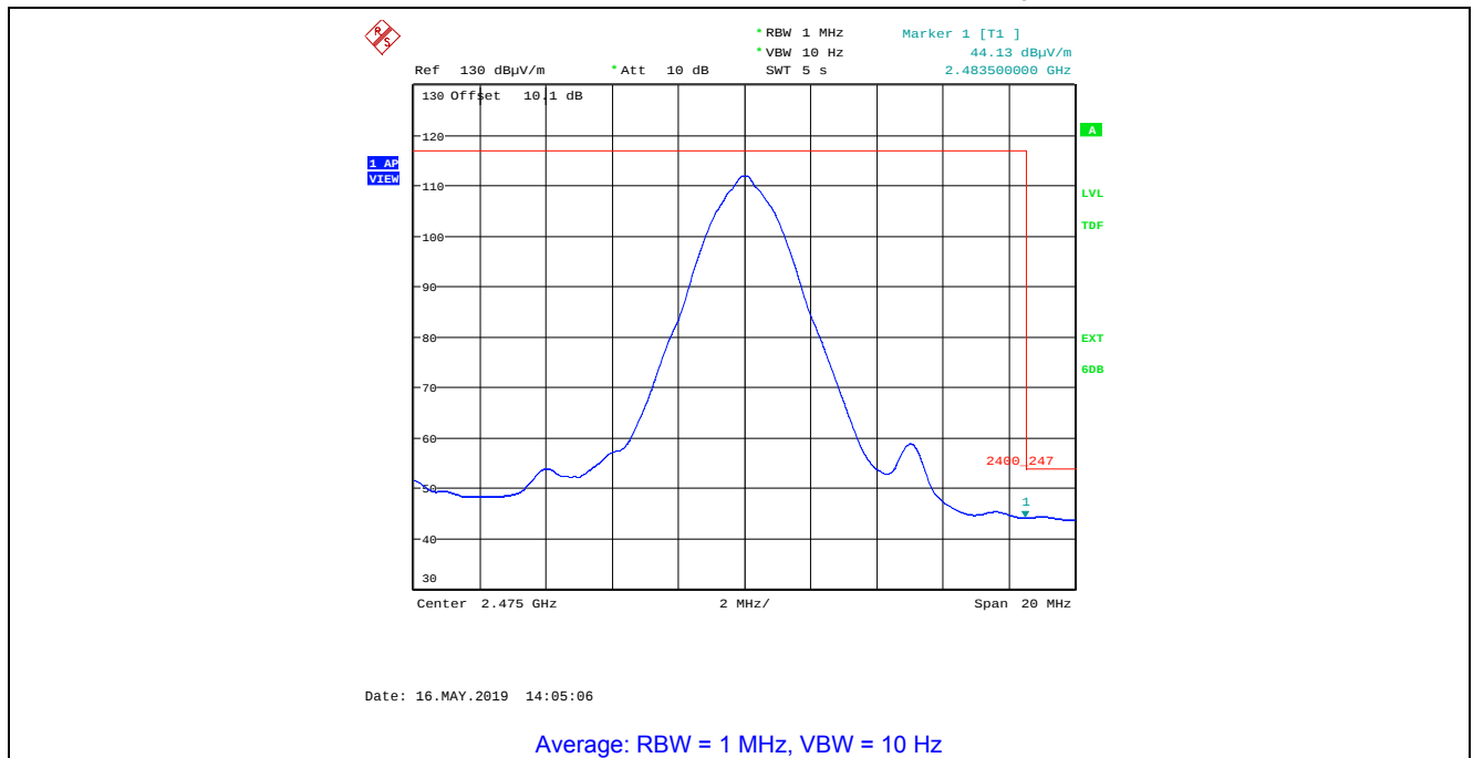
Plot 5.4.4.2.6. Band-Edge Radiated Emissions, Higher Band-edge Rx Antenna in Vertical Polarization, O-QPSK Modulation, Power Setting 15, Ch 25, 2475 MHz
