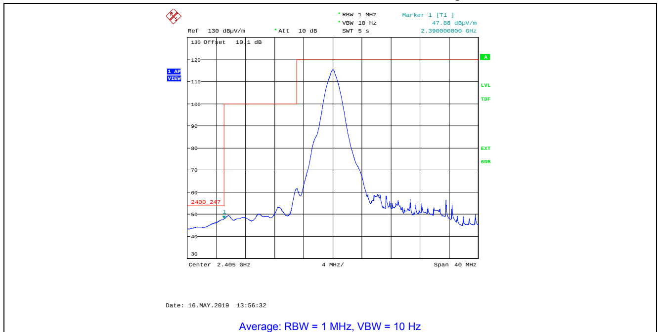
Plot 5.4.4.2.2. Band-Edge Radiated Emissions, Lower Band- edge Rx Antenna in Vertical Polarization, O-QPSK Modulation, Power Setting 15, Ch 11, 2405 MHz
