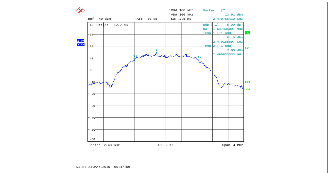
Plot 5.2.4.4. 6 dB Bandwidth, O-QPSK Modulation, Power Setting at 12, Channel 26, 2480 MHz
