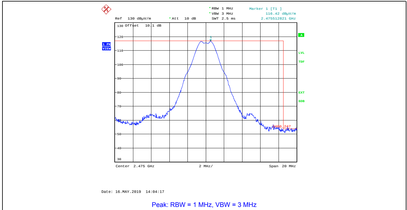
Plot 5.4.4.2.7. Band-Edge Radiated Emissions, Higher Band-edge Rx Antenna in Horizontal Polarization, O-QPSK Modulation, Power Setting 15, Ch 25, 2475 MHz
