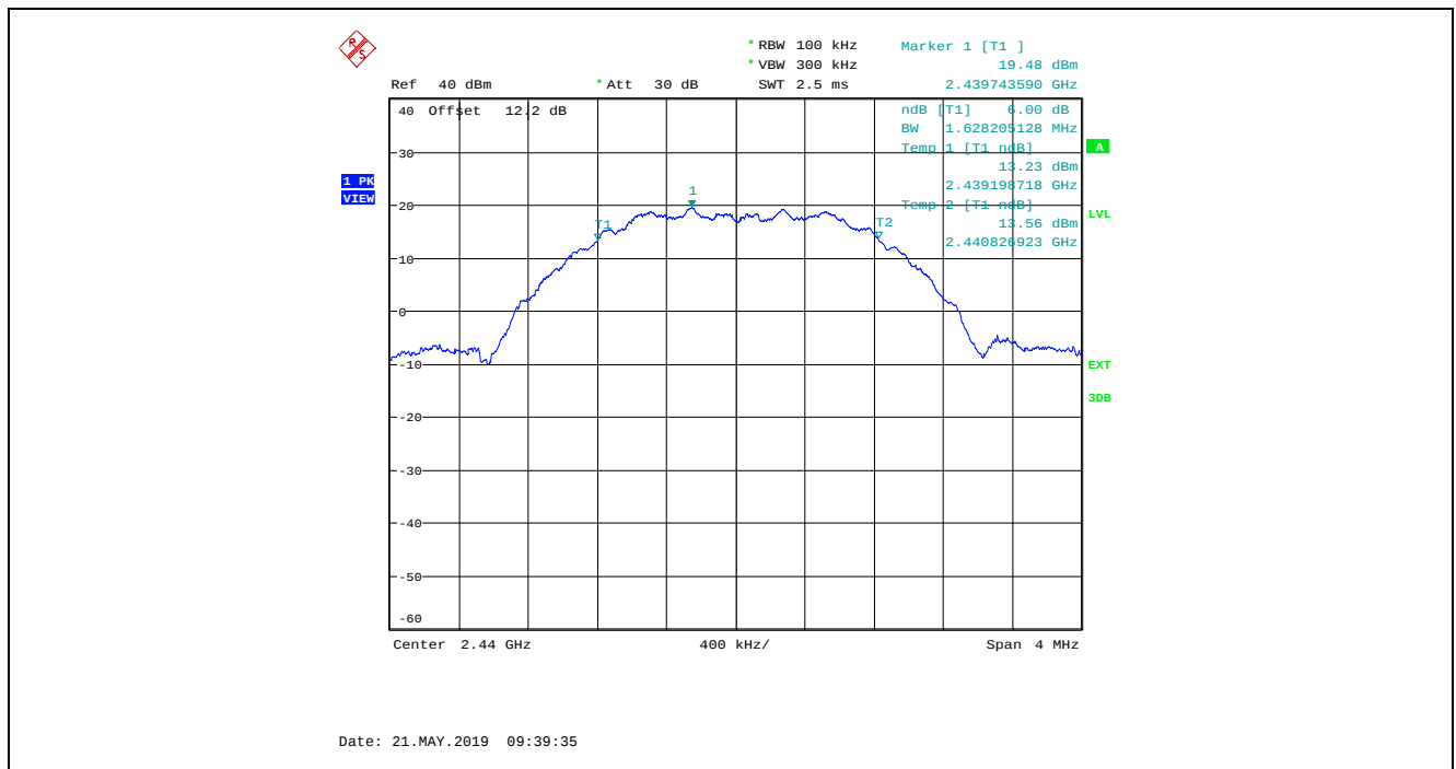
Plot 5.2.4.2. 6 dB Bandwidth, O-QPSK Modulation, Power Setting at 15, Channel 18, 2440 MHz
