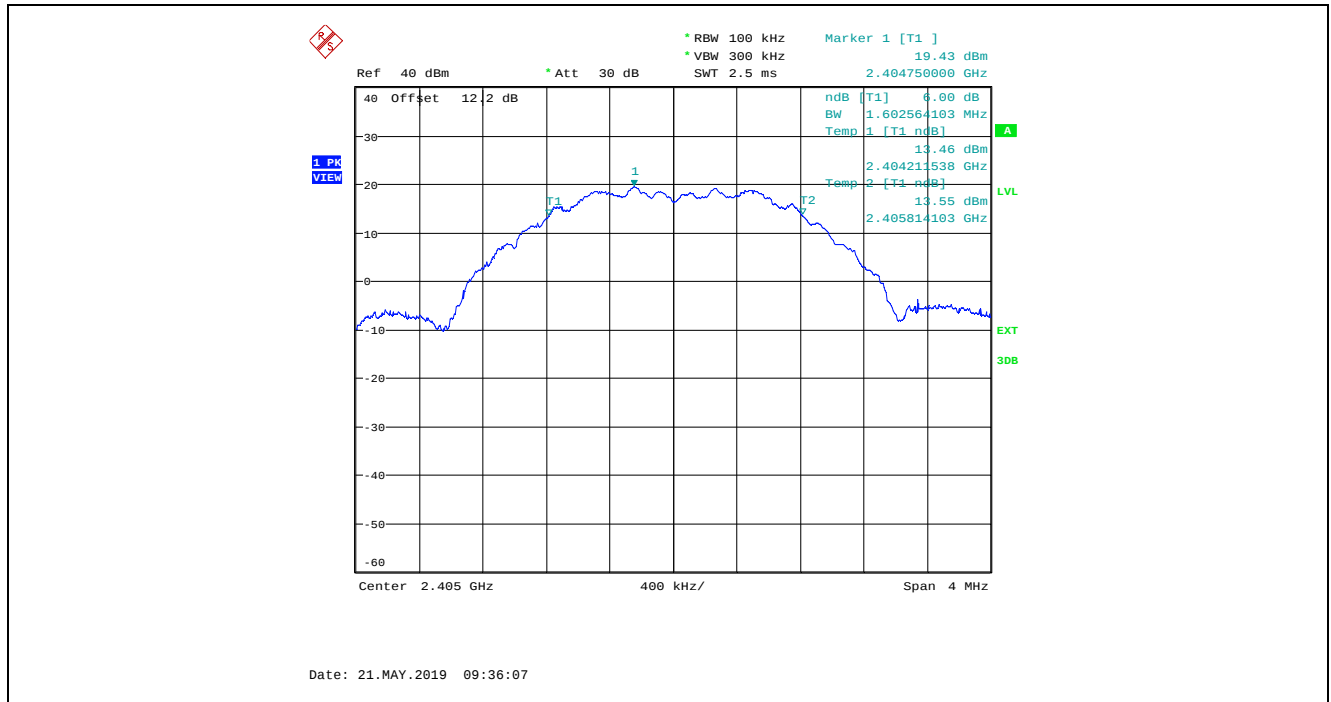
Plot 5.2.4.1. 6 dB Bandwidth, O-QPSK Modulation, Power Setting at 15, Channel 11, 2405 MHz
