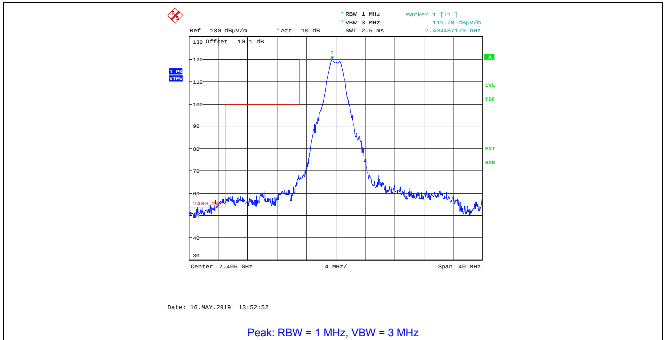
Plot 5.4.4.2.1. Band-Edge Radiated Emissions, Lower Band-edge Rx Antenna in Vertical Polarization, O-QPSK Modulation, Power Setting 15, Ch 11, 2405 MHz
