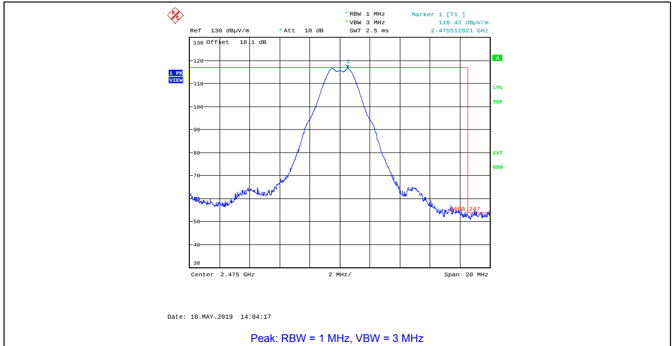
Plot 5.4.4.2.5. Band-Edge Radiated Emissions, Higher Band-edge Rx Antenna in Vertical Polarization, O-QPSK Modulation, Power Setting 15, Ch 25, 2475 MHz
