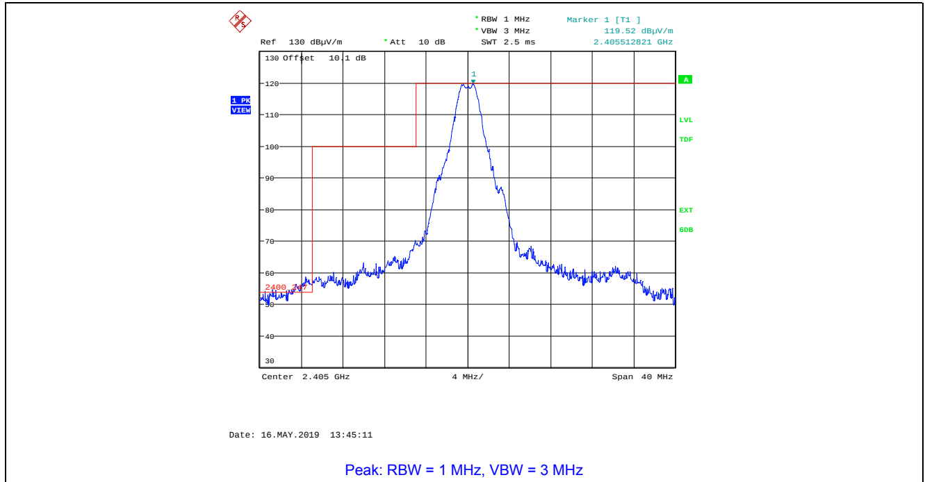
Plot 5.4.4.2.3. Band-Edge Radiated Emissions, Lower Band-edge Rx Antenna in Horizontal Polarization, O-QPSK Modulation, Power Setting 15, Ch 11, 2405 MHz
