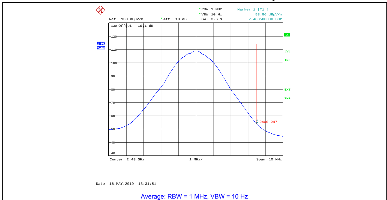
Plot 5.4.4.2.12. Band-Edge Radiated Emissions, Higher Band-edge Rx Antenna in Horizontal Polarization, O-QPSK Modulation, Power Setting 12, Ch 26, 2480 MHz
