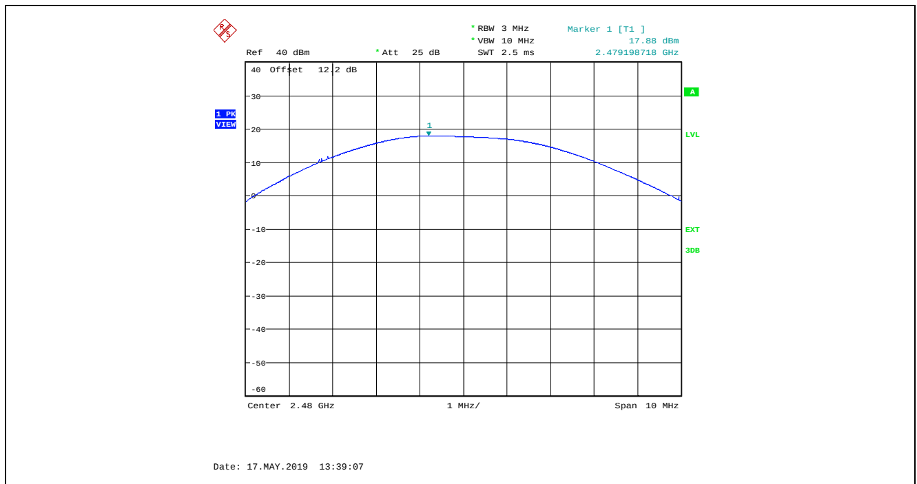
Plot 5.3.4.4. Maximum Peak Conducted Output Power, O-QPSK Modulation, Power Setting 12, Ch 26, 2480 MHz
