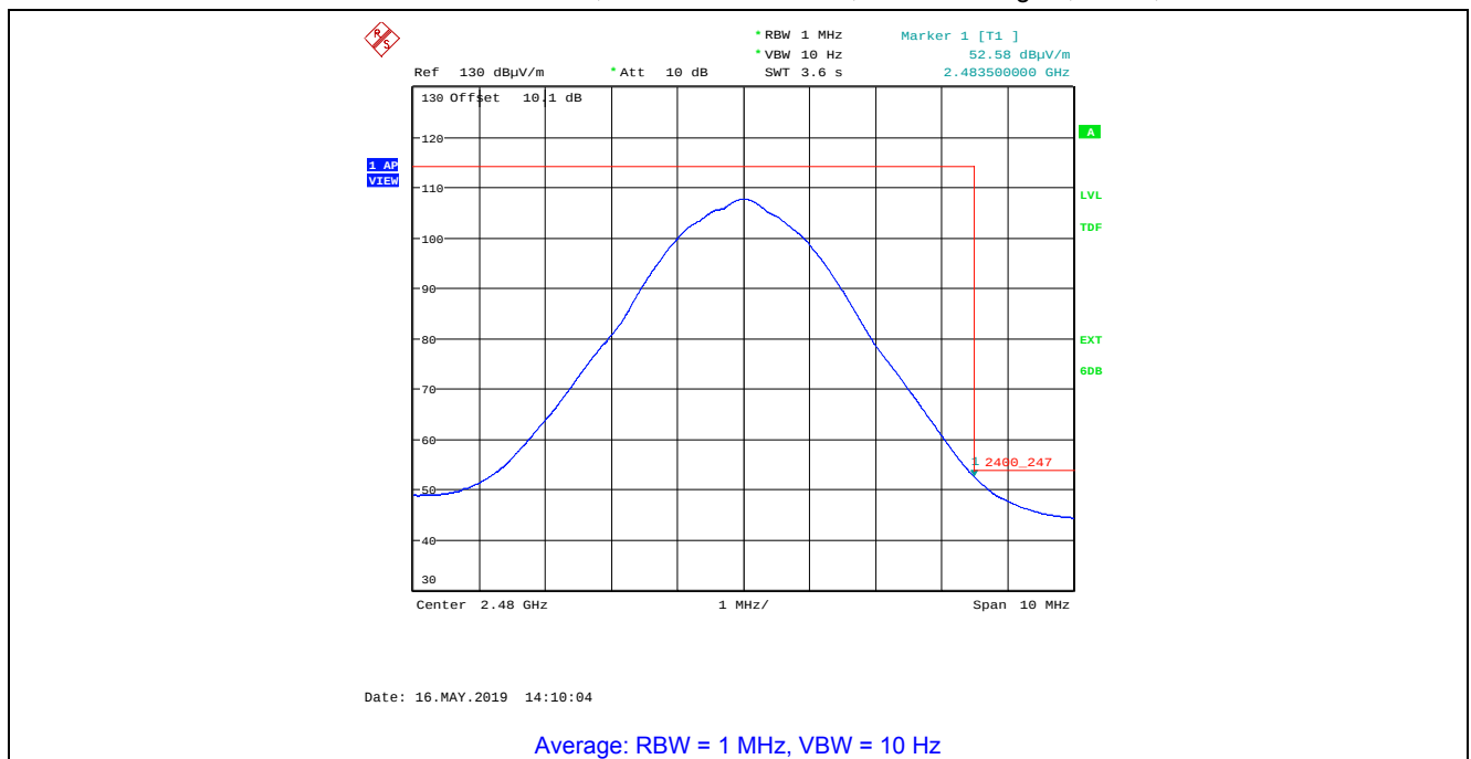
Plot 5.4.4.2.10. Band-Edge Radiated Emissions, Higher Band-edge Rx Antenna in Vertical Polarization, O-QPSK Modulation, Power Setting 12, Ch 26, 2480 MHz
