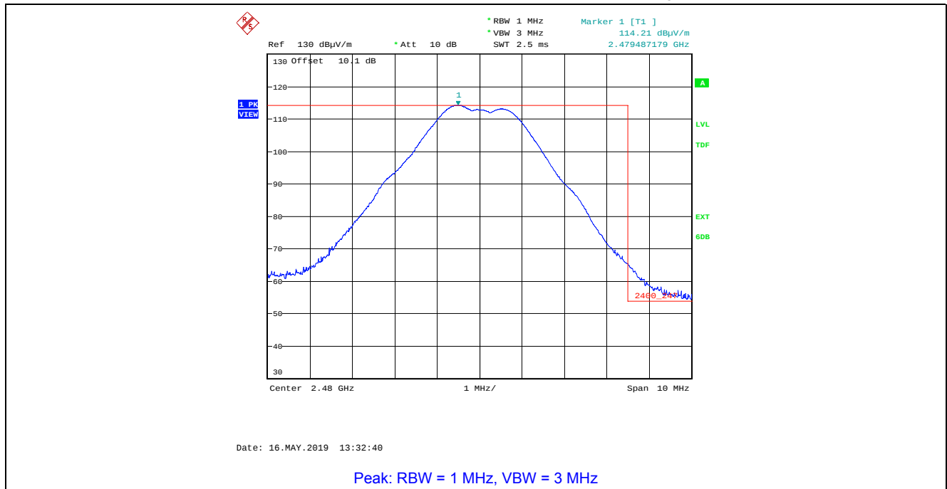
Plot 5.4.4.2.11. Band-Edge Radiated Emissions, Higher Band-edge Rx Antenna in Horizontal Polarization, O-QPSK Modulation, Power Setting 12, Ch 26, 2480 MHz
