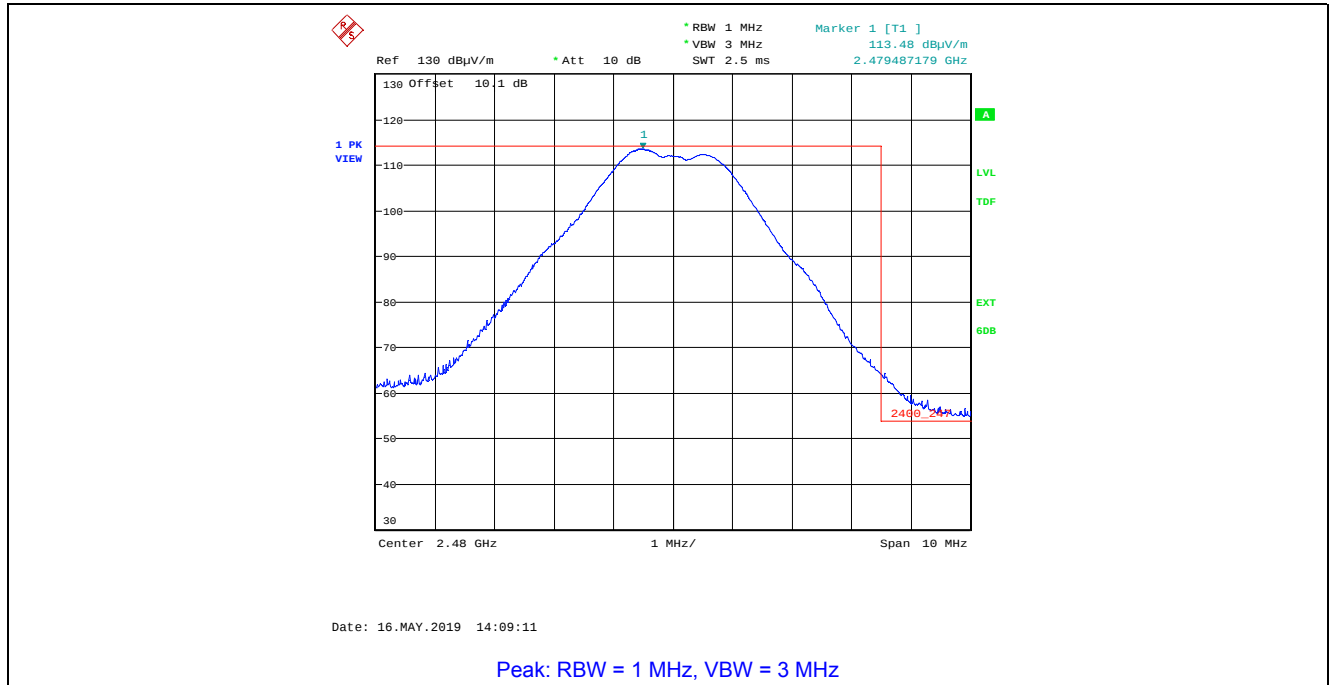
Plot 5.4.4.2.9. Band-Edge Radiated Emissions, Higher Band-edge Rx Antenna in Vertical Polarization, O-QPSK Modulation, Power Setting 12, Ch 26, 2480 MHz
