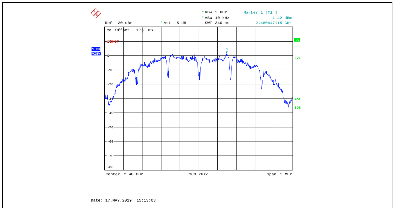
Plot 5.5.4.4. Power Spectral Density, O-QPSK Modulation, Power Setting 12, Channel 26, 2480 MHz
