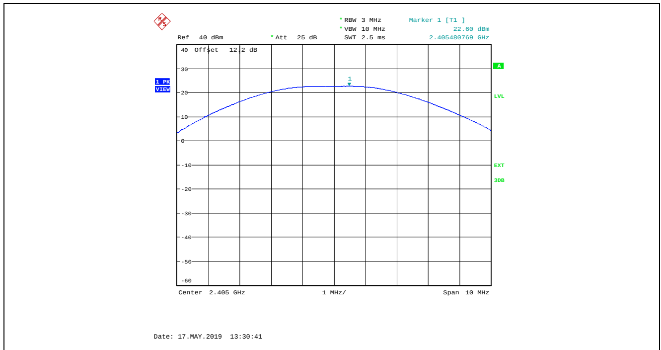
Plot 5.3.4.1. Maximum Peak Conducted Output Power, O-QPSK Modulation, Power Setting 15, Ch 11, 2405 MHz
