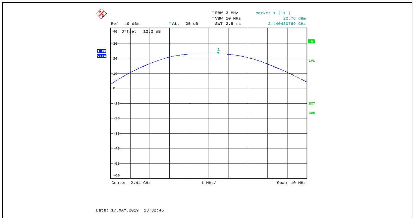
Plot 5.3.4.2. Maximum Peak Conducted Output Power, O-QPSK Modulation, Power Setting 15, Ch 18, 2440 MHz
