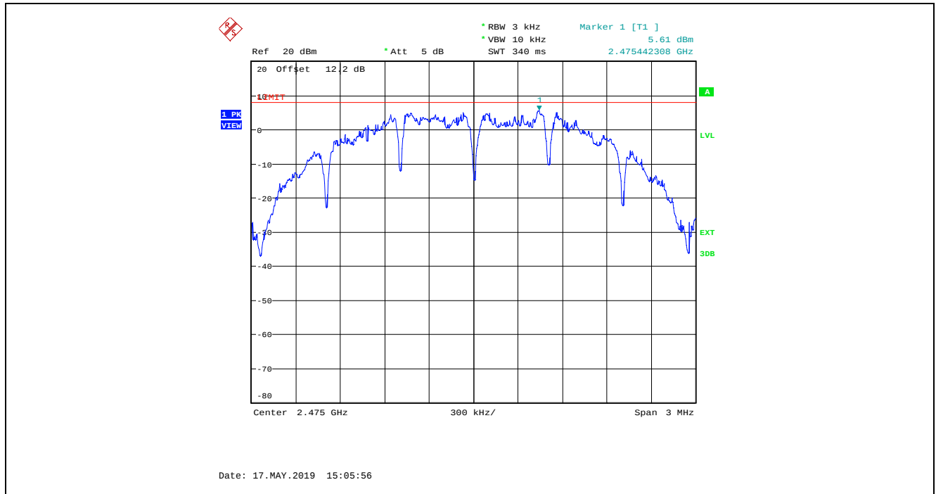
Plot 5.5.4.3. Power Spectral Density, O-QPSK Modulation, Power Setting 15, Channel 25, 2475 MHz
