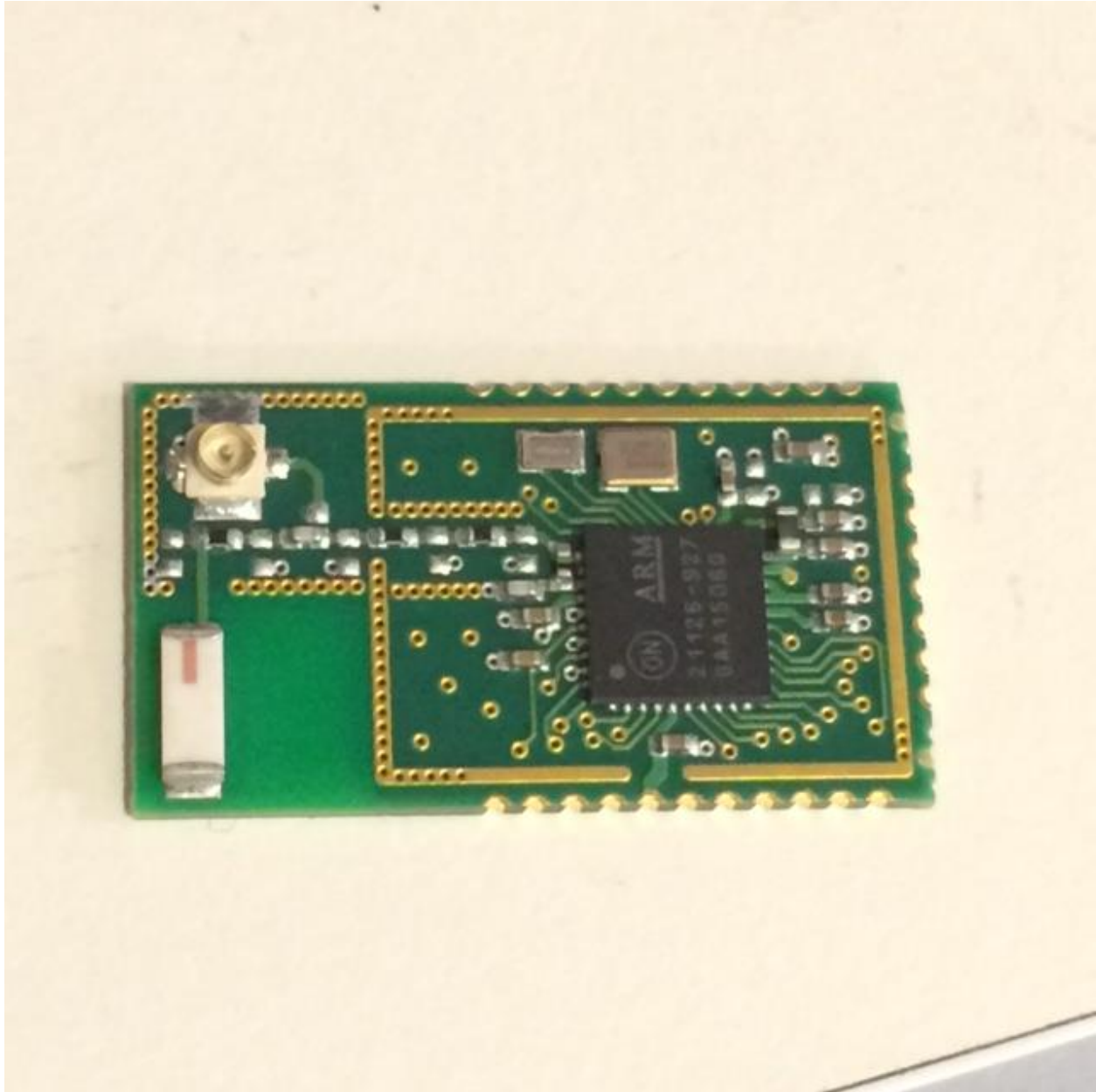
Illustration 1: EUT internal view – top
