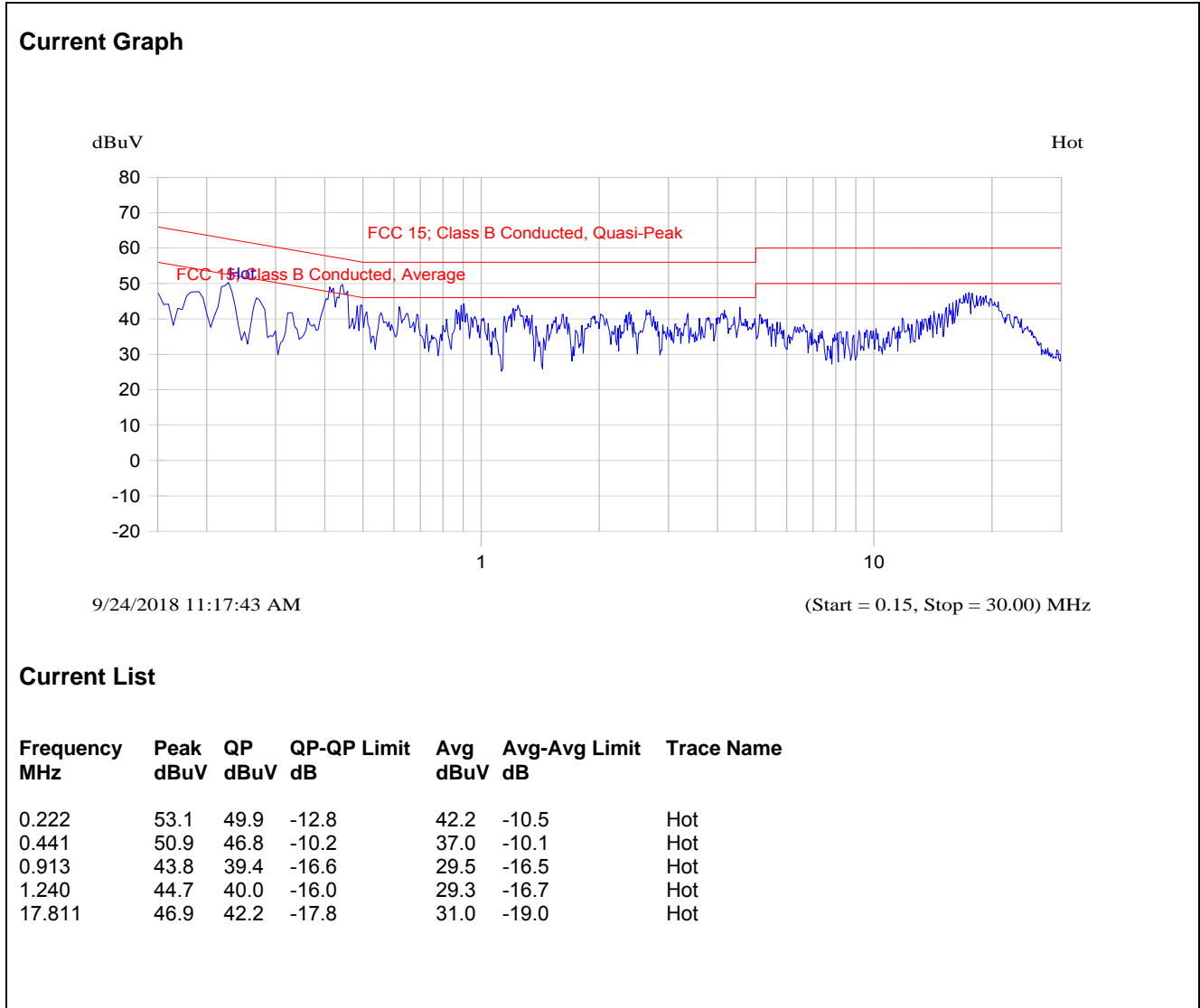
Plot 5.1.4.1. Power Line Conducted Emissions (BLE in Tx Mode) Line Voltage: 120 VAC; Line Tested: Hot
