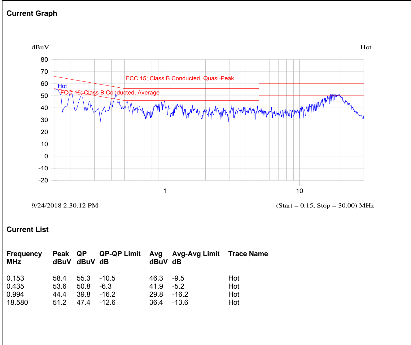
Plot 5.1.4.3. Power Line Conducted Emissions (Rx Mode) Line Voltage: 120 VAC; Line Tested: Hot
