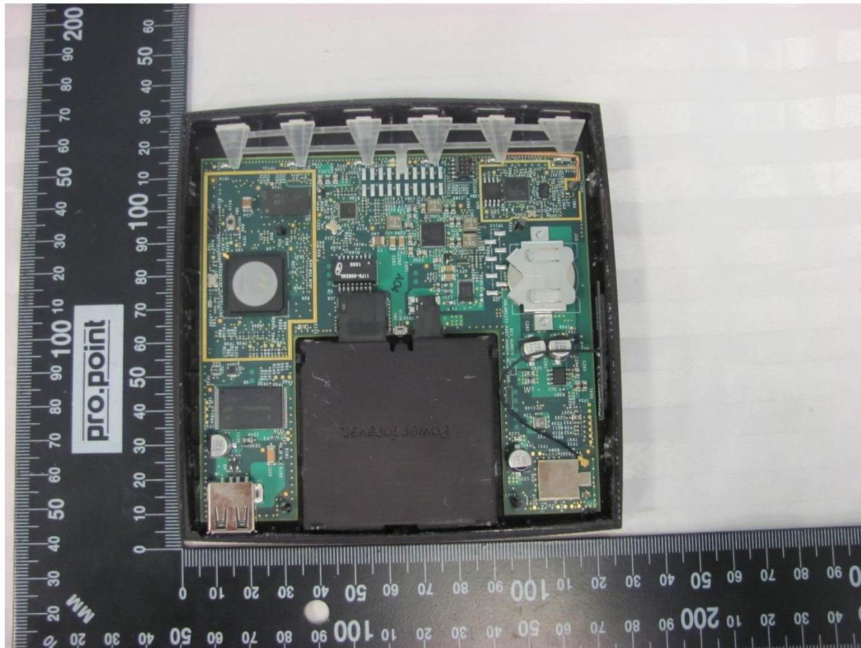
Figure 1: EUT internal top view 1
