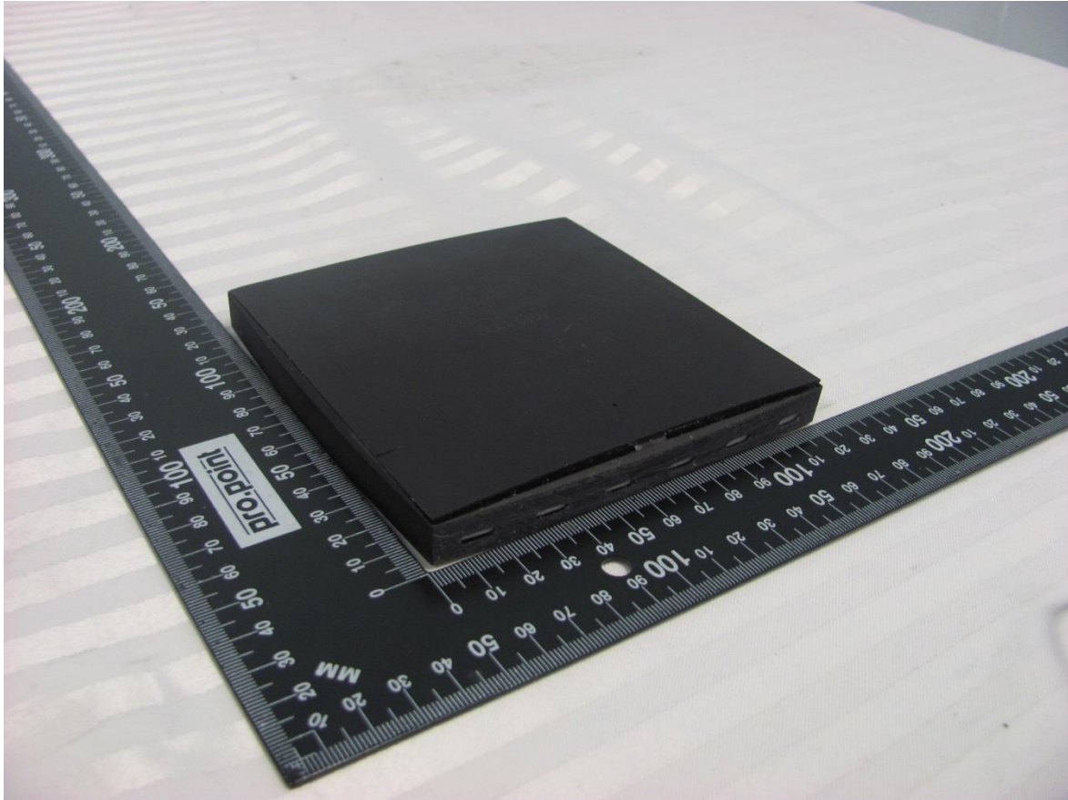
Figure 2: EUT external view
