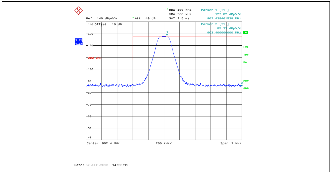
Plot 5.5.4.2.2.17. Band-Edge RF Radiated Emissions at 3 m, Mode 3 (150 kbps), Vertical Polarization Single Frequency Mode, Low End of Frequency Band
