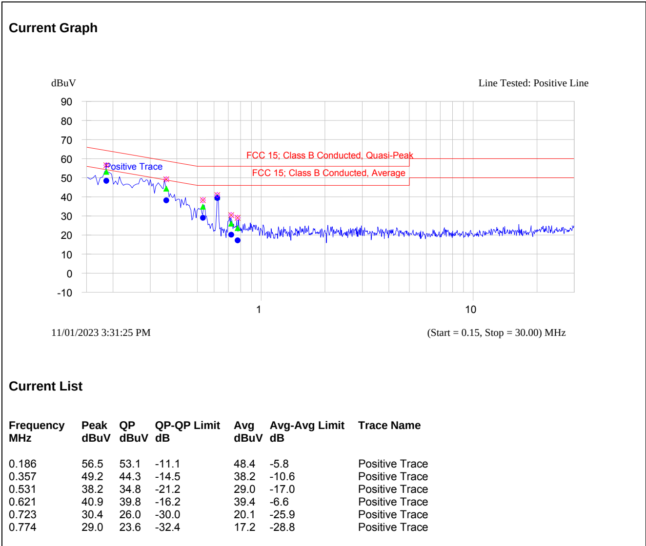
Plot 5.1.4.1. Power Line Conducted Emissions Line Voltage: 5 VDC; Line Tested: Positive
