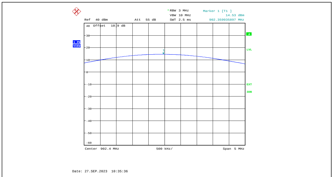
Plot 5.4.4.16. Maximum Peak Conducted Output Power, Mode 3, Raw Power Setting at -10, 902.4 MHz
