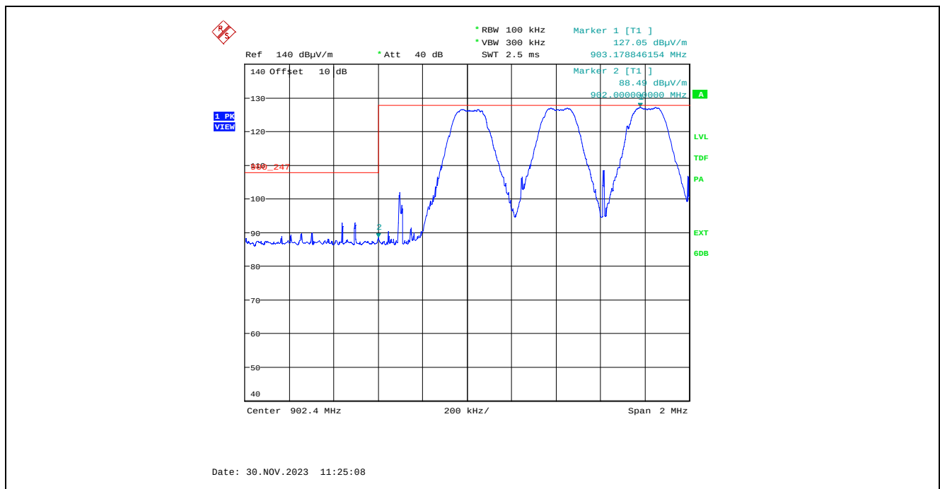
Plot 5.5.4.2.2.18. Band-Edge RF Radiated Emissions at 3 m, Mode 3 (150 kbps), Vertical Polarization Pseudorandom Channel Hopping Mode, Low End of Frequency Band
