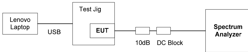
USB provide 5 Vdc and software to operate radio module
