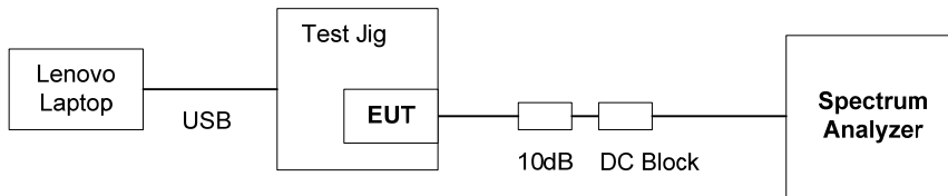
USB provide 5 Vdc and software to operate radio module
