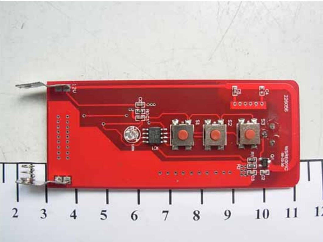
FIGURE 2 EMITTER (M/N: WSRE SERIES) MAIN BOARD (COMPONENT SIDE)
