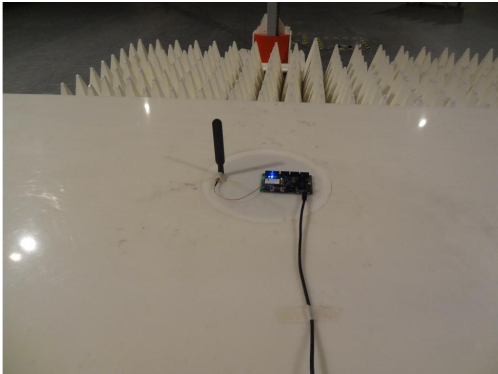
Test Setup – Module on the table (External Antenna)
