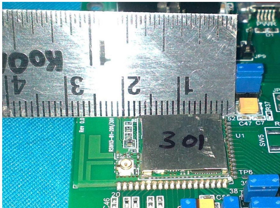
EUT Dimensional View & Redpine Antenna
