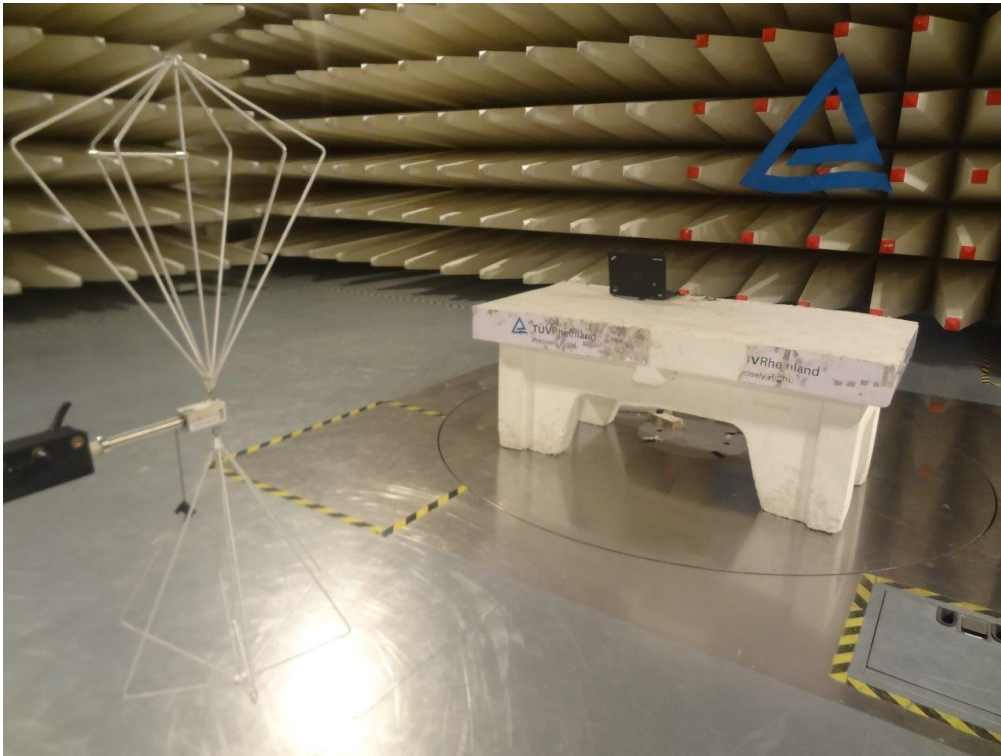
Frequency range:30MHz-200MHz
