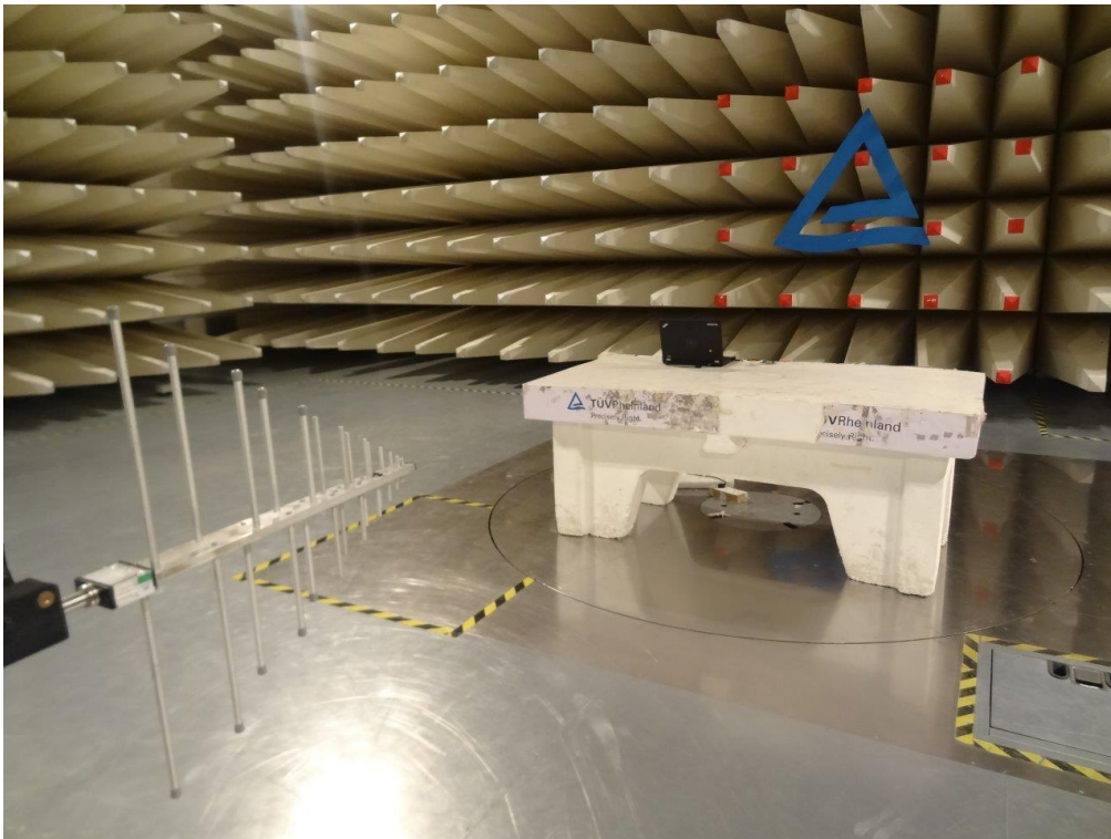
Frequency range:200MHz-1GHz
