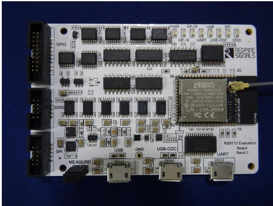
Photo 5: PCB Module
