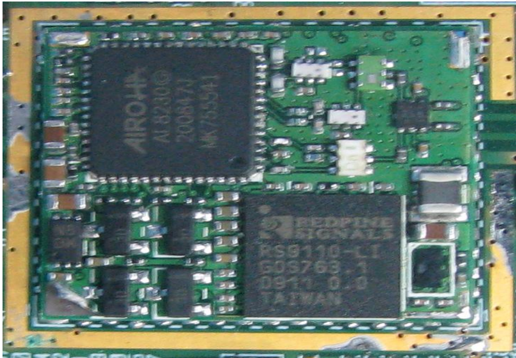
RF Section
