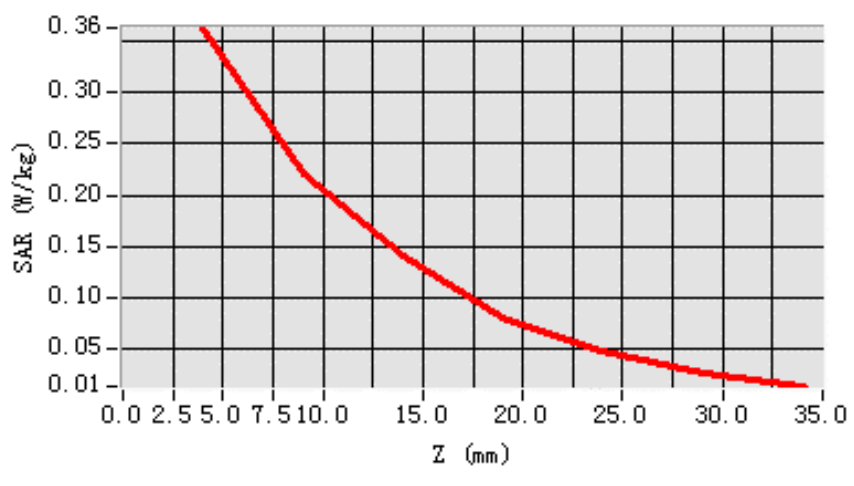
SAR, Z Axis Scan (X = 15, Y = -1)
