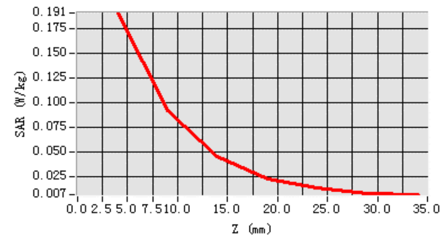
SAR, Z Axis Scan (X = -9, Y = 1)
