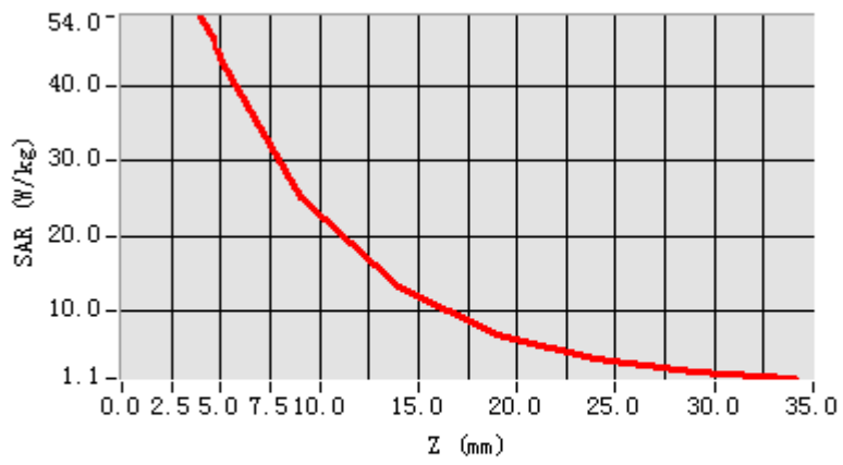
SAR, Z Axis Scan (X = 1, Y = -2)
