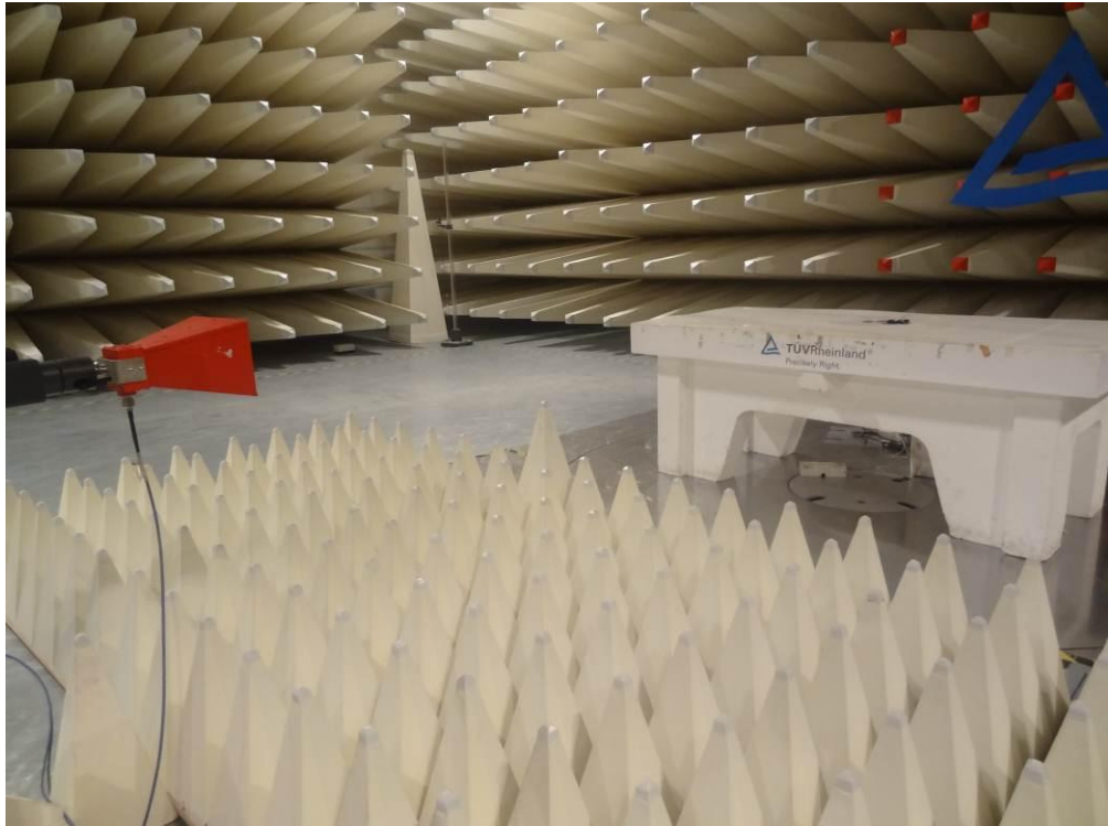
Test setup
