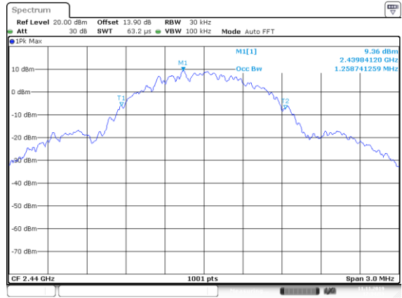
BLE-1Mbps Middle CH
