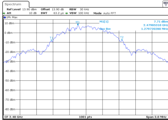
BLE-1Mbps High CH
