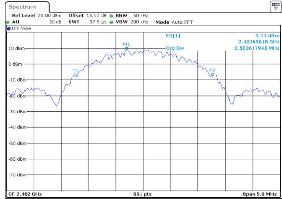
BLE-2Mbps Low CH
