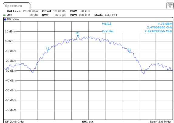
BLE-2Mbps High CH
