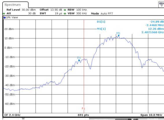
BLE-2Mbps Left Side
