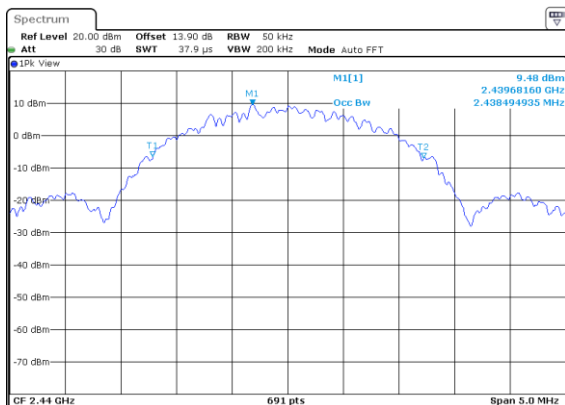
BLE-2Mbps Middle CH
