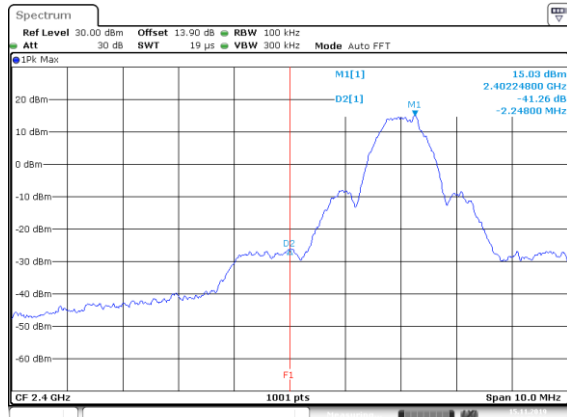
BLE-1Mbps Left Side
