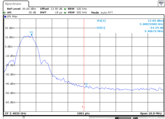
BLE-1Mbps Right Side
