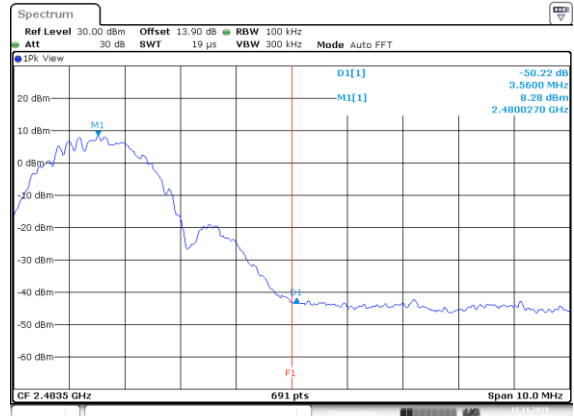
BLE-2Mbps Right Side
