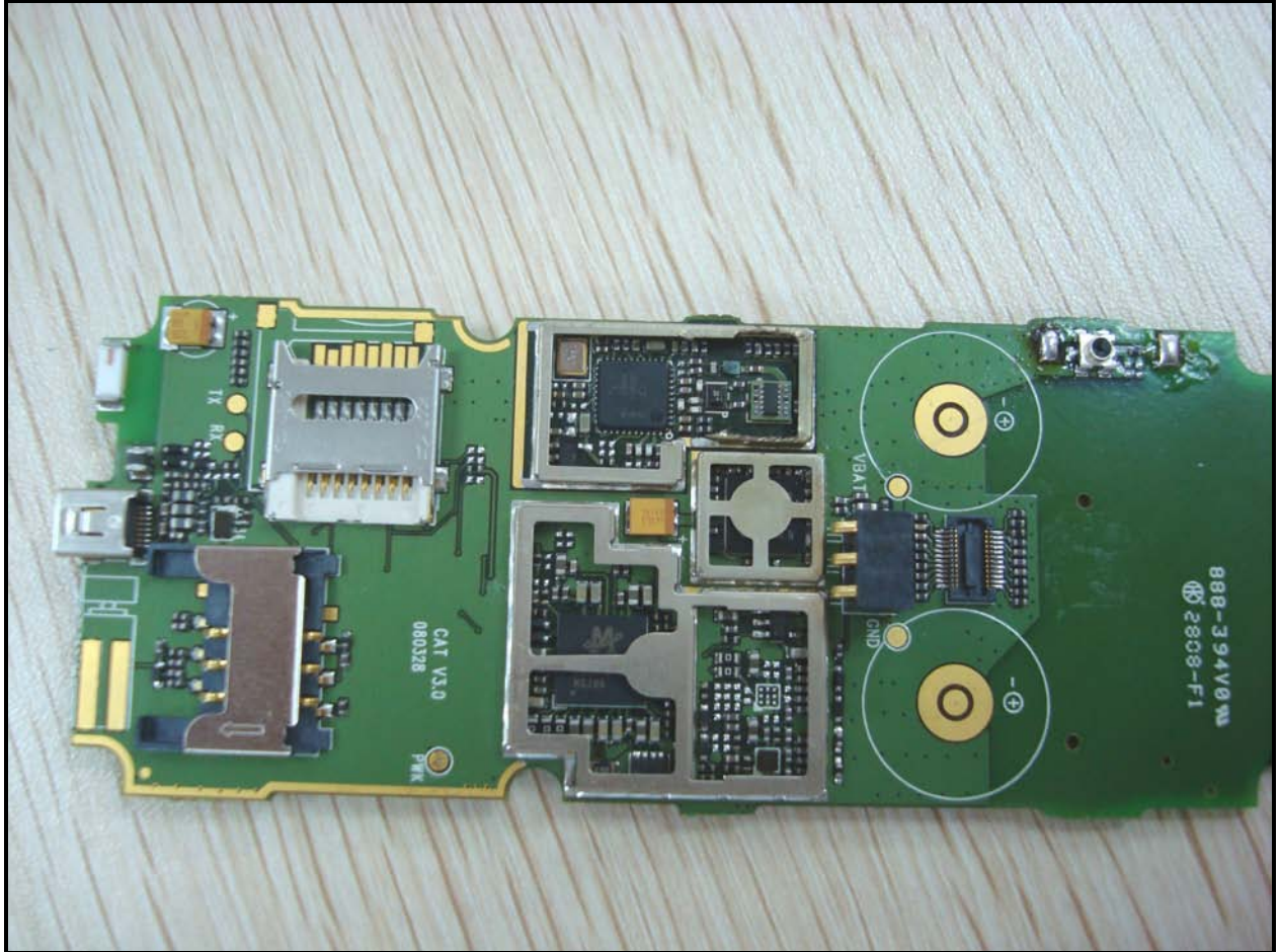
Photograph 11: PCB Back
