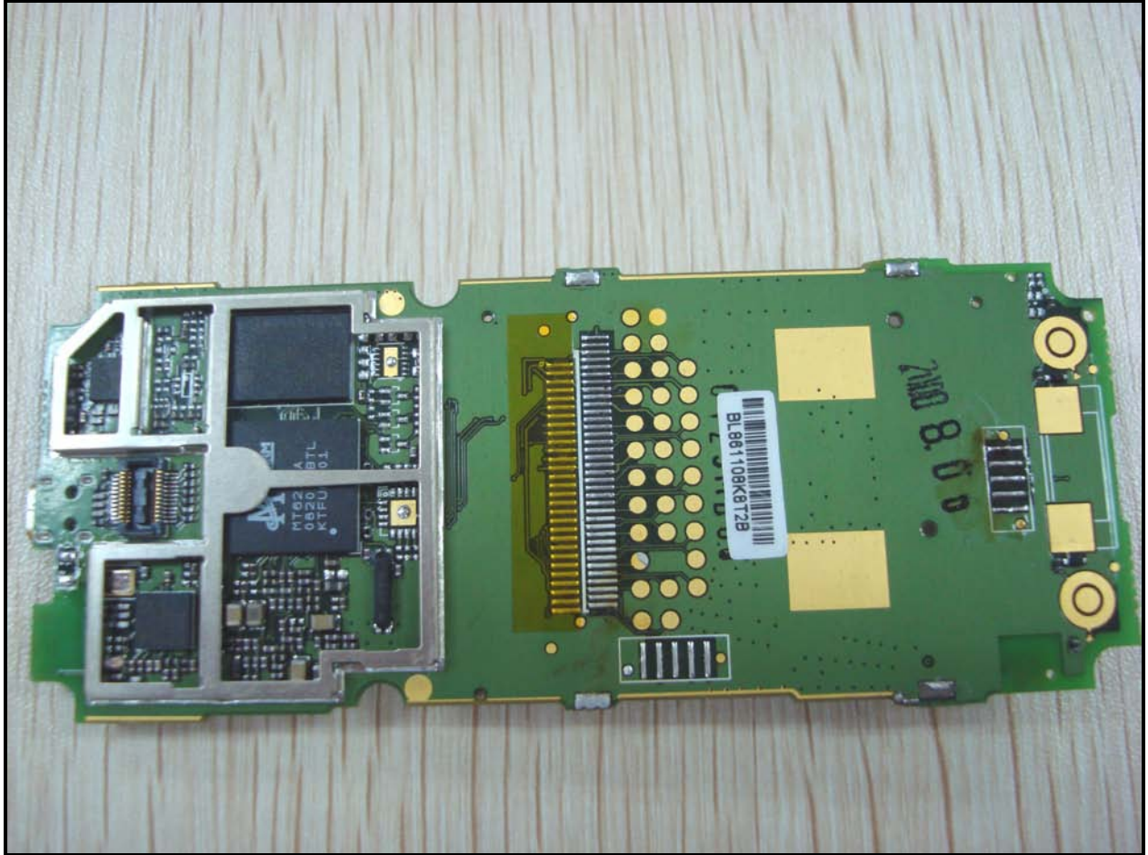
Photograph 10: PCB Front
