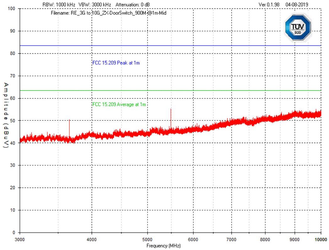
Graph 24 Test Results – Tx Spurious emission 3GHz – 10GHz – Mid Channel – Vertical polarisation
