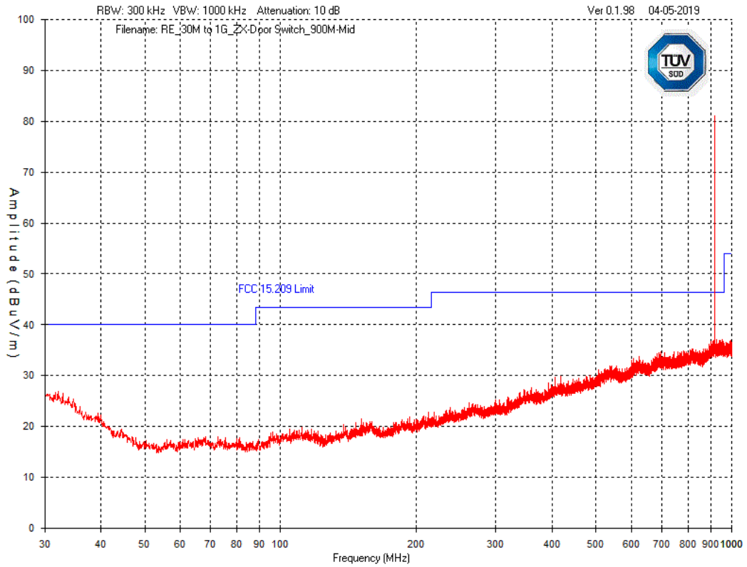
Graph 19 Test Results – Tx Spurious Emission 30MHz to 1GHz – Mid Channel – Vertical Polarization
