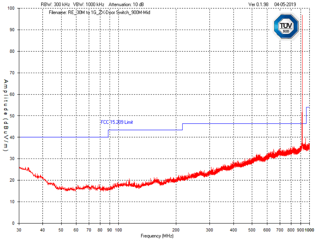
Graph 20 Test Results – Tx Spurious emission 30MHz to 1GHz – Mid Channel – Horizontal Polarization
