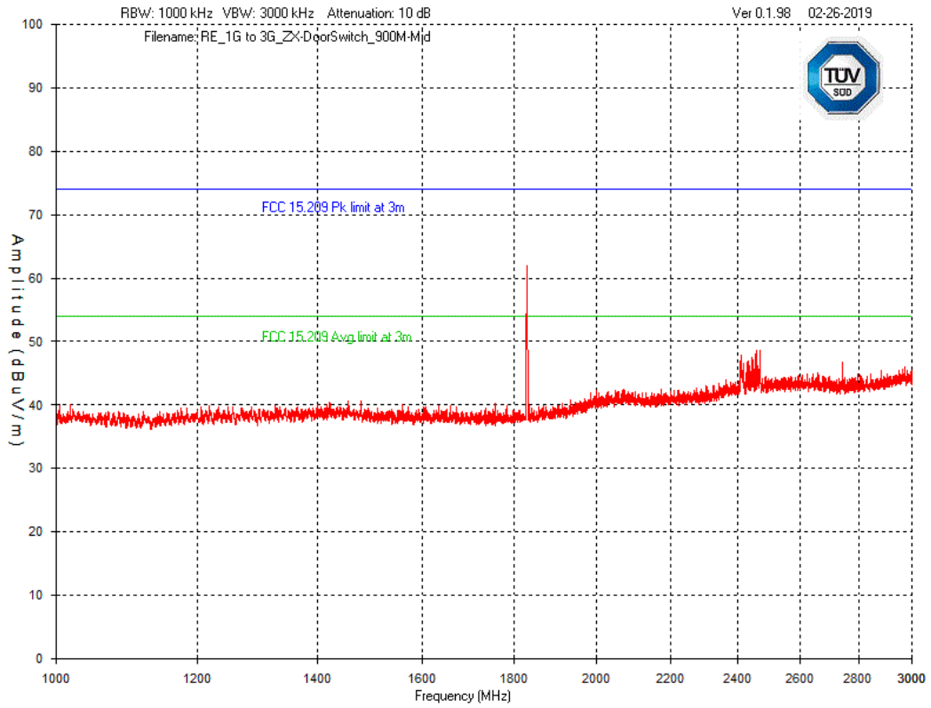
Graph 22 Test Results – Tx Spurious emission 1GHz – 3GHz – Mid Channel – Horizontal Polarization
