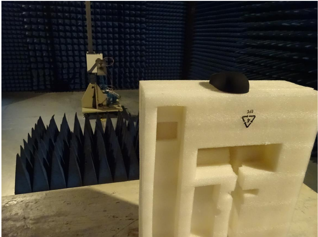
Setup Photo above 1GHz:
