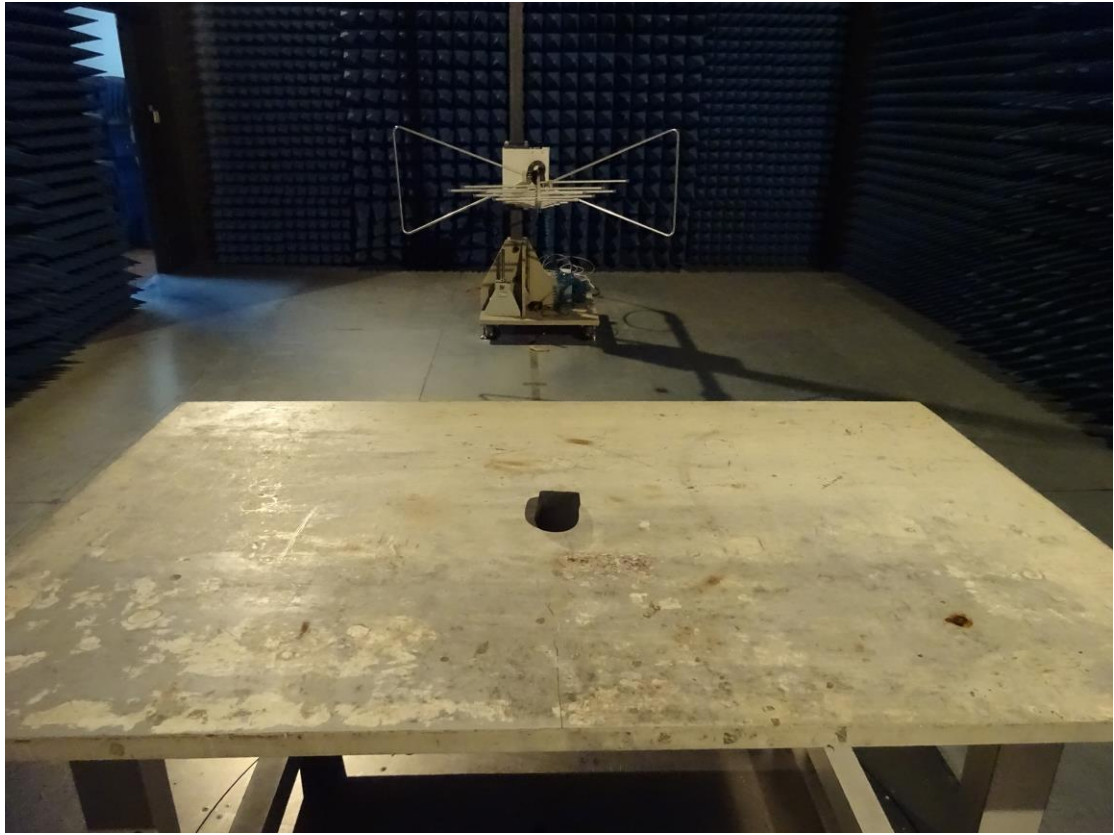
Setup Photo below 1GHz:
