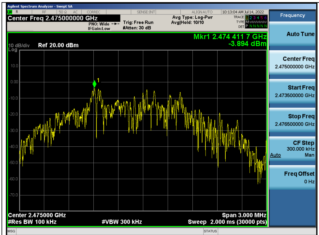
Test_Graph_2.4G_ANT1_2475_Reference Level
