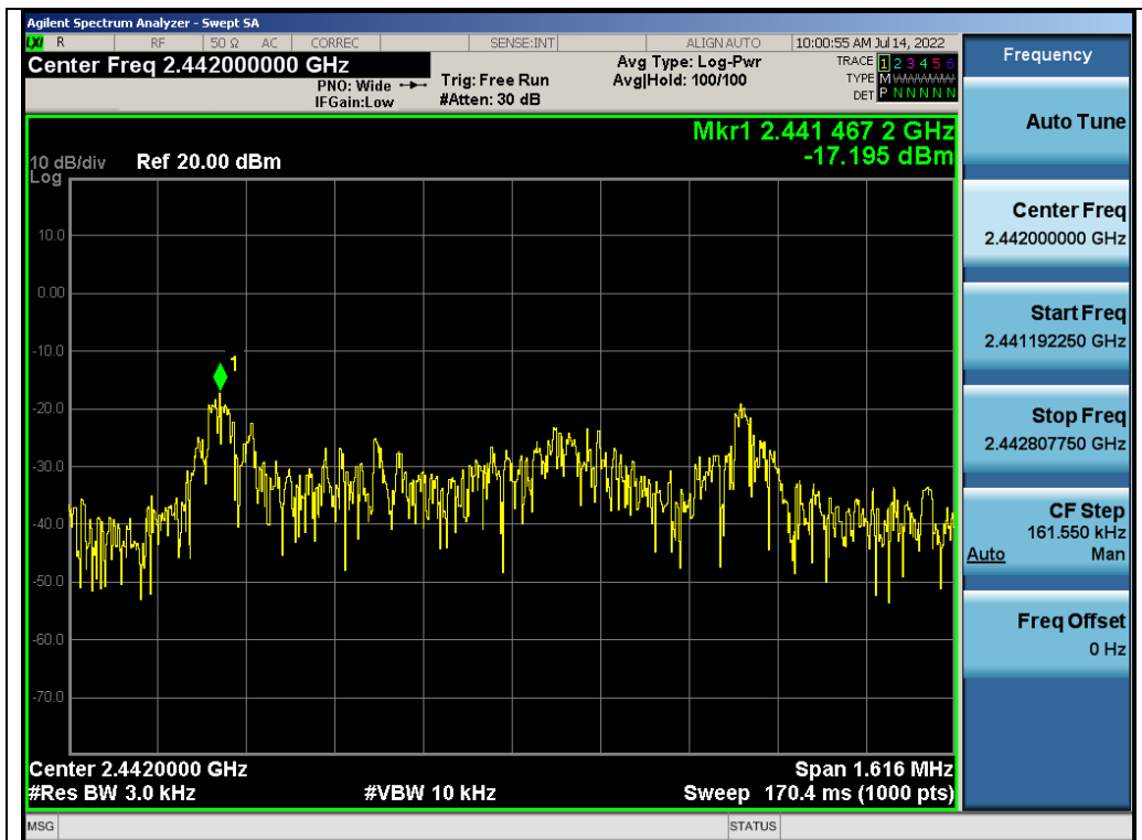
Test_Graph_2.4G_ANT1_2442_PSD
