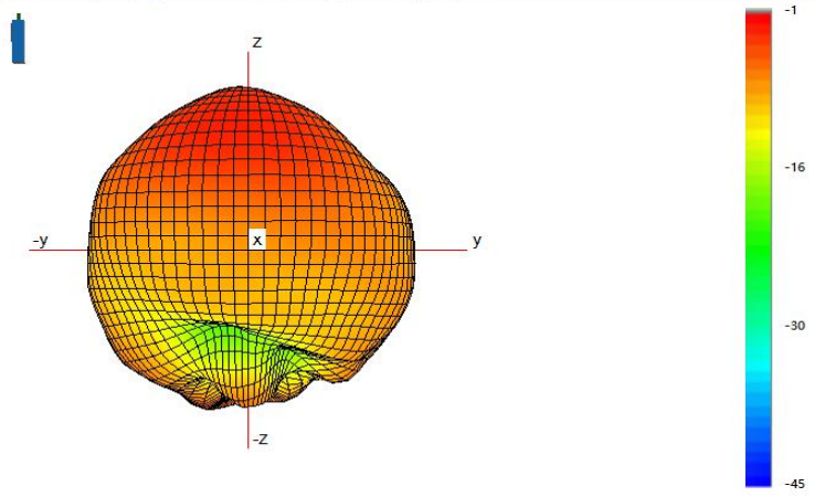
FREQUENCY=2450MHZ
