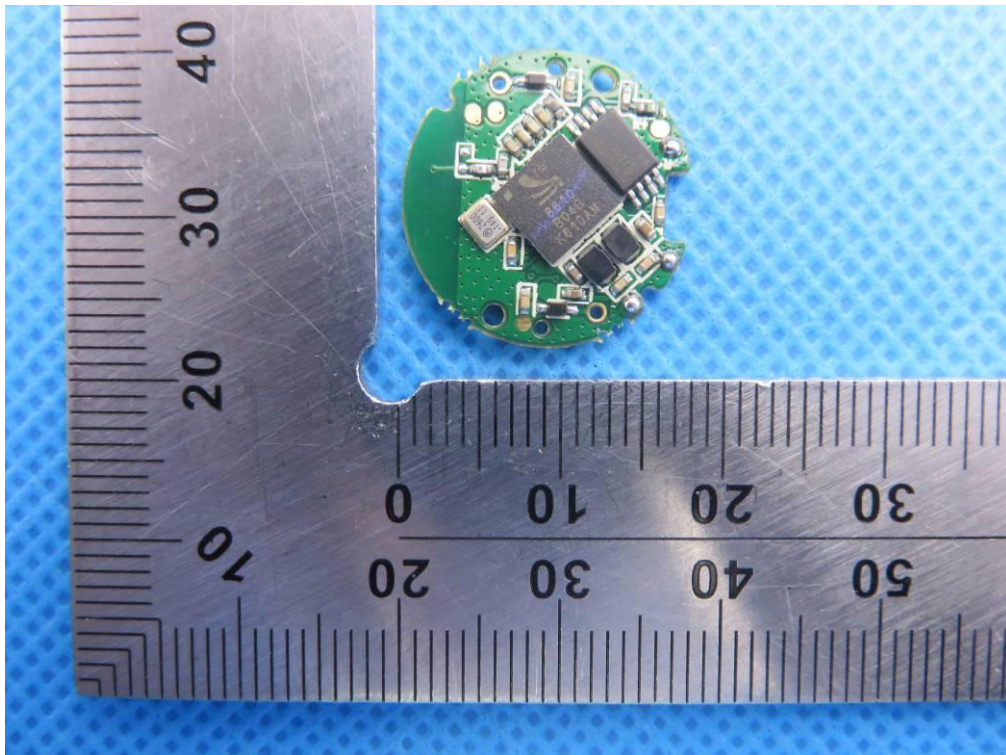
INTERNAL VIEW OF EUT-1 (BC02)
