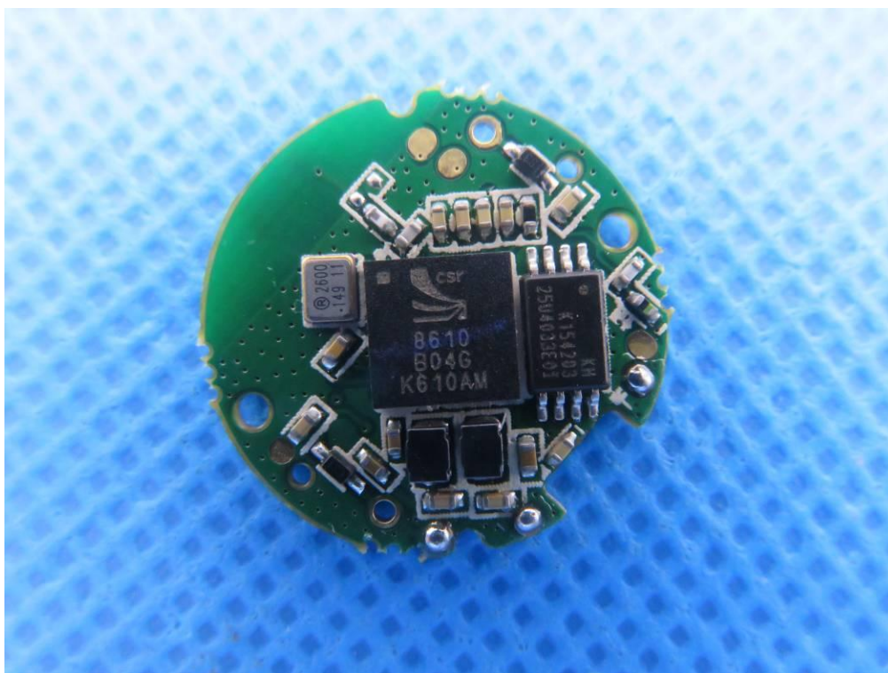
INTERNAL VIEW OF EUT-3 (BC02)
