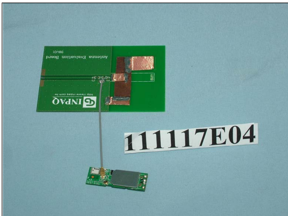
EUT: WFA9271M20 with PIFA antenna
