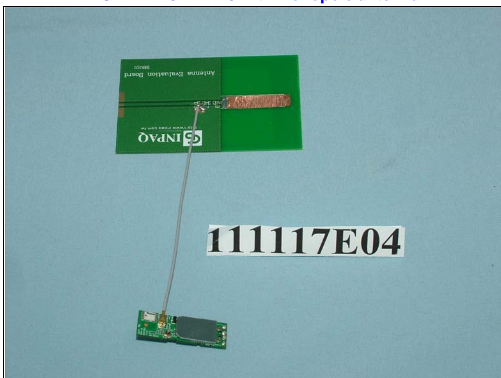
EUT: WFA9271M20 with Monopole antenna
