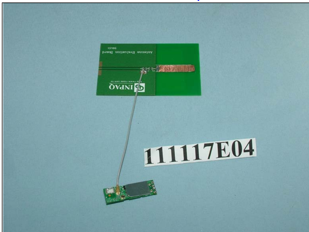
EUT: WFA9271M10 with Monopole antenna
