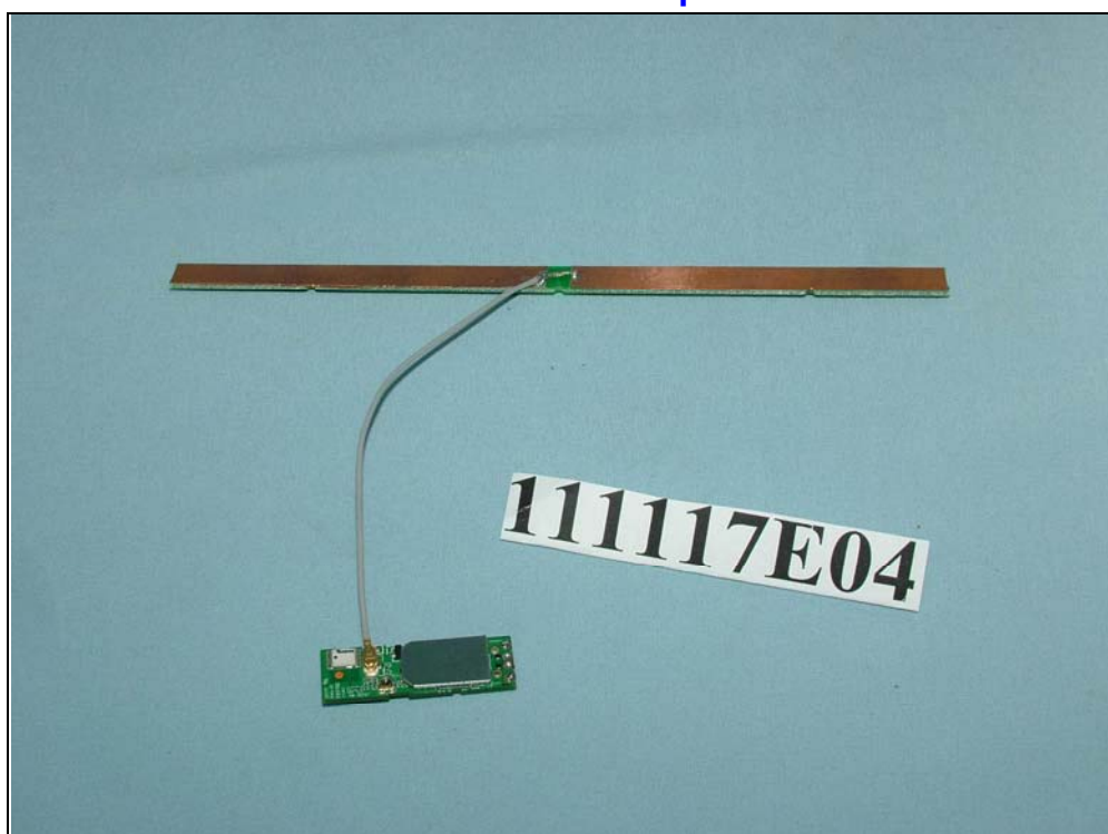
EUT: WFA9271M10 with Dipole antenna
