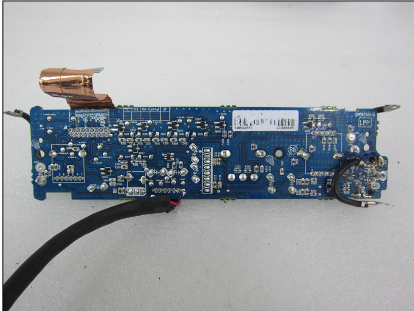
Panel B/D
