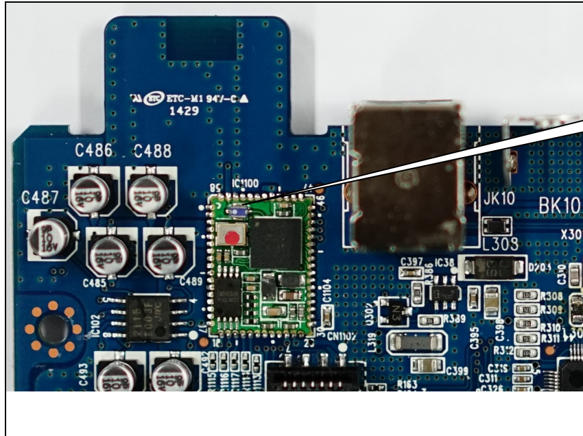
Chip Antenna
