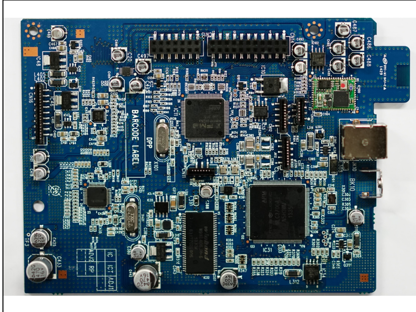
Main B/D
