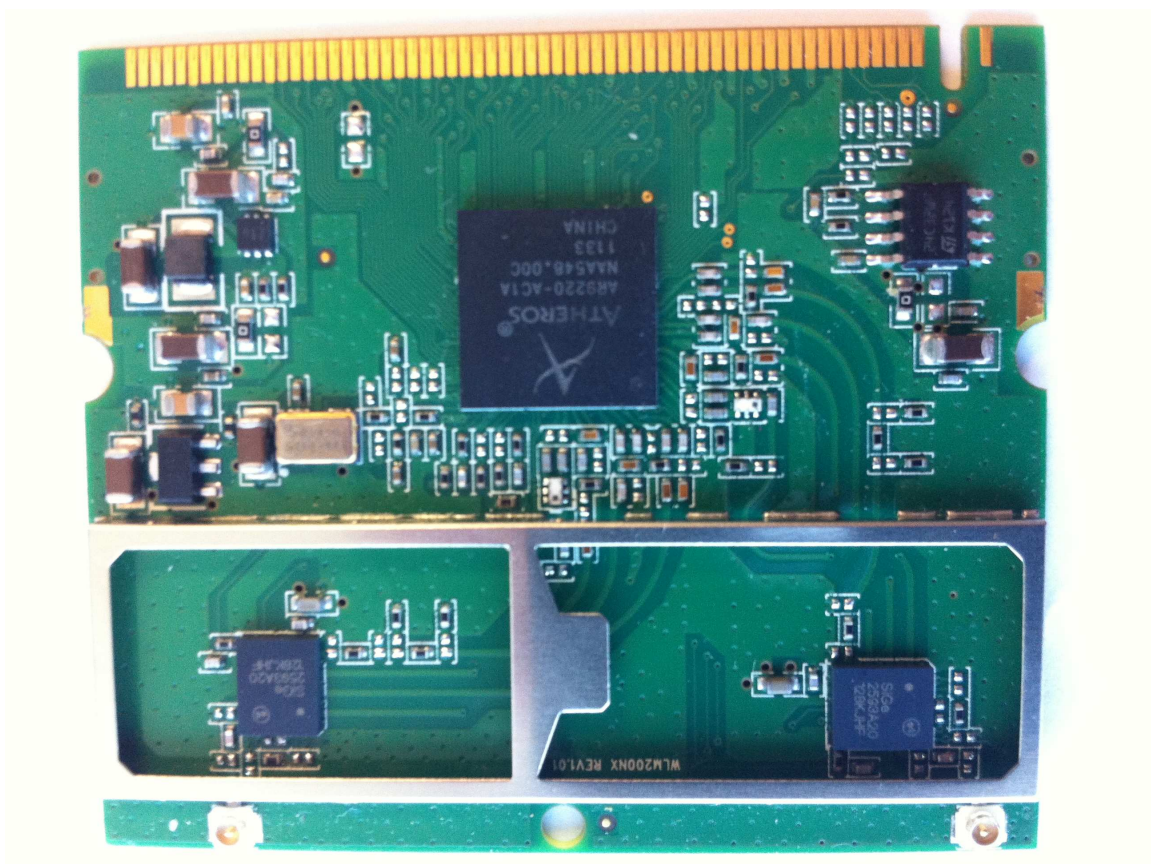
Front of module with RF shields removed
