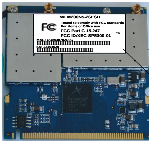
Radio Module and Label Location
