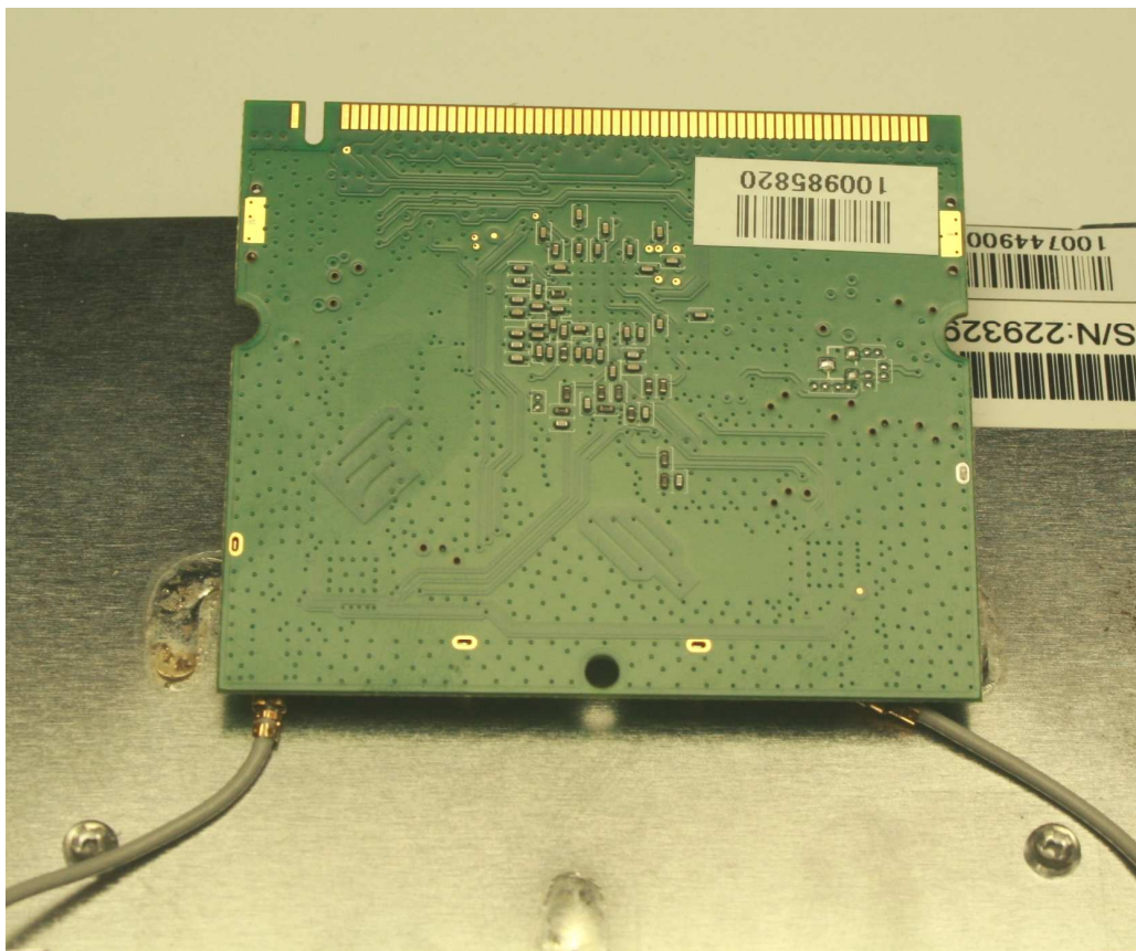
Top and Bottom views of the Radio Module FCC TK4-09-WLM200NX
