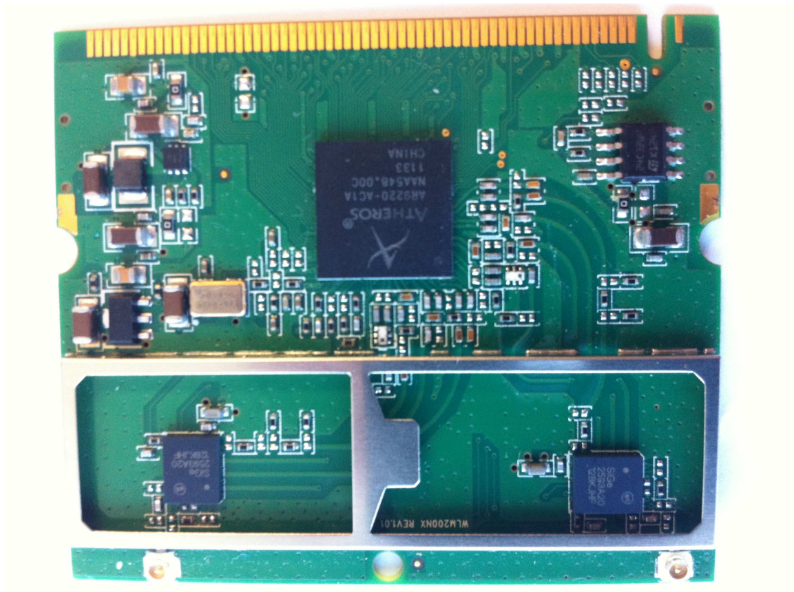
Top View of the Radio Module FCC TK4-09-WLM200NX with RF shield removed.
