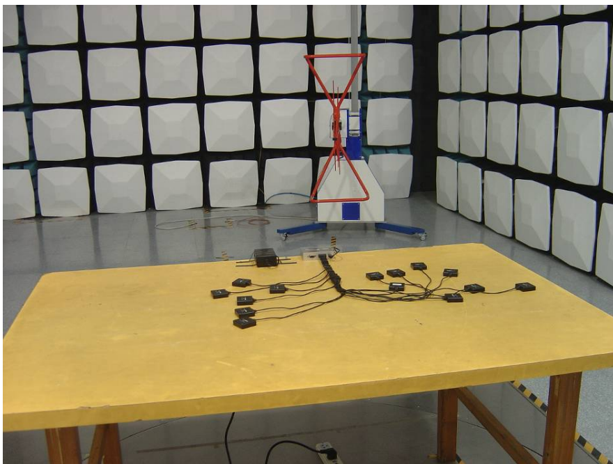
Radiated Emissions - Rear View (Charging Mode)
