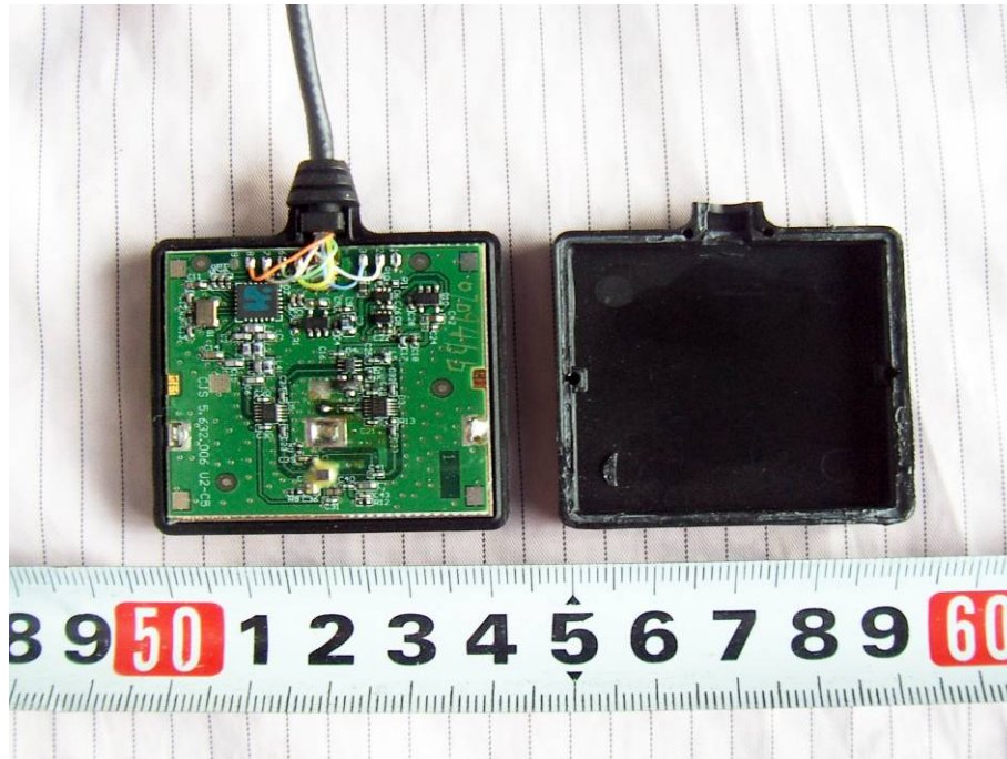
EUT – Antenna Module Cover off View
