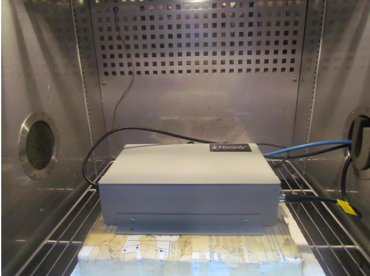
FCC RF Conducted Setup
