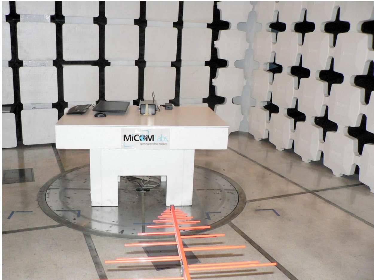
THNK15 Digital Emissions 30-1000MHz
