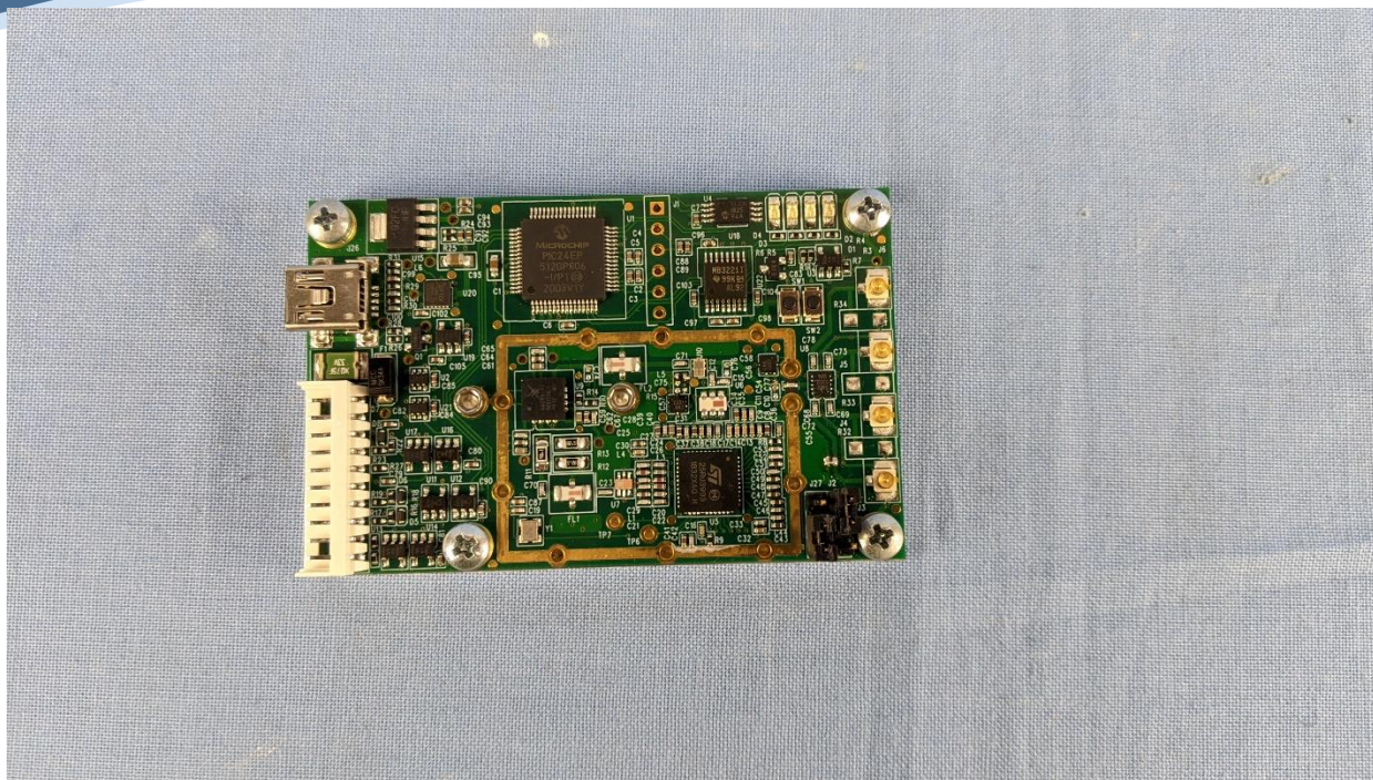
Top View Shield Removed
