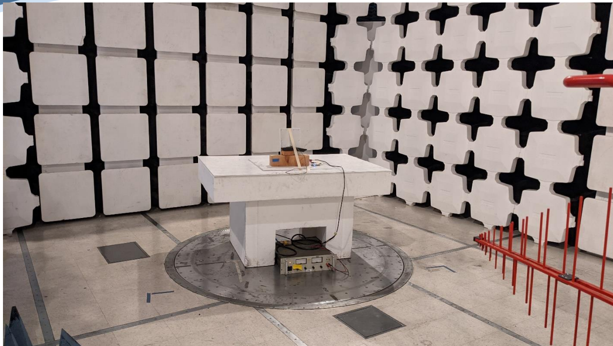
Digital Emissions 30MHz to 1GHz
