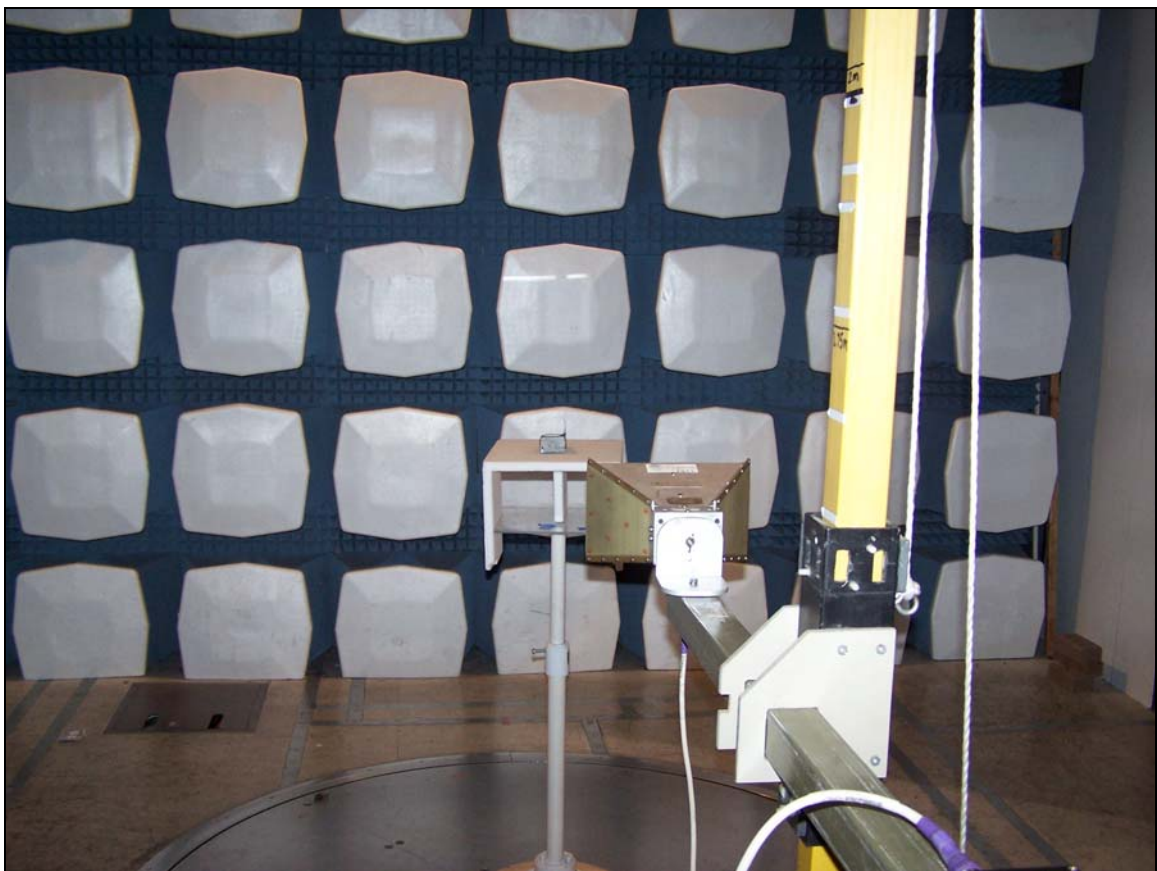
Photograph 2. Spurious Emissions Test Setup
