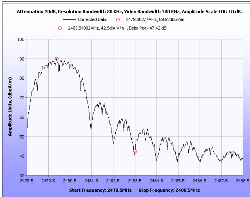
Plot 17. Band Edge, Upper Channel for Delta Marker Method
