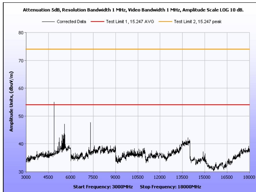
Plot 9. Radiated Harmonic Emissions, Mid Channel
