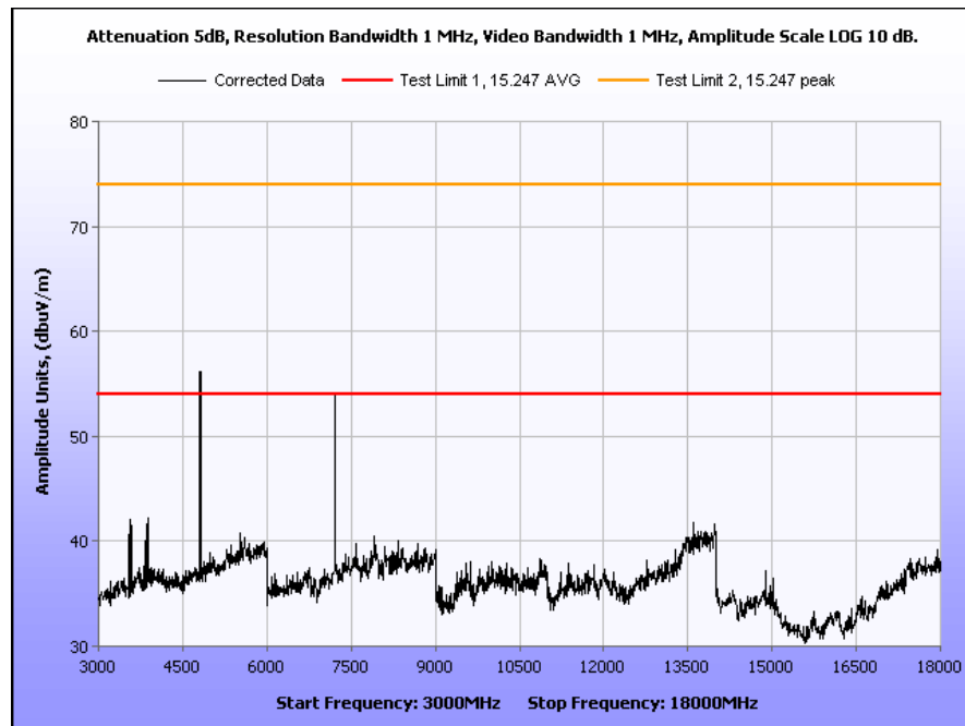
Plot 8. Radiated Harmonic Emissions, Low Channel
