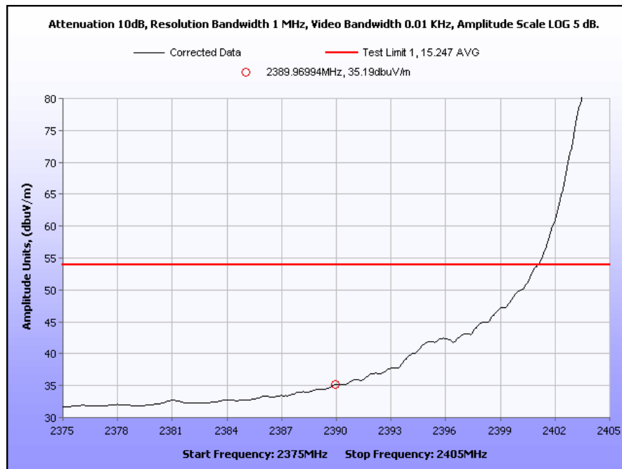
Plot 14. Lower Band Edge, Average
