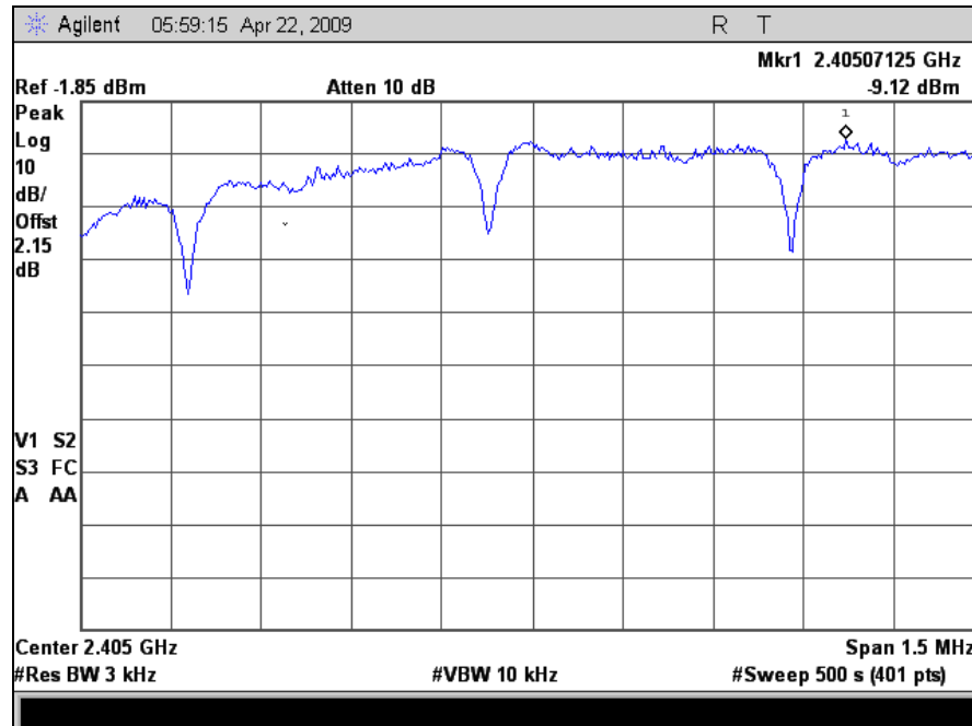
Plot 21. Peak Power Spectral Density, Low Channel
