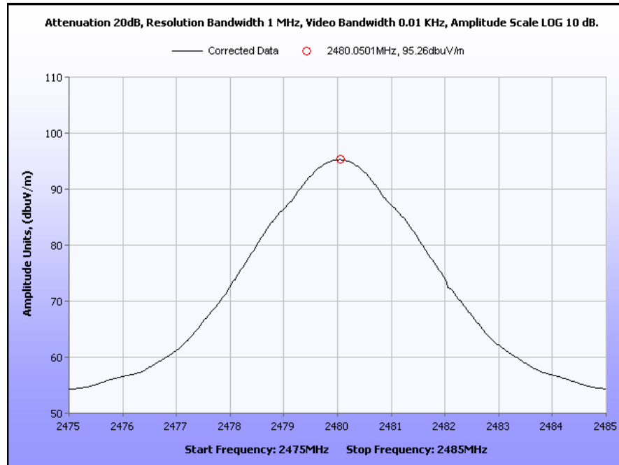
Plot 16. Peak Value of Fundamental, Upper Band Edge
