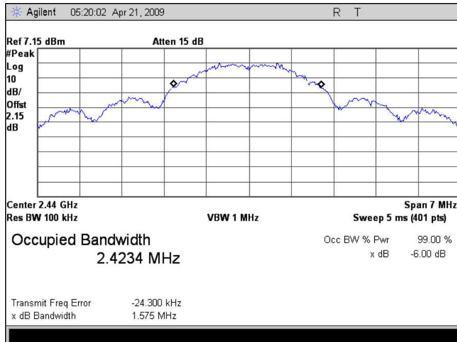
Plot 3. Occupied Band Width, Mid Channel, 6 dB
