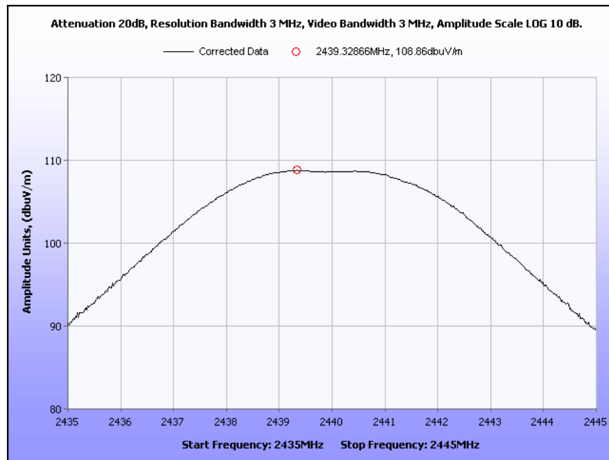
Plot 6. Peak Output Power, Mid Channel
