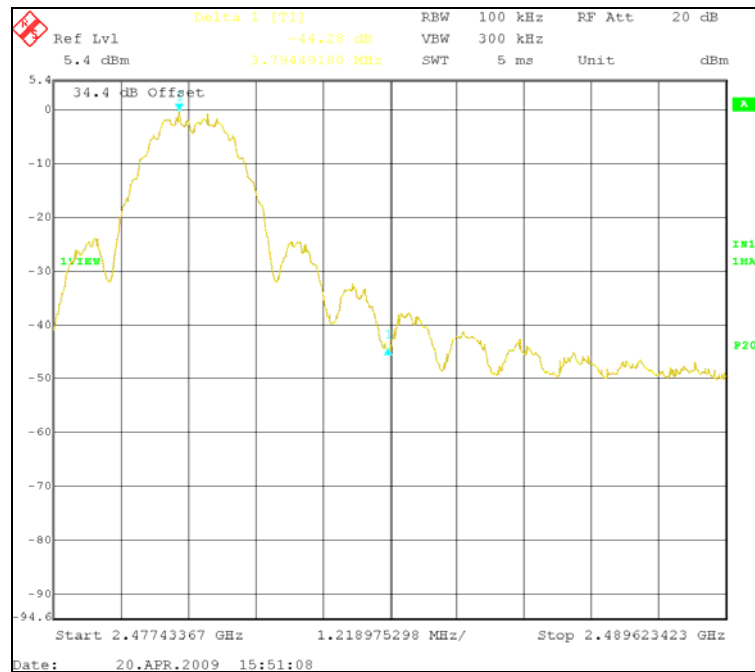
Plot 12. Conducted Spurious Emissions, Upper Band, 30 dBc
