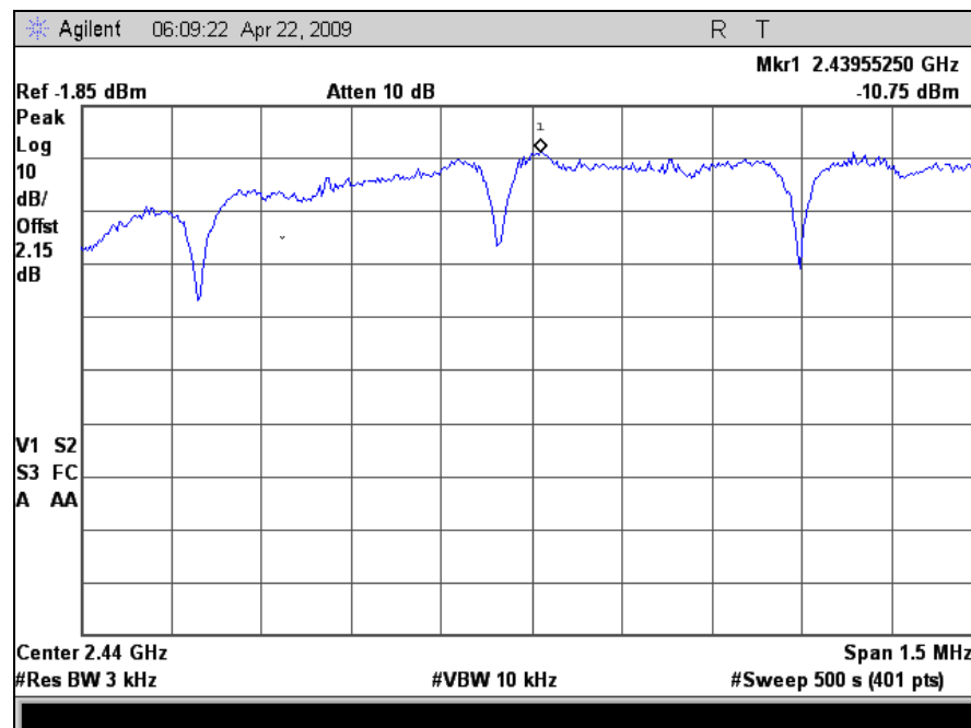
Plot 22. Peak Power Spectral Density, Mid Channel
