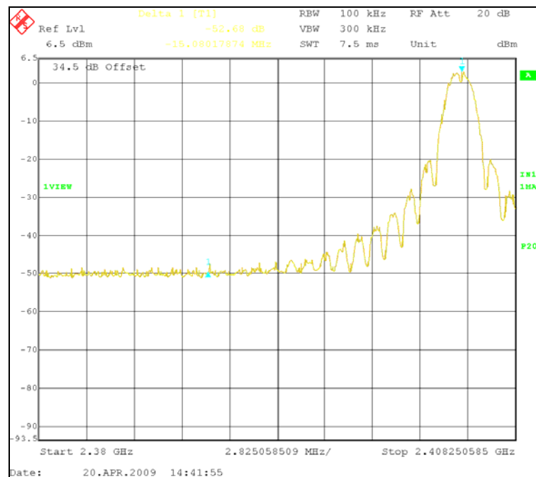
Plot 11. Conducted Spurious Emissions, Lower Band, 30 dBc
