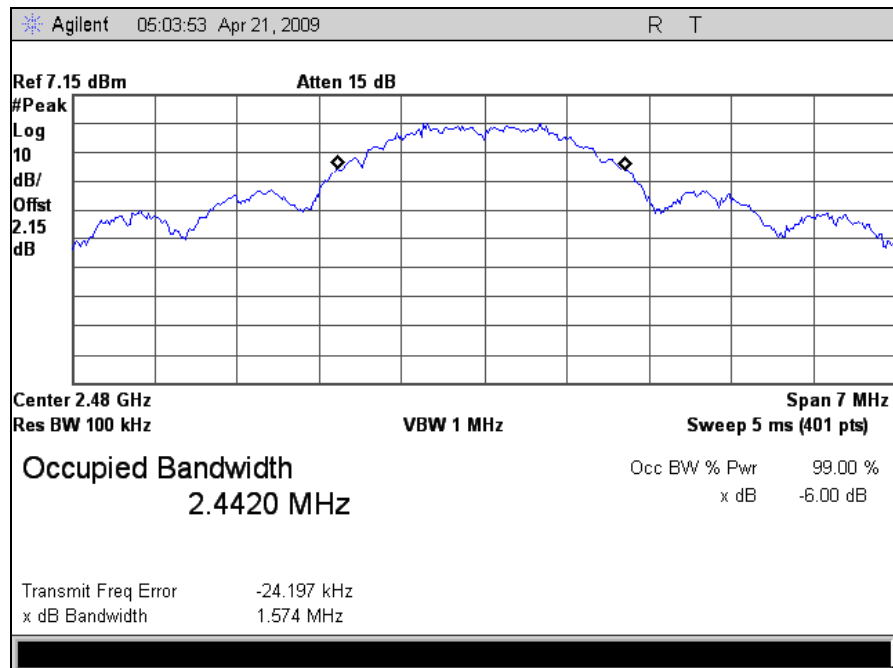
Plot 4. Occupied Band Width, High Channel, 6 dB
