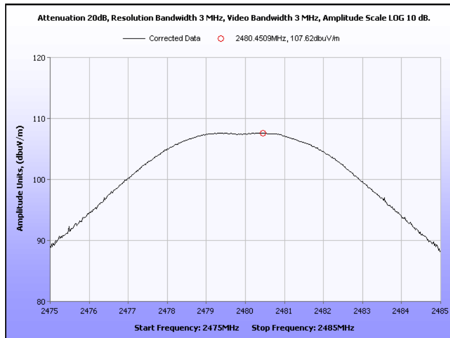
Plot 7. Peak Output Power, High Channel
