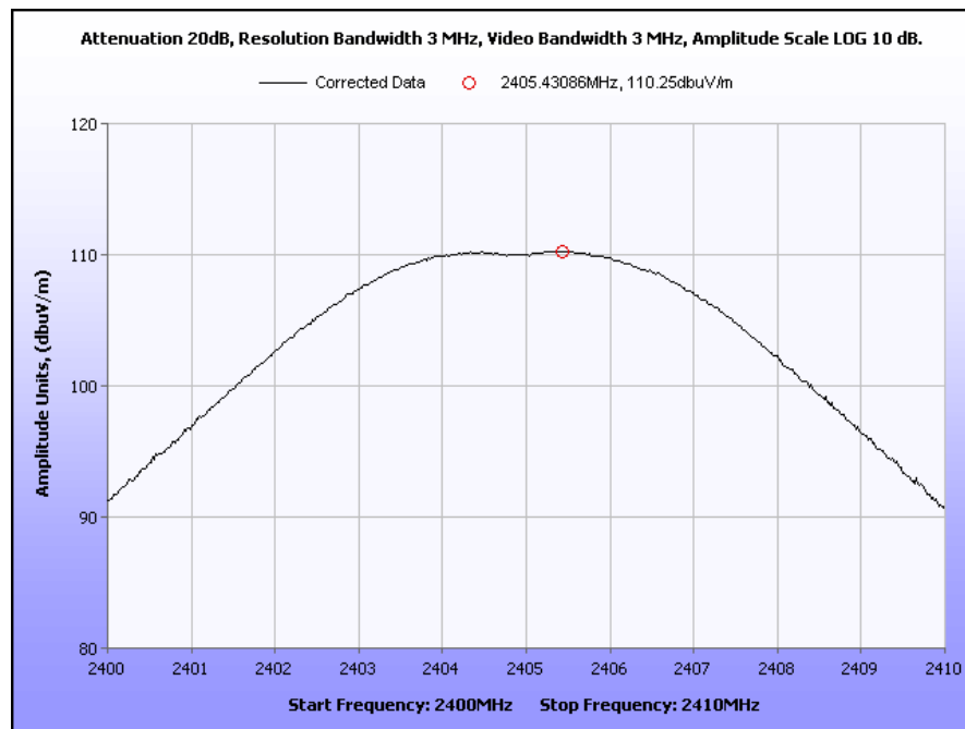
Plot 5. Peak Output Power, Low Channel
