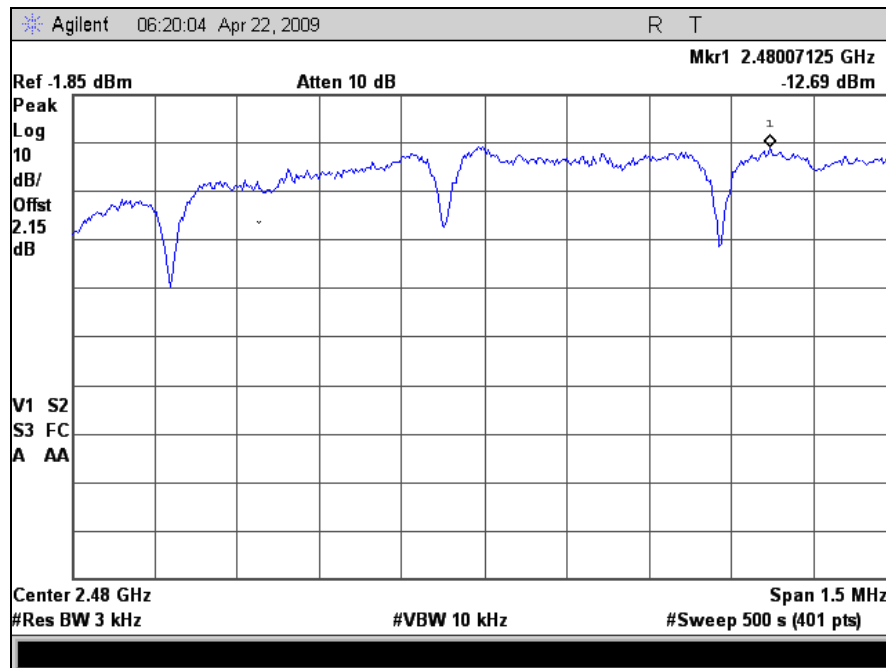
Plot 23. Peak Power Spectral Density, High Channel
