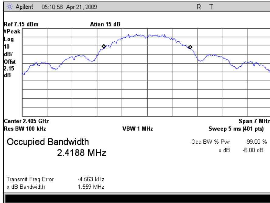
Plot 2. Occupied Band Width, Low Channel, 6 dB
