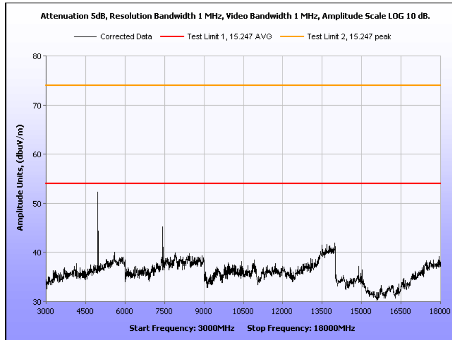
Plot 10. Radiated Harmonic Emissions, High Channel
