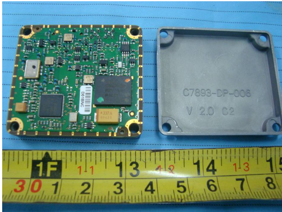
EUT – Iridium Module Main Board Top View
