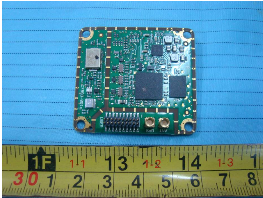
EUT – Iridium Antenna View
