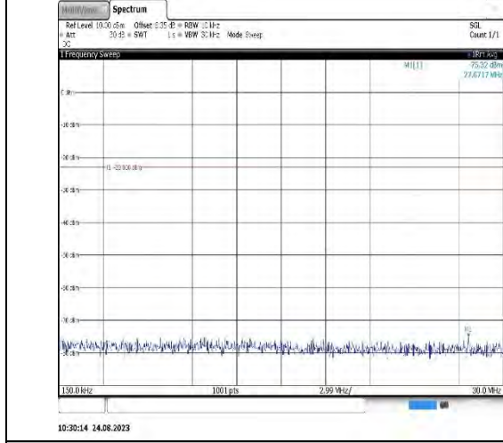
10:30:14 24.08.2023 Band26_10MHz_16QAM_26915_1RB#0_1000~300_0_1000~3000
