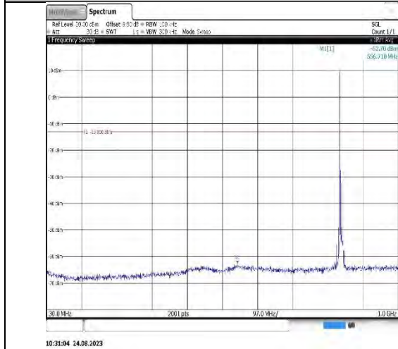
Band26_10MHz_QPSK_26990_1RB#0_3000~1000_3000~10000 0_3000~10000
