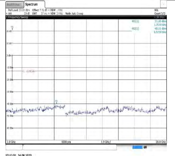
Band66-5MHz-16QAM-132647-1RB#0-Range2:1000~20000MHz
