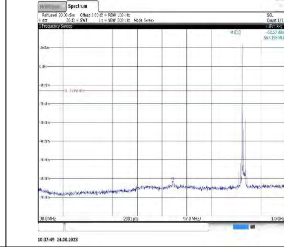
Band26_15MHz_16QAM_26915_1RB#0_3000~1000_0_3000~10000
