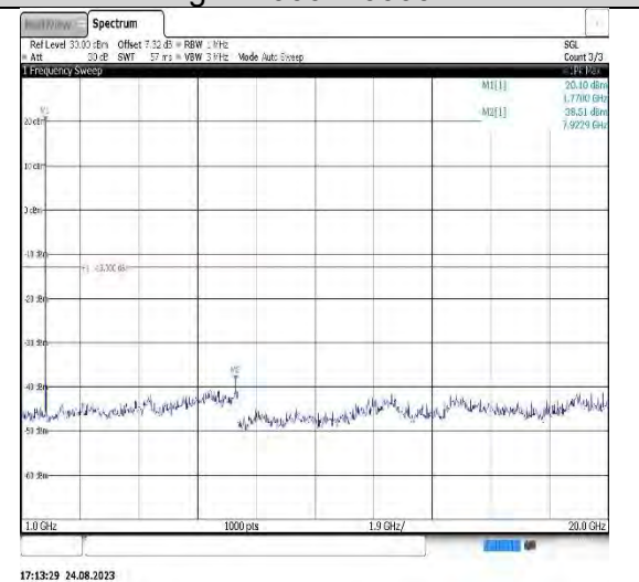
Band66-5MHz-16QAM-132647-1RB#0-Range2:1000~20000MHz
