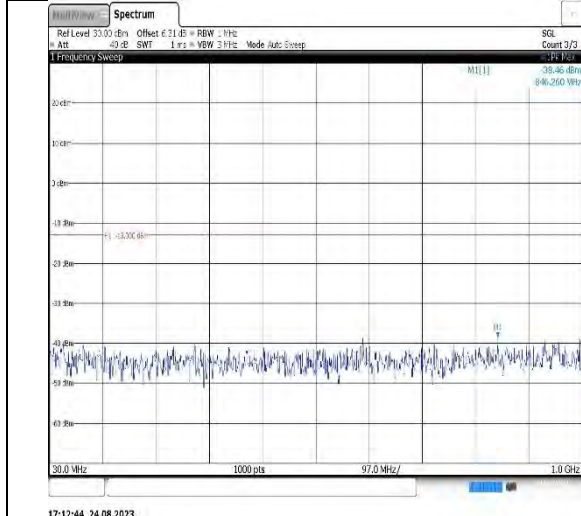
Band66-5MHz-16QAM-132647-1RB#0-Range1:30~1000MHz
