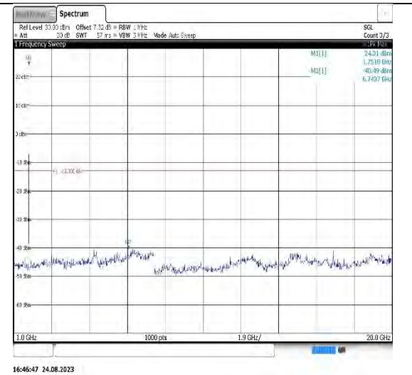
Band66-3MHz-16QAM-132657-1RB#0-Range2:1000~20000MHz
