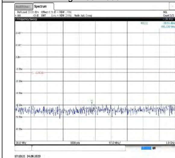
Band66-5MHz-16QAM-132647-1RB#0-Range1:30~1000MHz
