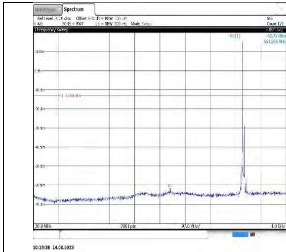
10:29:38 24.08.2023 Band26_10MHz_QPSK_26915_1RB#0_3000~1000_0_3000~10000
