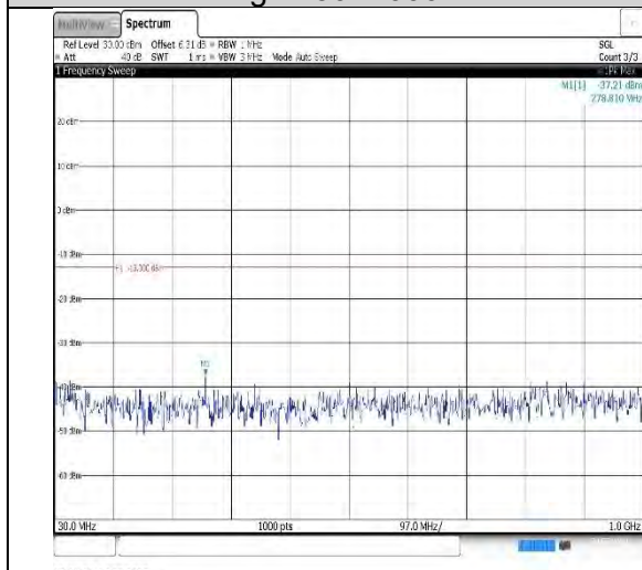
Band66-5MHz-QPSK-131997-1RB#0-Range1:30~1000MHz
