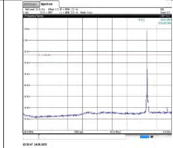
Band26_10MHz_16QAM_26990_1RB#0_3000~1000_0_3000~10000
