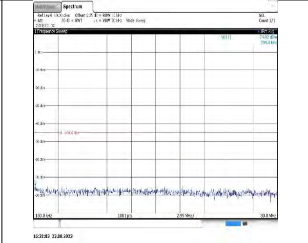
Band41_15MHz_QPSK_41515_1RB#0_1000~20000_1000~20000
