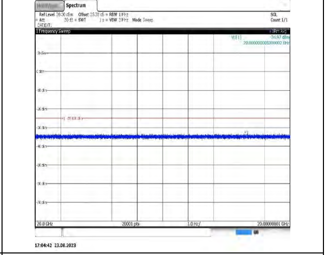
Band66-1.4MHz-QPSK-131979-1RB#0-Range2:1000~20000MHz
