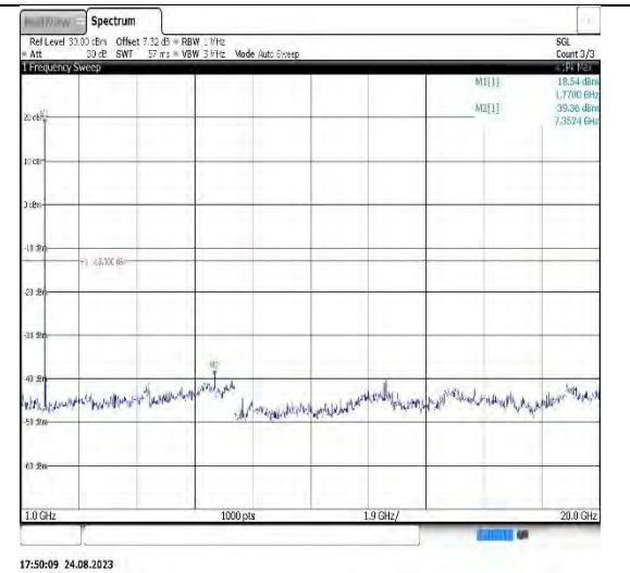
Band66-10MHz-16QAM-132022-1RB#0-Range2:1000~20000MHz
