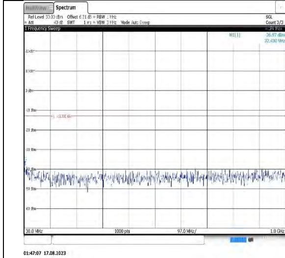
Band25-15MHz-16QAM-26615-1RB#0-Range1:30~1000MHz
