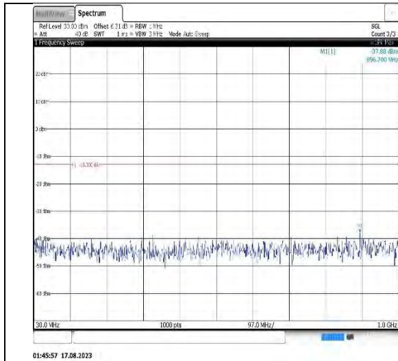
Band25-15MHz-16QAM-26365-1RB#0-Range1:30~1000MHz
