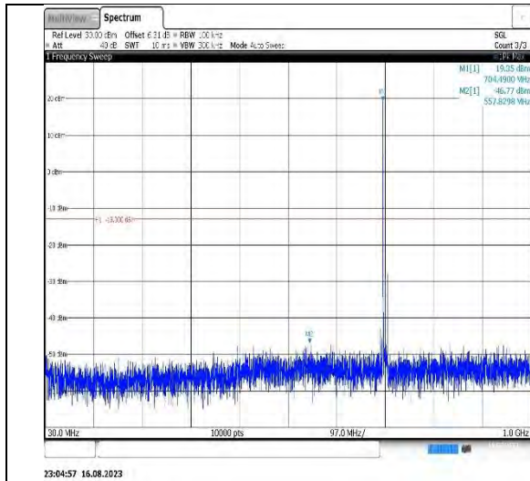
Band 17-10MHz-16QAM-23790-1RB#0-Range1:30~1000MHz
