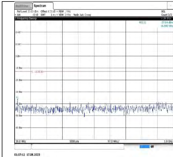
Band25-20MHz-16QAM-26140-1RB#0-Range1:30~1000MHz
