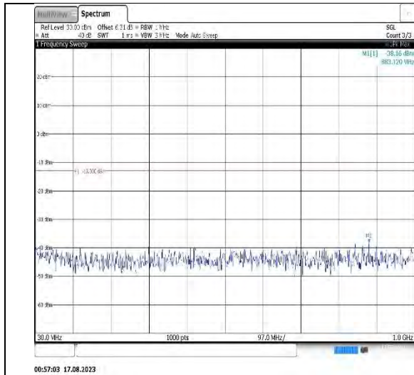
Band25-5MHz-QPSK-26365-1RB#0-Range1:30~1000MHz
