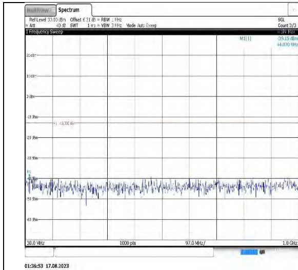
Band25-10MHz-16QAM-26640-1RB#0-Range1:30~1000MHz
