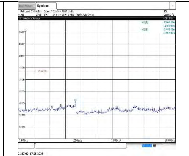
Band25-10MHz-16QAM-26640-1RB#0-Range2:1000~20000MHz
