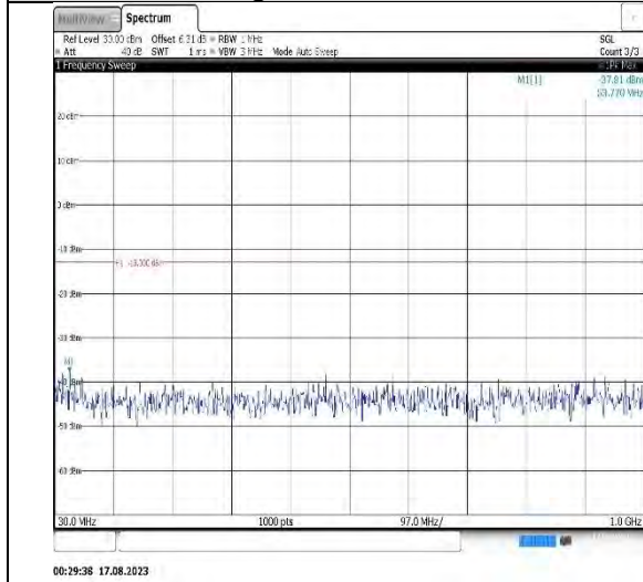
Band25-3MHz-16QAM-26055-1RB#0-Range1:30~1000MHz
