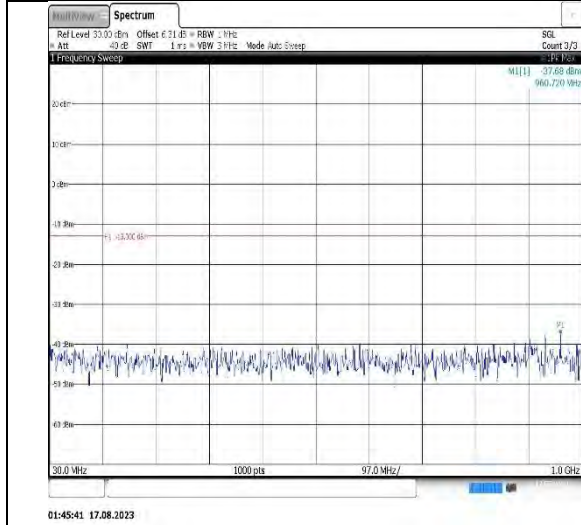
Band25-15MHz-QPSK-26115-1RB#0-Range1:30~1000MHz
