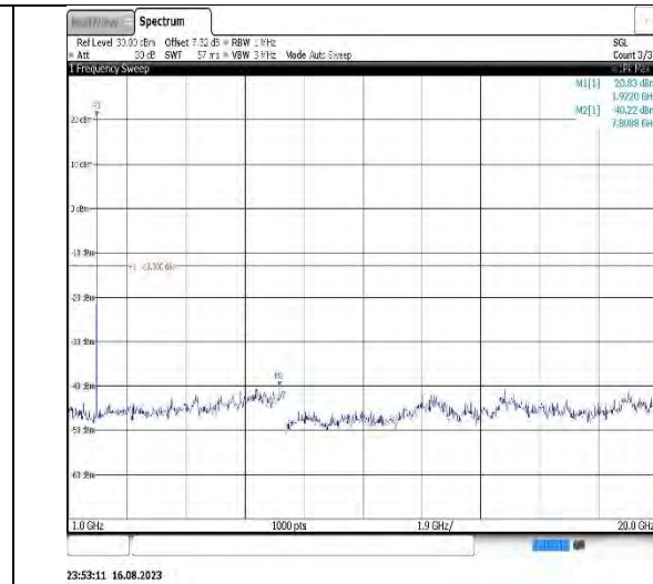
Band25-1.4MHz-16QAM-26047-1RB#0-Range2:1000~20000MHz
