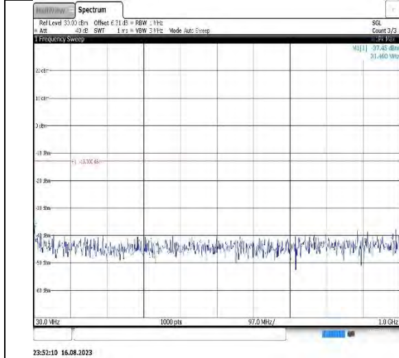
Band25-1.4MHz-16QAM-26365-1RB#0-Range1:30~1000MHz
