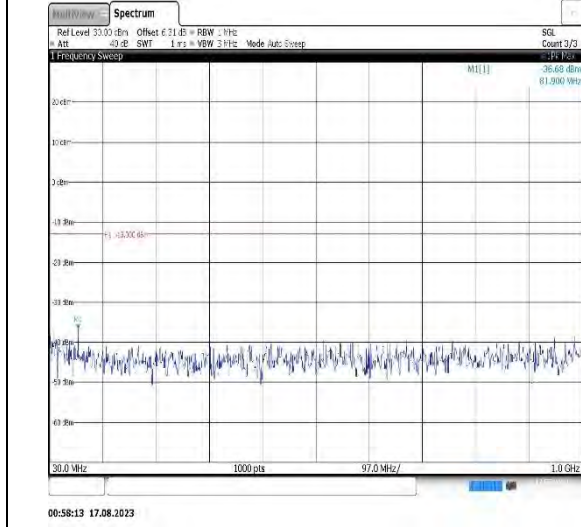
Band25-5MHz-QPSK-26665-1RB#0-Range1:30~1000MHz
