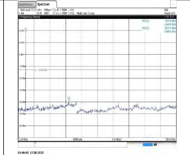
Band25-15MHz-16QAM-26615-1RB#0-Range2:1000~20000MHz
