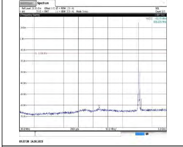
Band26_10MHz_QPSK_26740_1RB#0_3000~1000_3000~10000
