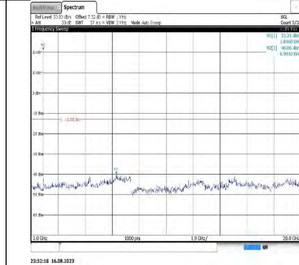
Band25-1.4MHz-16QAM-26365-1RB#0-Range2:1000~20000MHz
