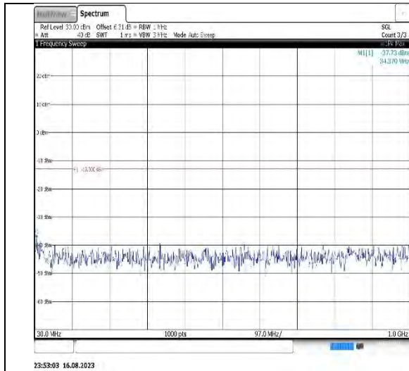
Band25-1.4MHz-16QAM-26047-1RB#0-Range1:30~1000MHz
