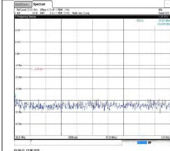
Band25-20MHz-16QAM-26365-1RB#0-Range1:30~1000MHz
