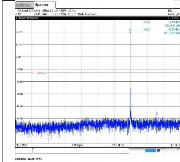
Band 17-10MHz-16QAM-23800-1RB#0-Range1:30~1000MHz
