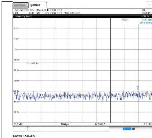
Band25-3MHz-QPSK-26675-1RB#0-Range1:30~1000MHz
