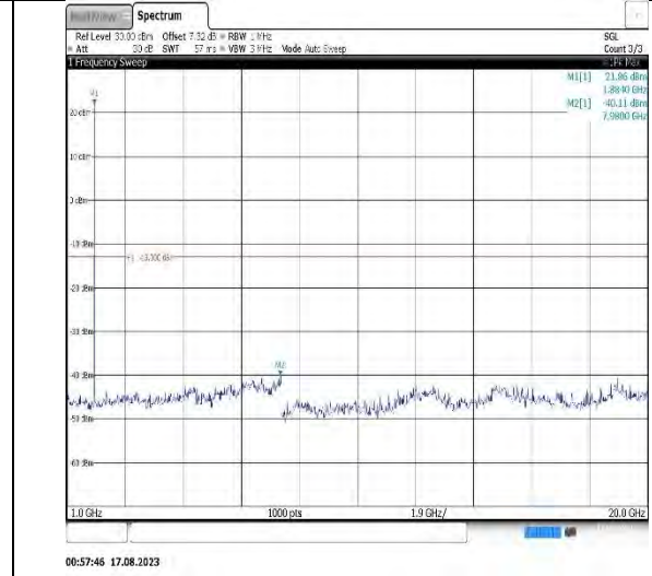
Band25-5MHz-QPSK-26665-1RB#0-Range2:1000~20000MHz
