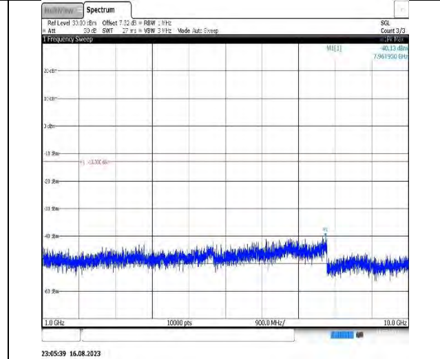
Band 17-10MHz-16QAM-23800-1RB#0-Range2:1000~10000MHz
