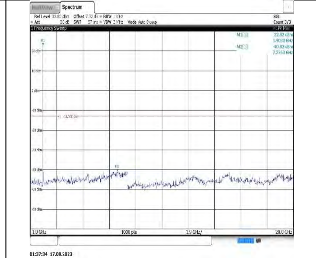
Band25-15MHz-QPSK-26115-1RB#0-Range2:1000~20000MHz
