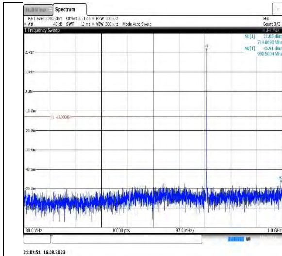
21:02:51 16.08.2023 Band12-1.4MHz-16QAM-23017-1RB#0-Range1:30~1000MHz
