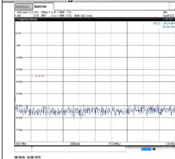
Band7-15MHz-QPSK-21100-1RB#0-Range1:30~1000MHz
