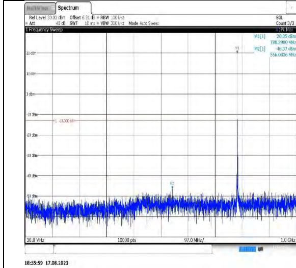
Band 14-5MHz-QPSK-23305-1RB#0- Range1:30~1000MHz
