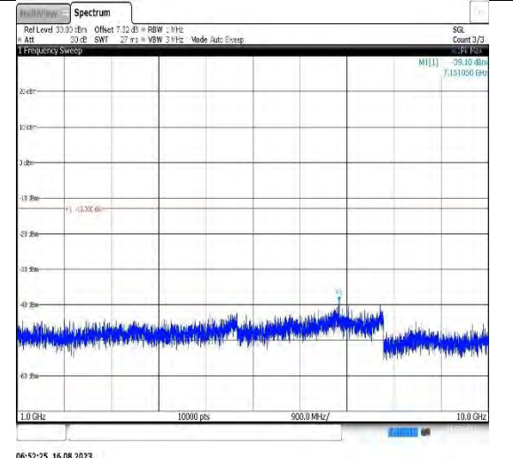
Band5-5MHz-16QAM-20625-1RB#0- Range2:1000~10000MHz
