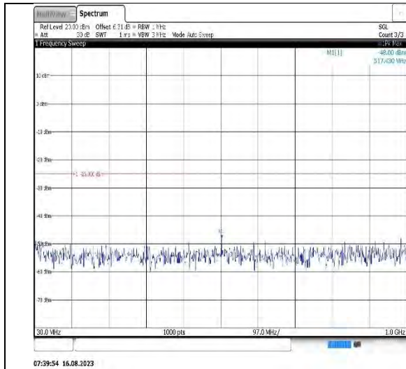
Band7-5MHz-QPSK-21425-1RB#0-Range1:30~1000MHz
