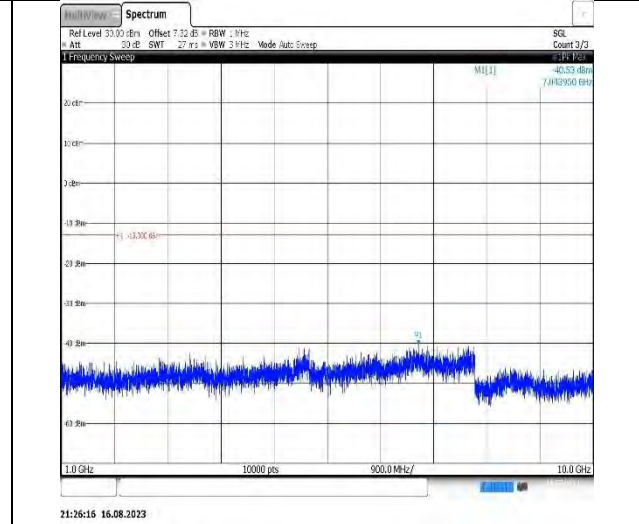
Band12-3MHz-16QAM-23025-1RB#0- Range2:1000~10000MHz
