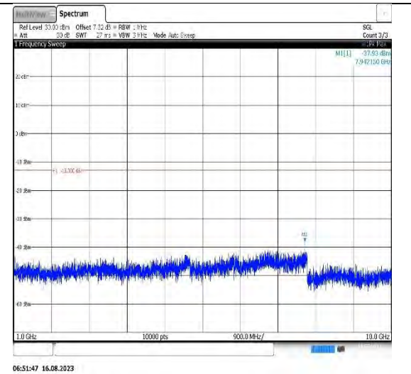
Band5-5MHz-16QAM-20525-1RB#0- Range2:1000~10000MHz
