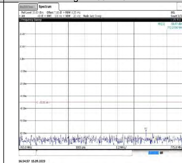
Band13-5MHz-16QAM-23230-1RB#0-Range2:763~775MHz
