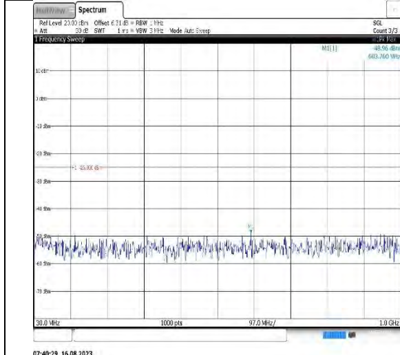
Band7-5MHz-16QAM-20775-1RB#0-Range1:30~1000MHz
