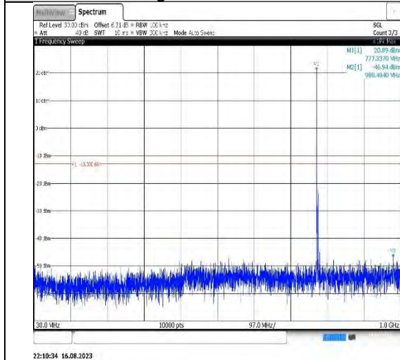
22:10:34 16.08.2023 Band 13-5MHz-QPSK-23205-1RB#0-Range1:30~1000MHz
