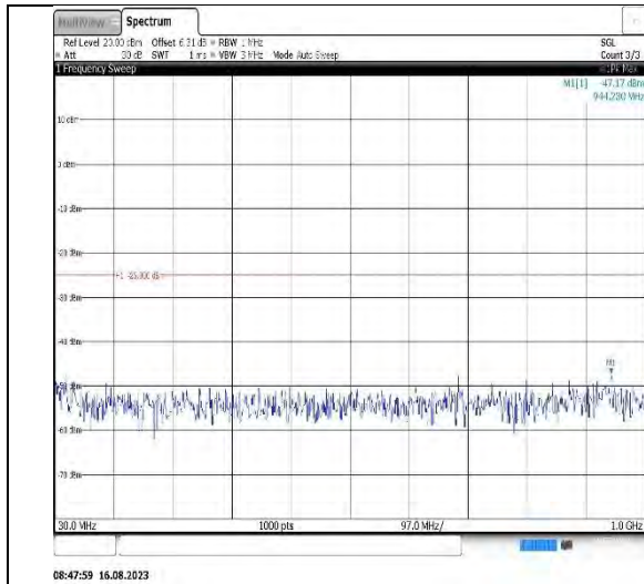
Band7-20MHz-16QAM-21100-1RB#0-Range1:30~1000MHz
