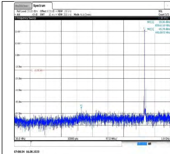
Band5-10MHz-16QAM-20450-1RB#0- Range1:30~1000MHz
