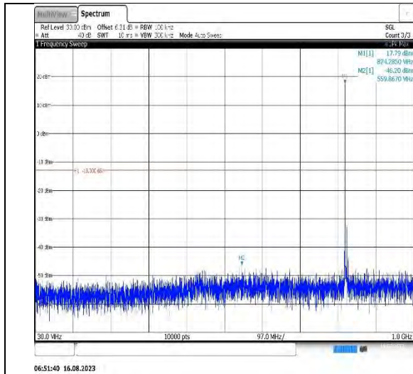
Band5-5MHz-16QAM-20525-1RB#0- Range1:30~1000MHz
