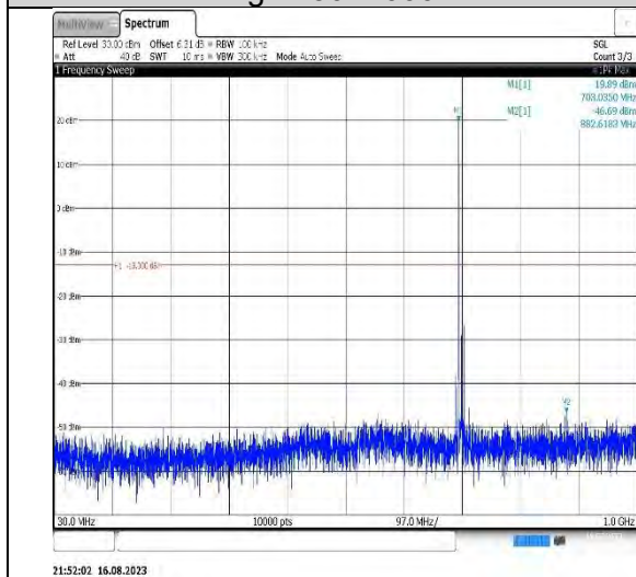
Band12-10MHz-QPSK-23095-1RB#0- Range1:30~1000MHz
