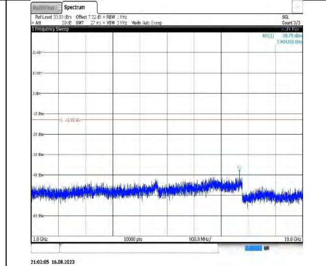
21:02:05 16.08.2023 Band12-1.4MHz-16QAM-23095-1RB#0-Range2:1000~10000MHz
