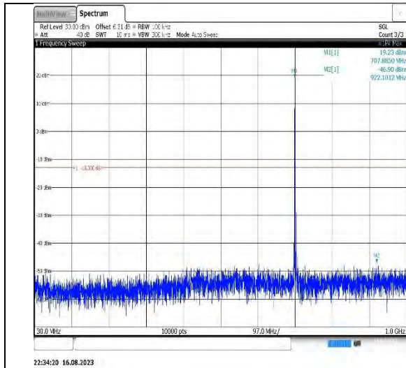
Band17-5MHz-16QAM-23825-1RB#0- Range1:30~1000MHz
