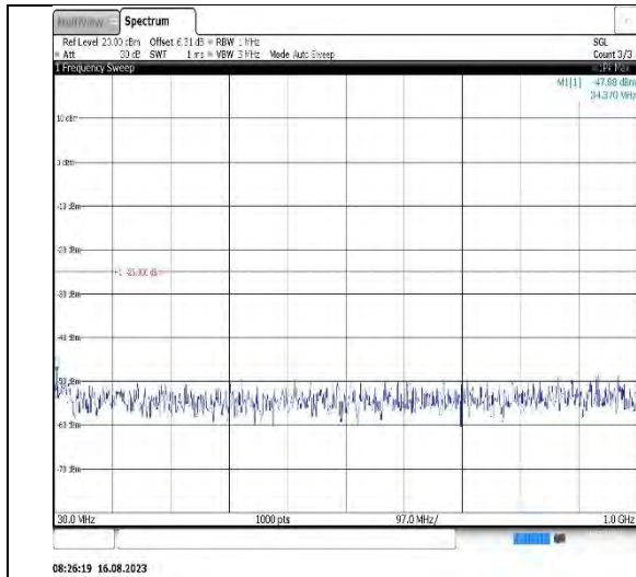
Band7-15MHz-16QAM-21375-1RB#0-Range1:30~1000MHz
