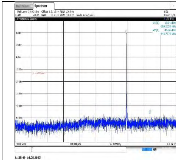
Band12-5MHz-QPSK-23095-1RB#0- Range1:30~1000MHz
