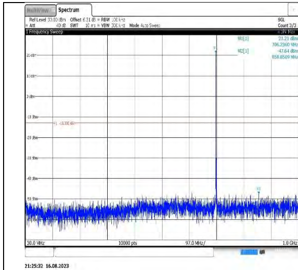
Band12-3MHz-QPSK-23165-1RB#0- Range1:30~1000MHz
