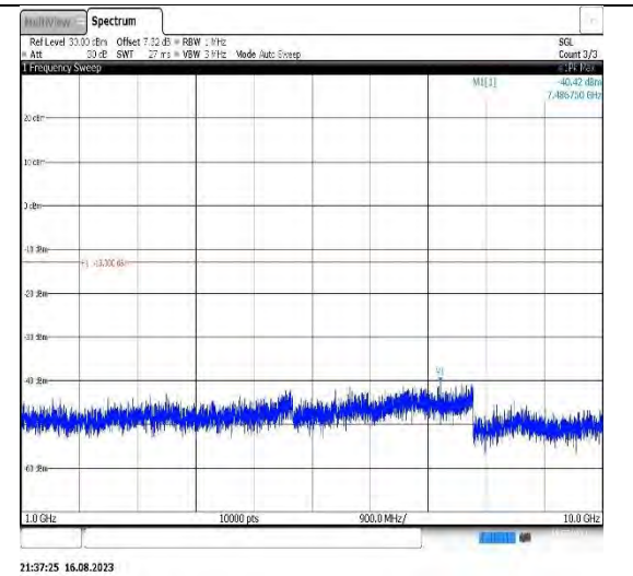
Band12-10MHz-QPSK-23060-1RB#0- Range2:1000~10000MHz
