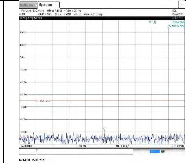
Band 14-5MHz-QPSK-23305-1RB#0- Range2:769~775MHz
