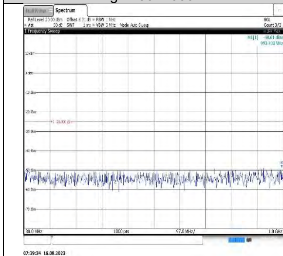
Band7-5MHz-16QAM-20775-1RB#0-Range1:30~1000MHz
