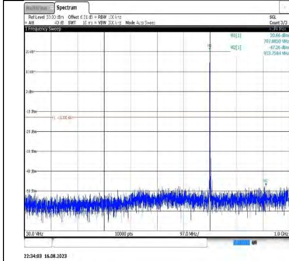
Band17-5MHz-QPSK-23790-1RB#0-Range1:30~1000MHz
