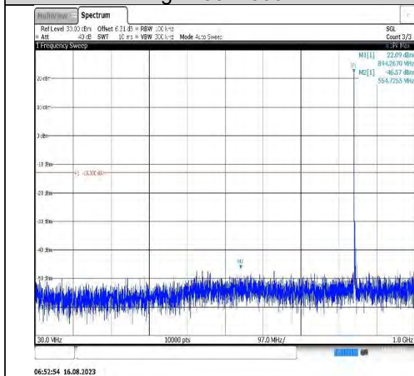
Band5-5MHz-16QAM-20625-1RB#0- Range1:30~1000MHz
