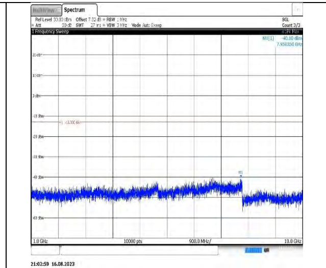
21:02:59 16.08.2023 Band12-1.4MHz-16QAM-23017-1RB#0-Range2:1000~10000MHz
