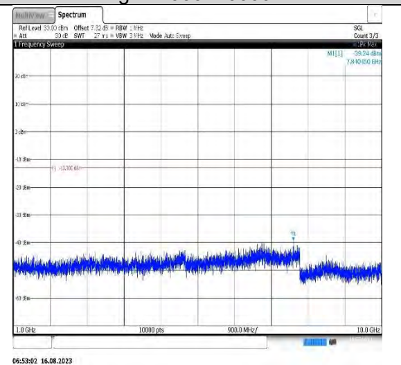
Band5-5MHz-16QAM-20625-1RB#0- Range2:1000~10000MHz
