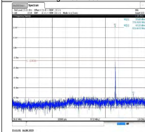
Band13-5MHz-16QAM-23230-1RB#0-Range1:30~1000MHz
