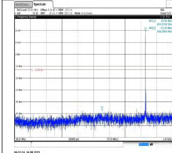
Band5-5MHz-16QAM-20625-1RB#0- Range1:30~1000MHz
