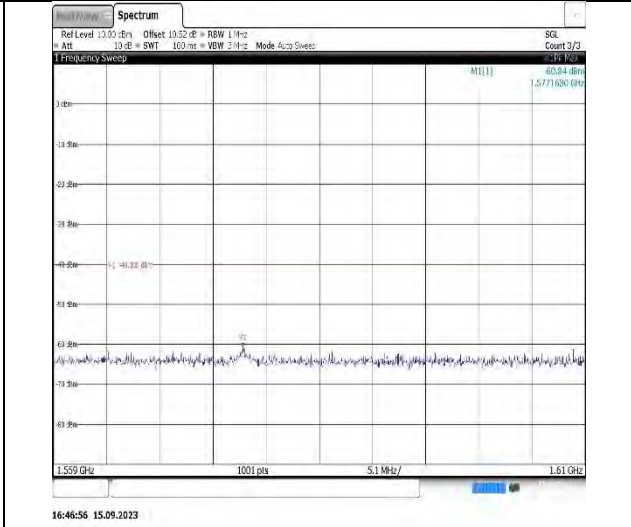
Band14-10MHz-QPSK-23330-1RB#0- Range5:1559~1610MHz
