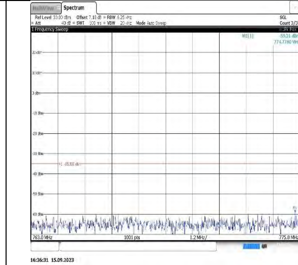
Band13-10MHz-QPSK-23230-1RB#0- Range2:763~775MHz
