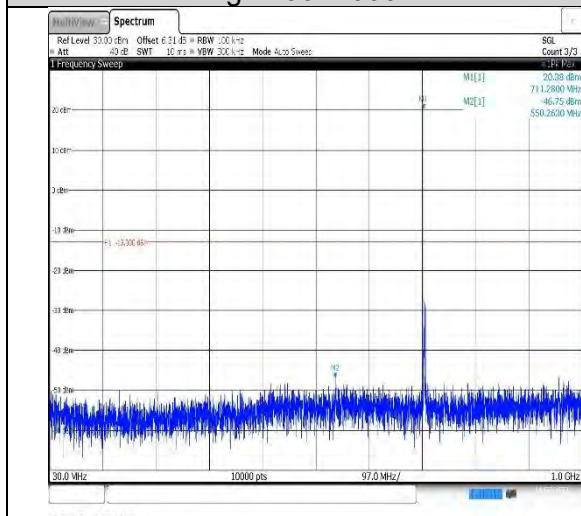
Band12-5MHz-QPSK-23155-1RB#0- Range1:30~1000MHz
