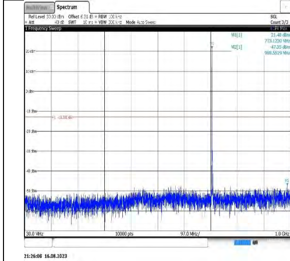
Band12-3MHz-16QAM-23025-1RB#0- Range1:30~1000MHz
