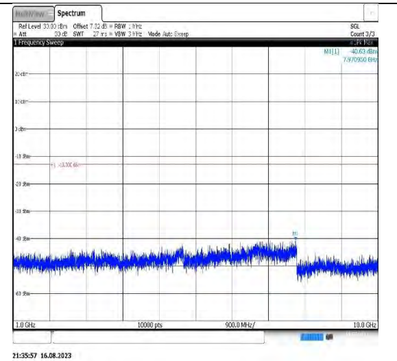
Band12-5MHz-QPSK-23095-1RB#0- Range2:1000~10000MHz
