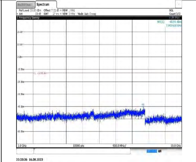
Band17-5MHz-QPSK-23790-1RB#0-Range2:1000~10000MHz
