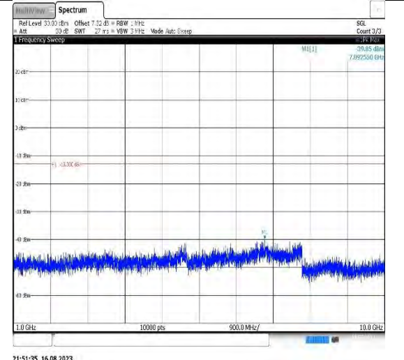
Band12-10MHz-QPSK-23095-1RB#0- Range2:1000~10000MHz
