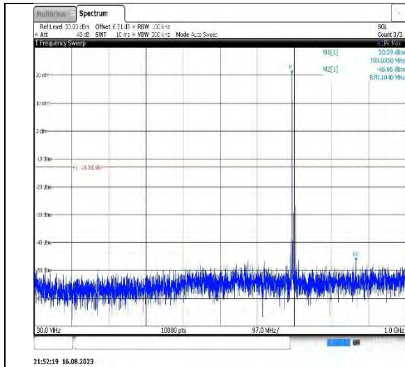
21:52:19 16.08.2023 Band 12-10MHz-16QAM-23130-1RB#0-Range1:30~1000MHz
