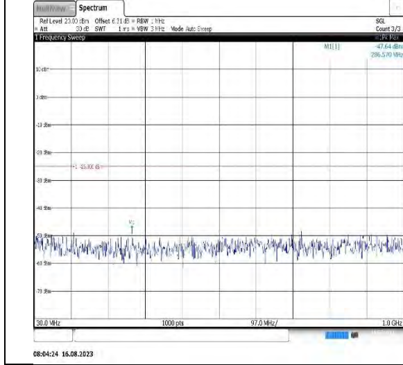
Band7-10MHz-QPSK-21400-1RB#0-Range1:30~1000MHz
