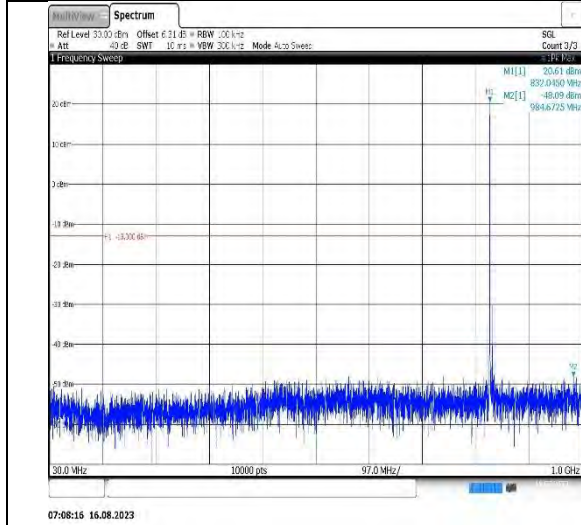
Band5-10MHz-16QAM-20525-1RB#0- Range1:30~1000MHz
