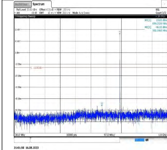
21:01:58 16.08.2023 Band12-1.4MHz-16QAM-23095-1RB#0-Range1:30~1000MHz
