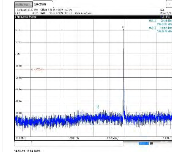
Band12-10MHz-QPSK-23095-1RB#0- Range1:30~1000MHz
