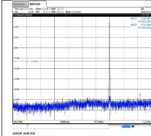
Band17-10MHz-QPSK-23780-1RB#0- Range1:30~1000MHz
