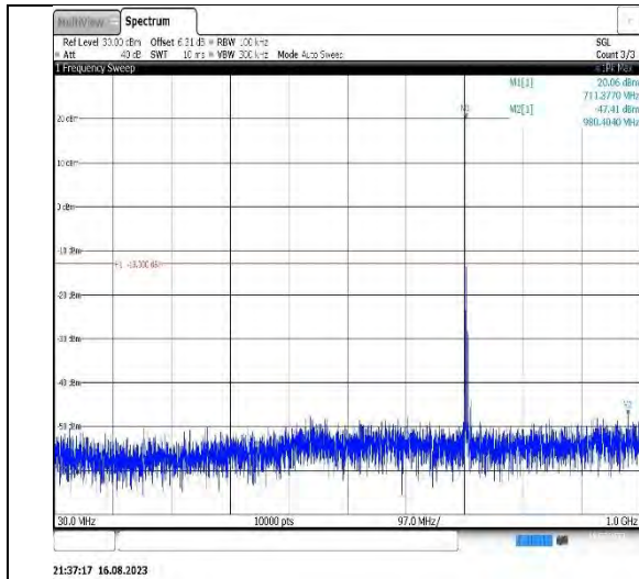
Band12-10MHz-QPSK-23060-1RB#0- Range1:30~1000MHz
