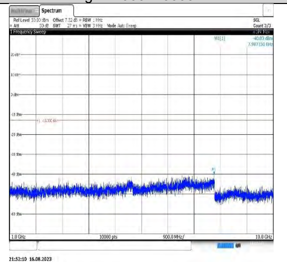
Band12-10MHz-QPSK-23095-1RB#0- Range2:1000~10000MHz
