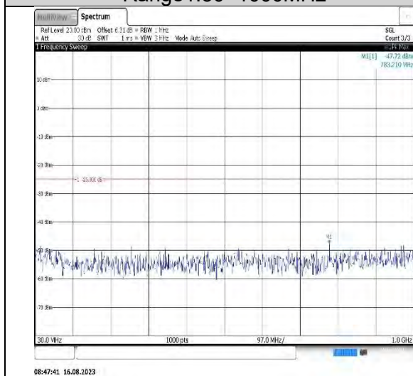
Band7-20MHz-QPSK-20850-1RB#0-Range1:30~1000MHz
