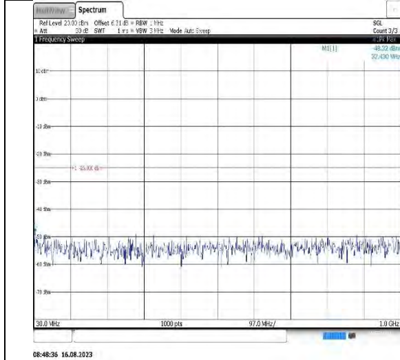
Band7-20MHz-16QAM-21350-1RB#0-Range1:30~1000MHz
