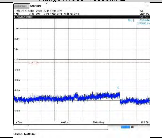
Band14-5MHz-16QAM-23305-1RB#0- Range4:1000~10000MHz
