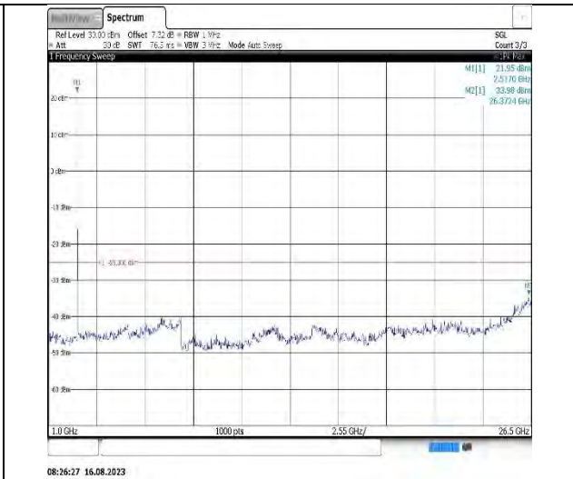
Band7-15MHz-16QAM-21375-1RB#0-Range2:1000~26500MHz
