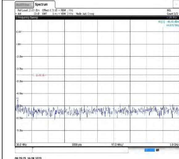
Band7-15MHz-QPSK-21100-1RB#0-Range1:30~1000MHz
