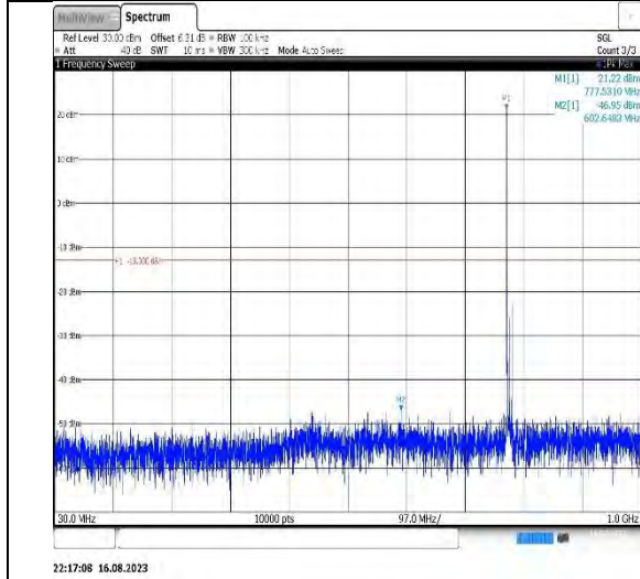
Band13-10MHz-QPSK-23230-1RB#0- Range1:30~1000MHz
