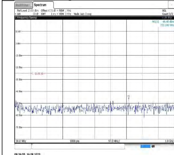
Band7-20MHz-QPSK-20850-1RB#0-Range1:30~1000MHz
