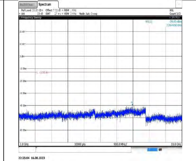
Band17-10MHz-QPSK-23780-1RB#0- Range2:1000~10000MHz
