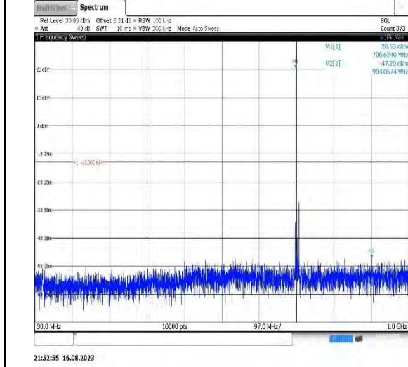
21:52:55 16.08.2023 Band 13-5MHz-QPSK-23205-1RB#0-Range1:30~1000MHz
