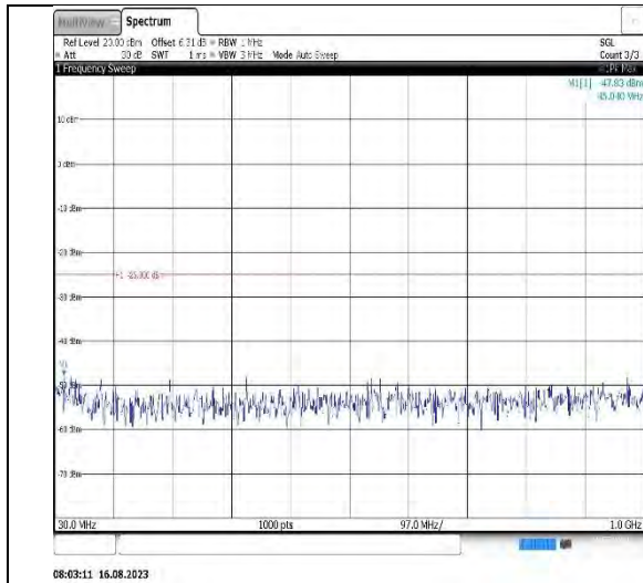
Band7-10MHz-QPSK-21100-1RB#0-Range1:30~1000MHz
