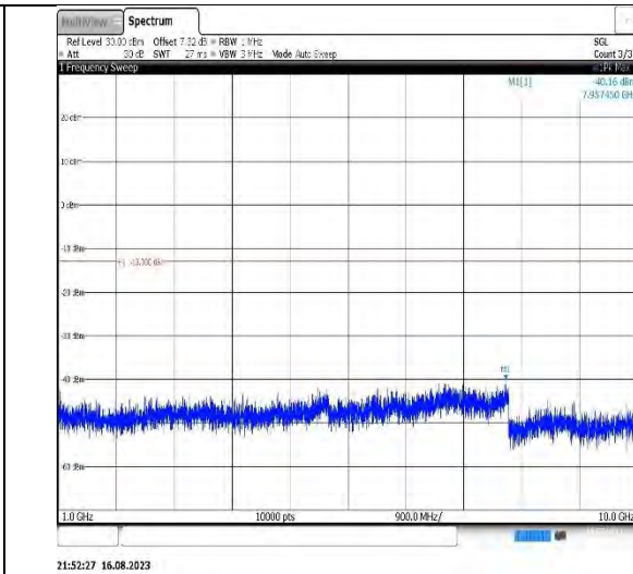
21:52:27 16.08.2023 Band 12-10MHz-16QAM-23130-1RB#0-Range2:1000~10000MHz
