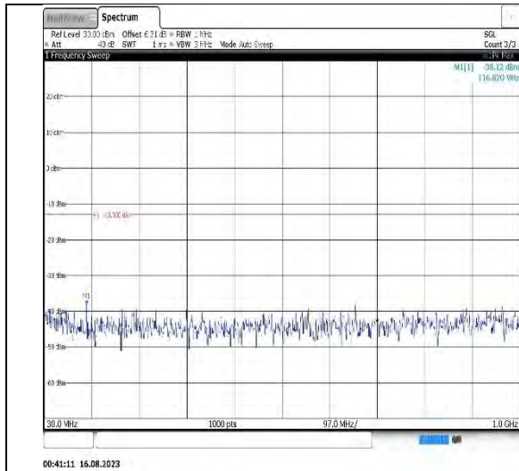
Band2-5MHz-QPSK-18900-1RB#0-Range1:30~1000MHz
