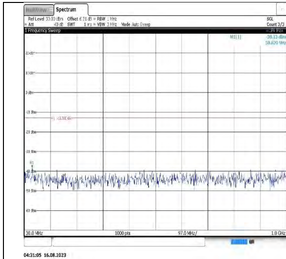
Band4-15MHz-16QAM-20025-1RB#0-Range1:30~1000MHz
