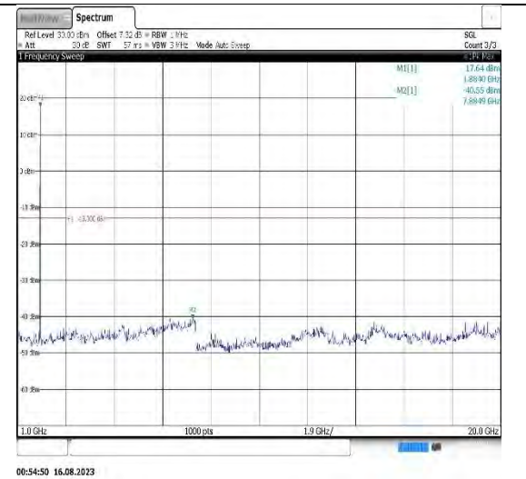
Band2-10MHz-16QAM-19150-1RB#0- Range2:1000~20000MHz
