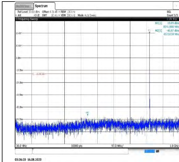
Band5-1.4MHz-QPSK-20525-1RB#0- Range1:30~1000MHz
