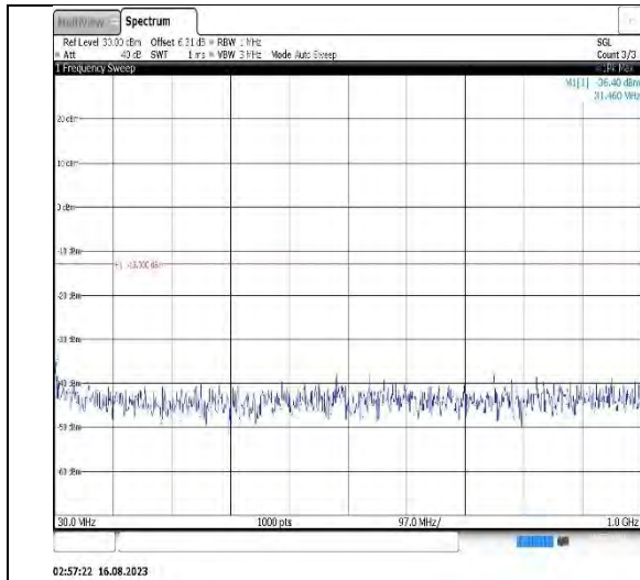
Band4-3MHz-QPSK-20175-1RB#0- Range1:30~1000MHz
