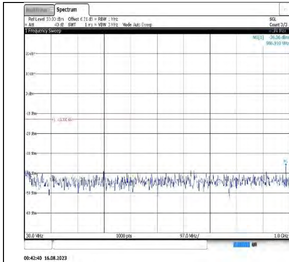
Band2-10MHz-QPSK-18650-1RB#0-Range1:30~1000MHz
