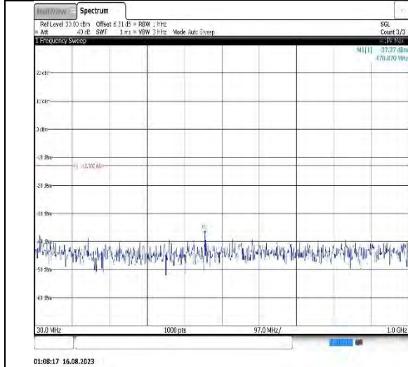
Band2-15MHz-QPSK-18675-1RB#0- Range1:30~1000MHz
