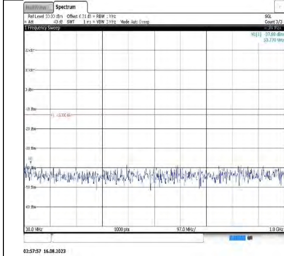
Band4-3MHz-QPSK-20385-1RB#0- Range1:30~1000MHz
