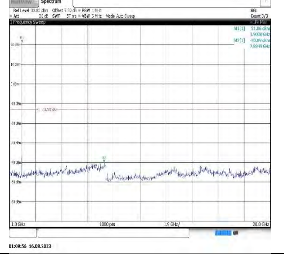
Band2-15MHz-16QAM-19125-1RB#0-Range2:1000~20000MHz
