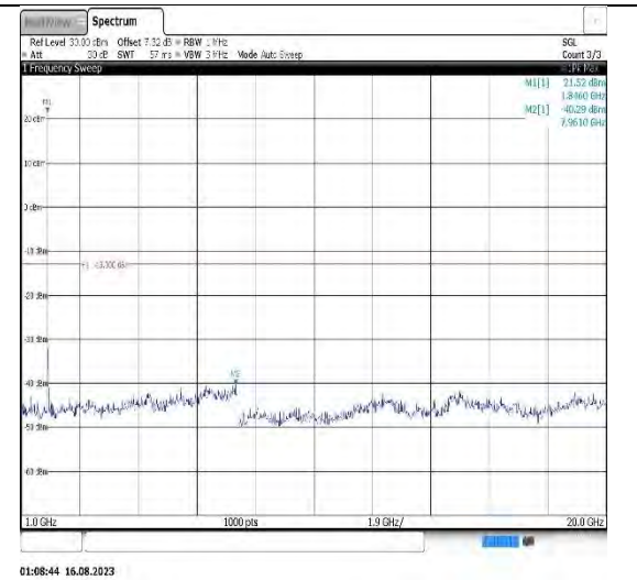
Band2-15MHz-16QAM-18900-1RB#0-Range2:1000~20000MHz
