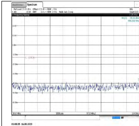
Band2-15MHz-16QAM-18900-1RB#0-Range1:30~1000MHz
