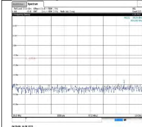
Band4-15MHz-16QAM-20175-1RB#0-Range1:30~1000MHz
