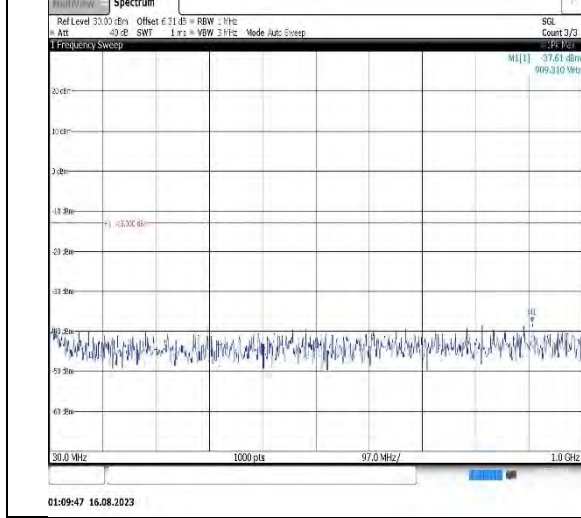
Band2-15MHz-16QAM-19125-1RB#0-Range1:30~1000MHz
