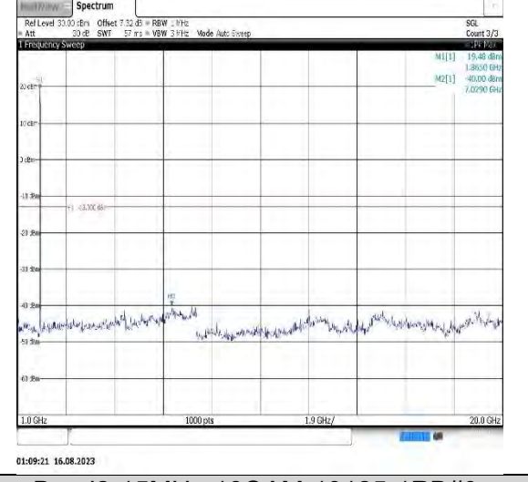
Band2-15MHz-16QAM-19125-1RB#0-Range2:1000~20000MHz
