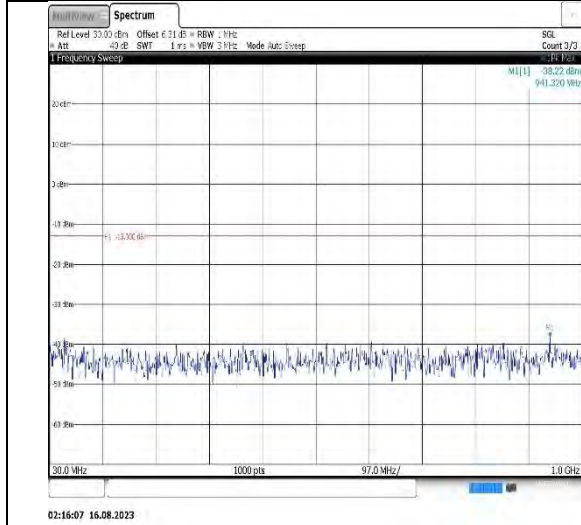
Band4-1.4MHz-16QAM-19957-1RB#0-Range1:30~1000MHz
