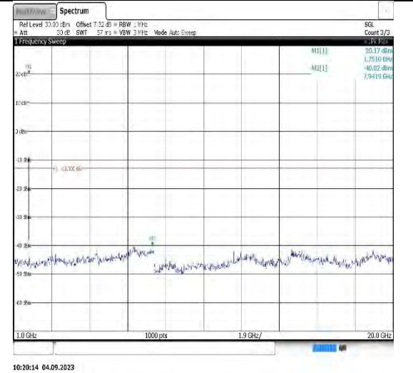
Band4-10MHz-16QAM-20350-1RB#0- Range2:1000~20000MHz
