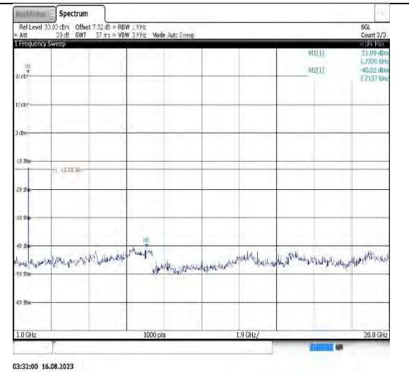
Band4-5MHz-16QAM-20375-1RB#0-Range2:1000~20000MHz
