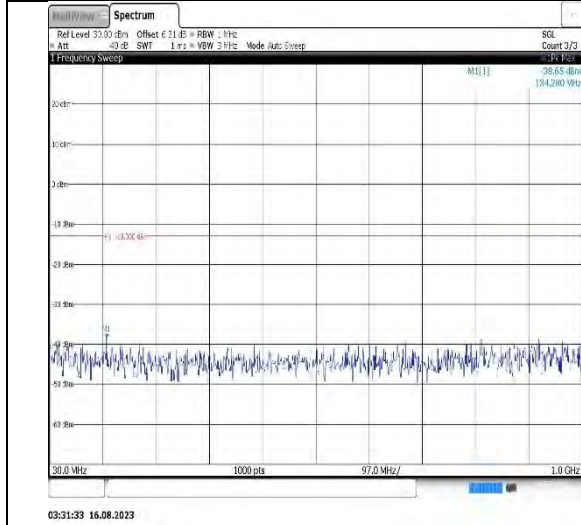
Band4-5MHz-QPSK-19975-1RB#0-Range1:30~1000MHz
