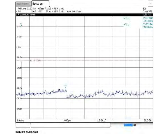
Band4-1.4MHz-16QAM-19957-1RB#0-Range2:1000~20000MHz
