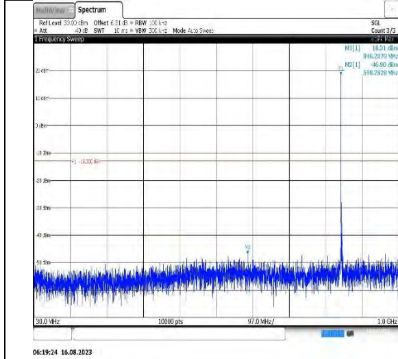
Band5-5MHz-QPSK-20425-1RB#0- Range1:30~1000MHz
