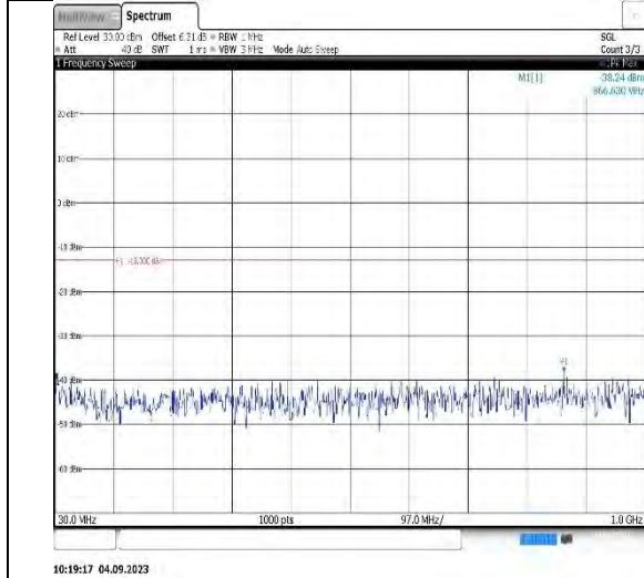
Band4-10MHz-16QAM-20350-1RB#0- Range1:30~1000MHz
