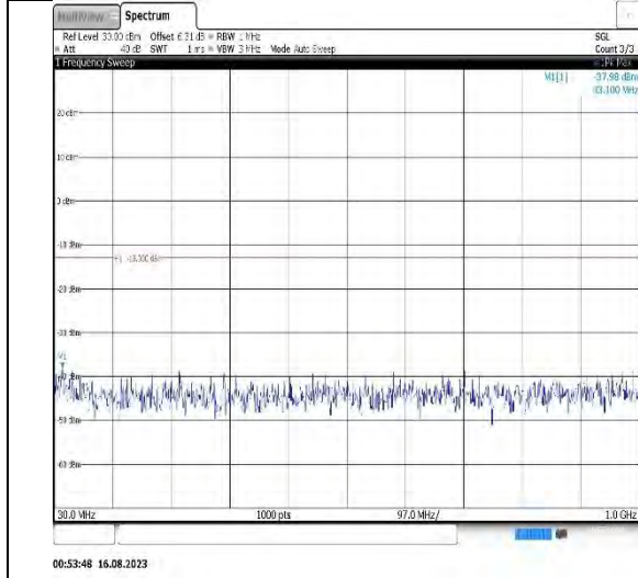
Band2-10MHz-QPSK-18900-1RB#0-Range1:30~1000MHz
