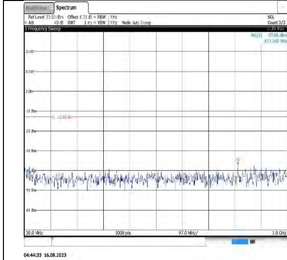
Band4-20MHz-16QAM-20050-1RB#0-Range1:30~1000MHz
