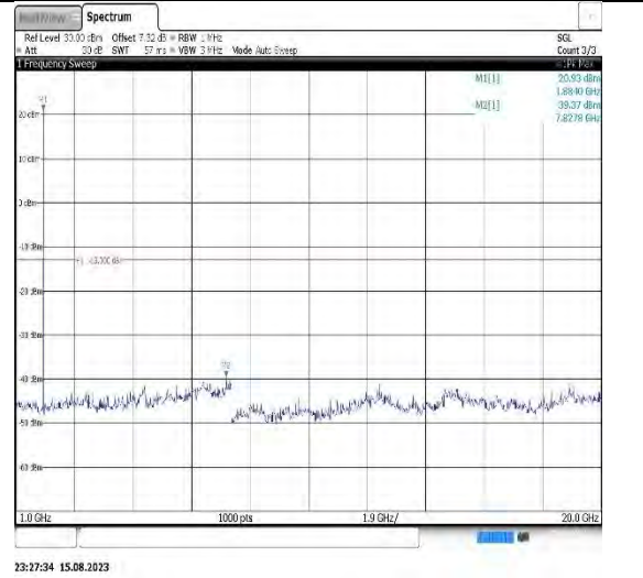
Band2-1.4MHz-16QAM-18900-1RB#0- Range2:1000~20000MHz
