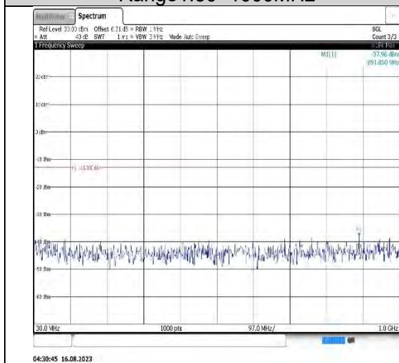
Band4-15MHz-16QAM-20175-1RB#0-Range1:30~1000MHz
