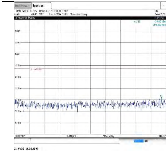
Band2-20MHz-16QAM-18700-1RB#0- Range1:30~1000MHz
