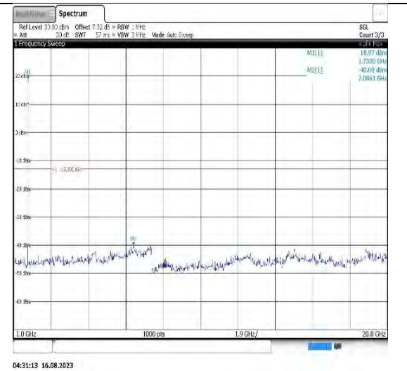
Band4-15MHz-16QAM-20025-1RB#0-Range2:1000~20000MHz
