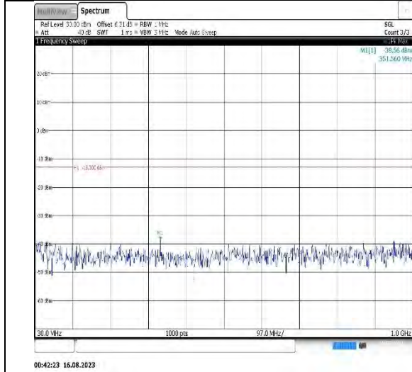
Band2-5MHz-QPSK-19175-1RB#0-Range1:30~1000MHz
