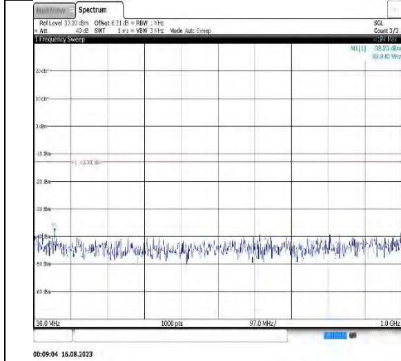
Band2-3MHz-16QAM-18615-1RB#0-Range1:30~1000MHz
