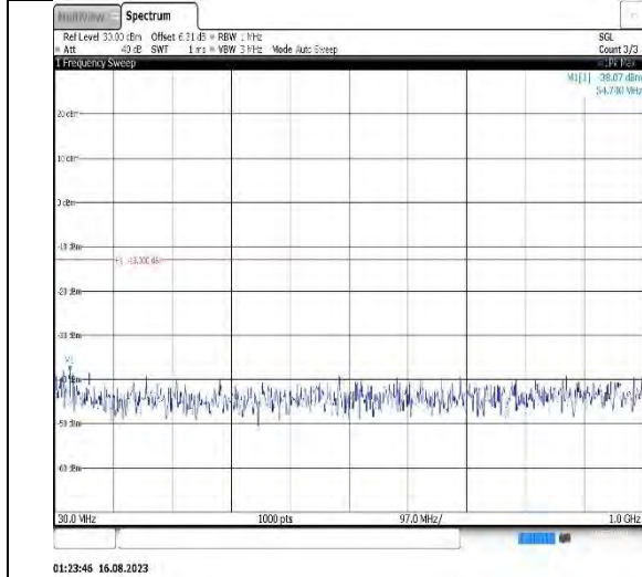
Band2-20MHz-16QAM-18900-1RB#0- Range1:30~1000MHz
