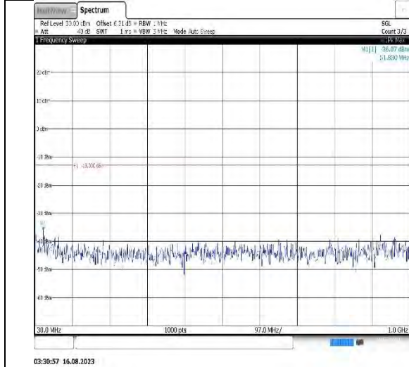
Band4-5MHz-QPSK-20175-1RB#0-Range1:30~1000MHz
