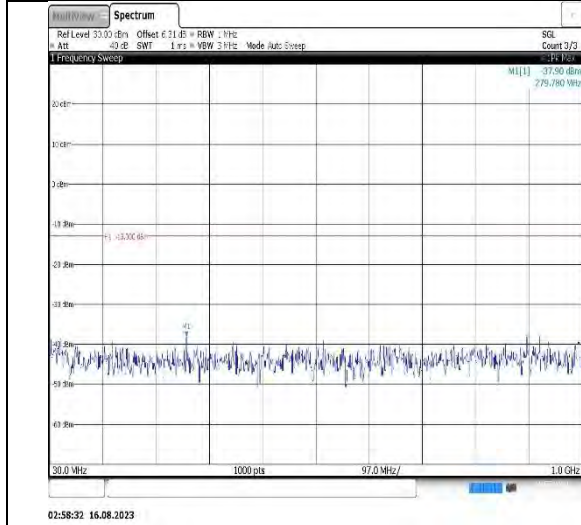
Band4-3MHz-QPSK-20175-1RB#0- Range1:30~1000MHz
