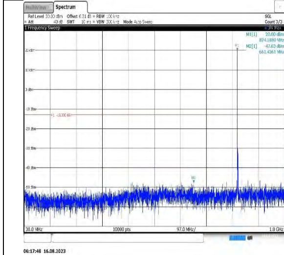
Band5-3MHz-QPSK-20525-1RB#0- Range1:30~1000MHz
