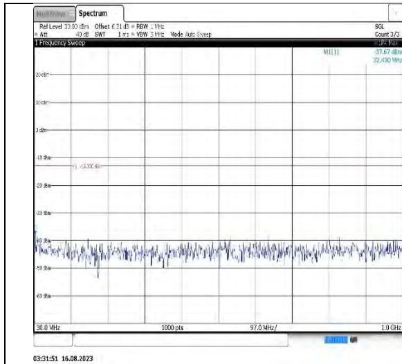
Band4-5MHz-16QAM-20375-1RB#0-Range1:30~1000MHz
