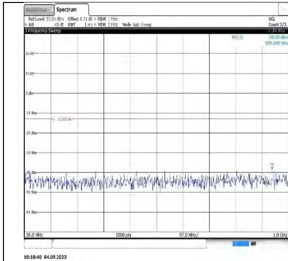
Band4-10MHz-16QAM-20175-1RB#0- Range1:30~1000MHz
