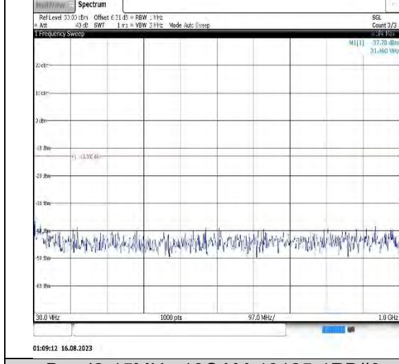
Band2-15MHz-16QAM-19125-1RB#0-Range1:30~1000MHz
