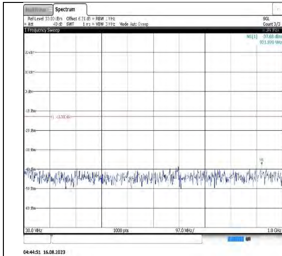
Band4-20MHz-QPSK-20300-1RB#0-Range1:30~1000MHz
