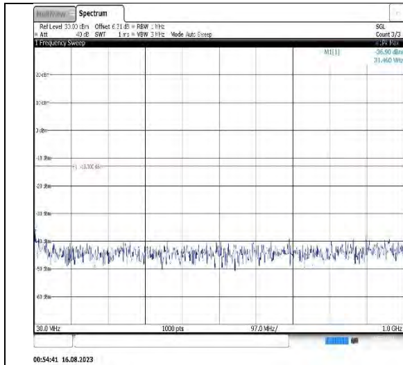
Band2-10MHz-16QAM-19150-1RB#0- Range1:30~1000MHz
