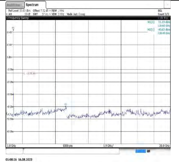
Band2-15MHz-QPSK-18675-1RB#0- Range2:1000~20000MHz
