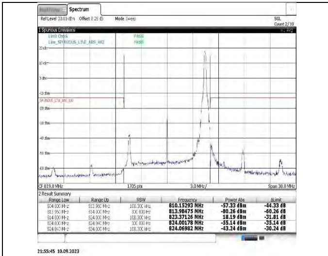
Band26(824-849)-10MHz-16QAM-26840-1RB#0
