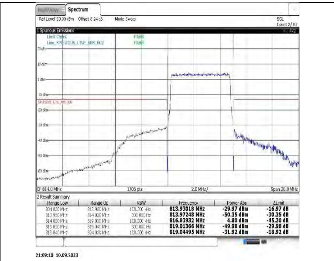
Band26(814-824)-5MHz-QPSK-26765-25RB#0
