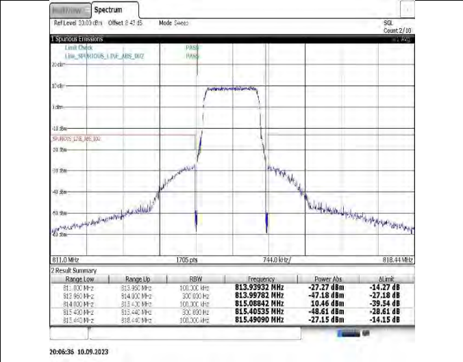
Band26(814-824)-1.4MHz-16QAM-26783-6RB#0
