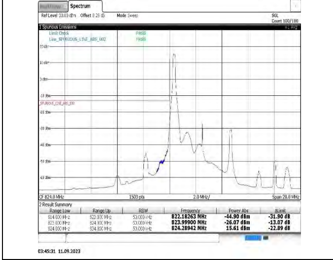
Band26(824-849)-5MHz-QPSK-27015-1RB#24
