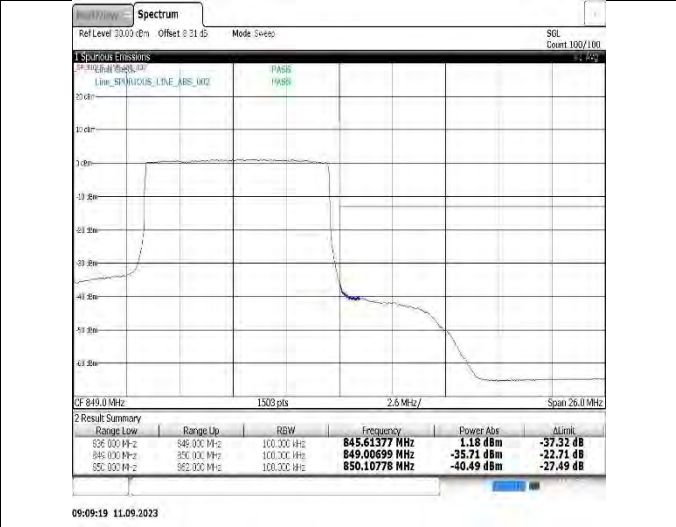
Band26(824-849)-15MHz-QPSK-26865-75RB#0
