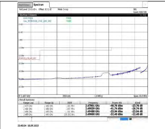
Band41-20MHz-QPSK-39750-100RB#0
