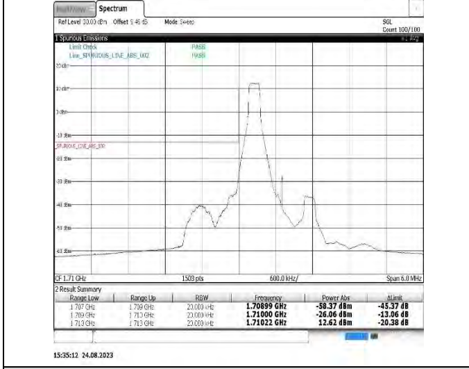
Band66-1.4MHz-QPSK-132665-1RB#5
