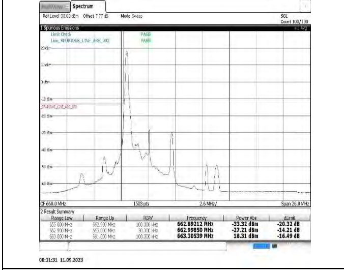
Band71-5MHz-16QAM-133147-1RB#0
