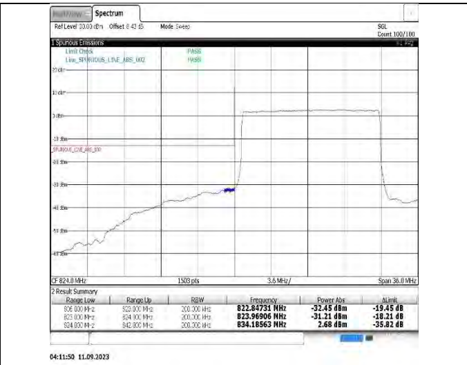
Band26(824-849)-15MHz-QPSK-26965-75RB#0
