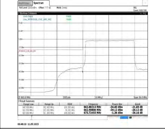
Band71-15MHz-16QAM-133197-75RB#0
