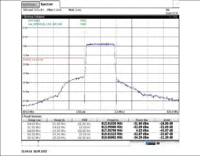
Band26(814-824)-5MHz-16QAM-26765-25RB#0
