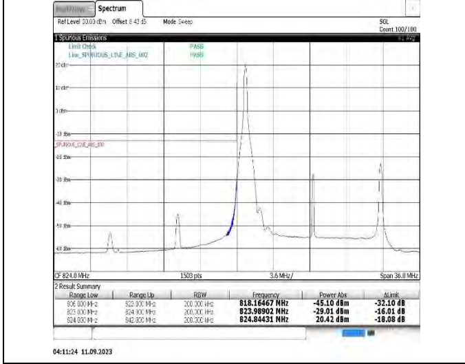
Band26(824-849)-15MHz-16QAM-26865-1RB#0
