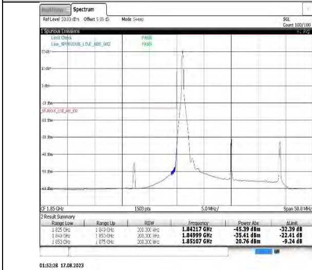
Band25-20MHz-16QAM-26140-1RB#99
