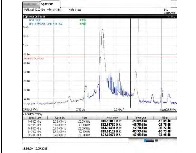
Band26(814-824)-5MHz-16QAM-26765-1RB#24
