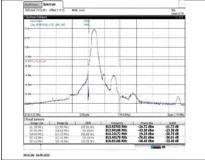
Band26(814-824)-1.4MHz-QPSK-26783-1RB#5
