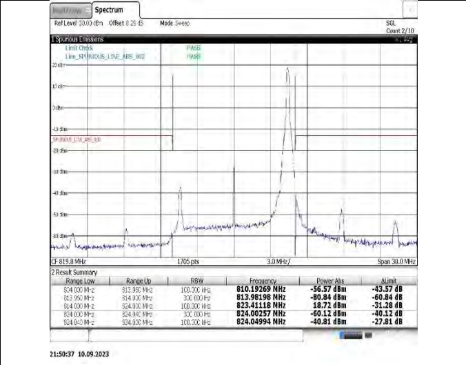
Band26(824-849)-10MHz-QPSK-26990-1RB#49
