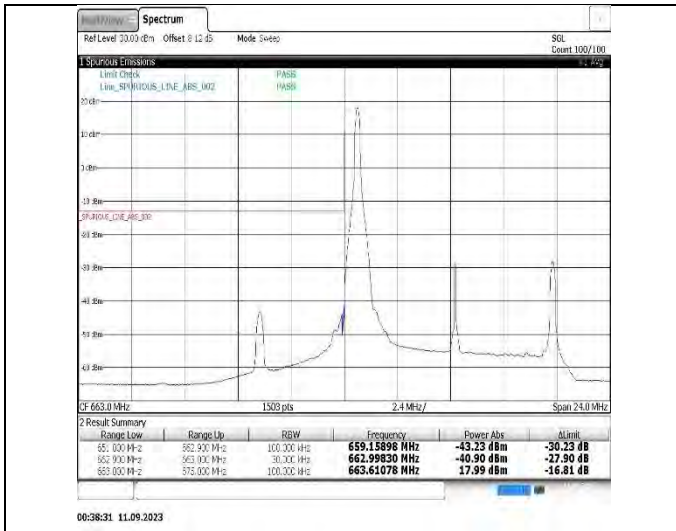
Band71-10MHz-16QAM-133422-1RB#49
