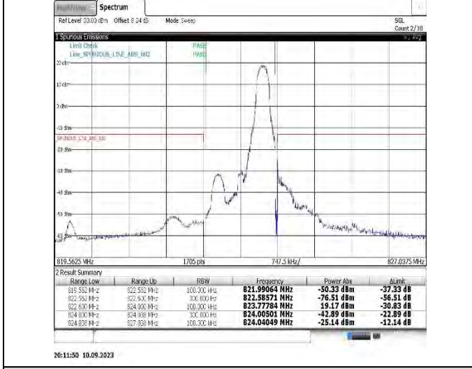
Band26(824-849)-1.4MHz-QPSK-26797-1RB#0
