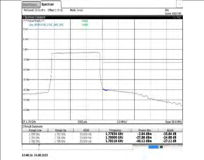
Band66-15MHz-QPSK-132047-75RB#0
