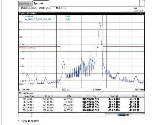
Band26(824-849)-5MHz-QPSK-26815-1RB#0
