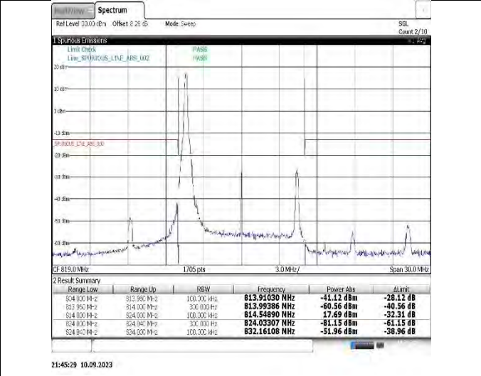
Band26(814-824)-10MHz-16QAM-26740-50RB#0
