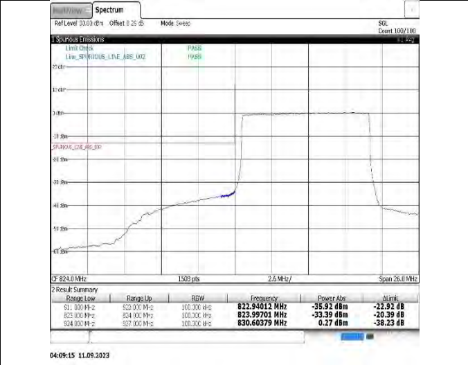
Band26(824-849)-10MHz-16QAM-26990-50RB#0
