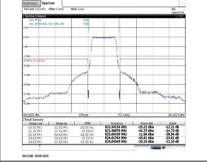
Band26(824-849)-1.4MHz-QPSK-26797-6RB#0
