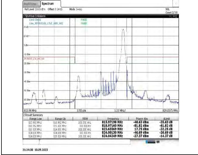
Band26(824-849)-5MHz-16QAM-26815-1RB#0
