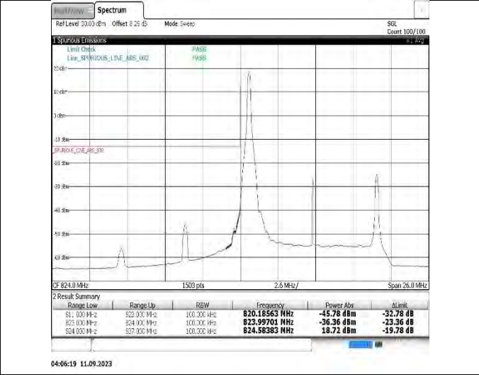
Band26(824-849)-10MHz-16QAM-26740-1RB#0
