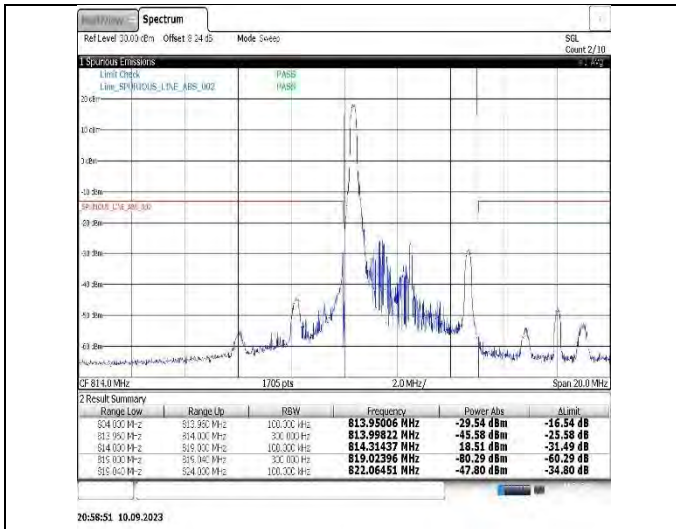
Band26(814-824)-5MHz-QPSK-26765-1RB#24
