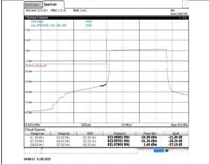
Band26(814-824)-10MHz-16QAM-26740-1RB#49
