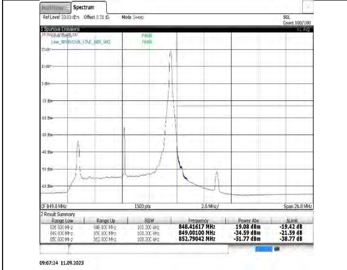
Band26(824-849)-15MHz-QPSK-26865-1RB#0
