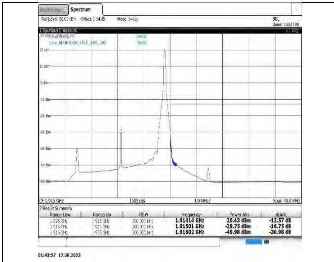
Band25-15MHz-16QAM-26115-1RB#0
