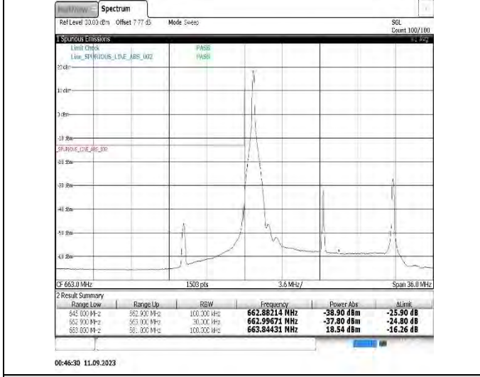
Band71-15MHz-16QAM-133197-1RB#0
