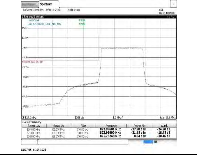
Band26(824-849)-3MHz-16QAM-27025-15RB#0
