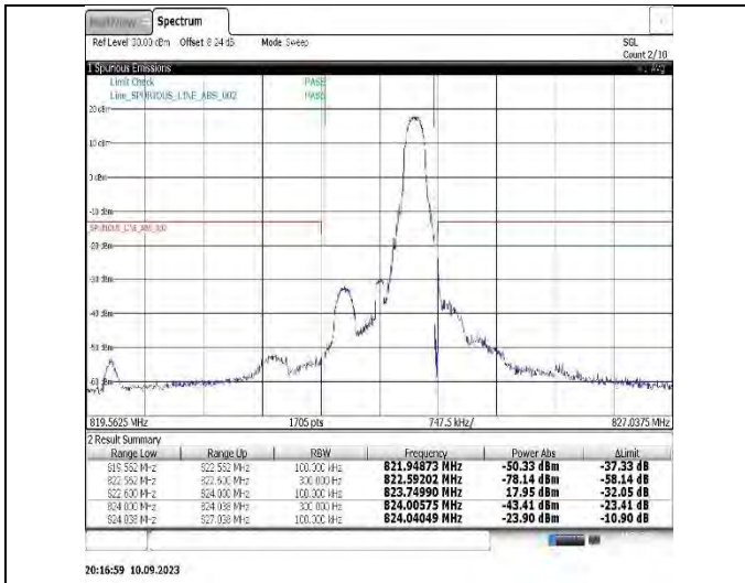
Band26(824-849)-1.4MHz-16QAM-26797-1RB#0
