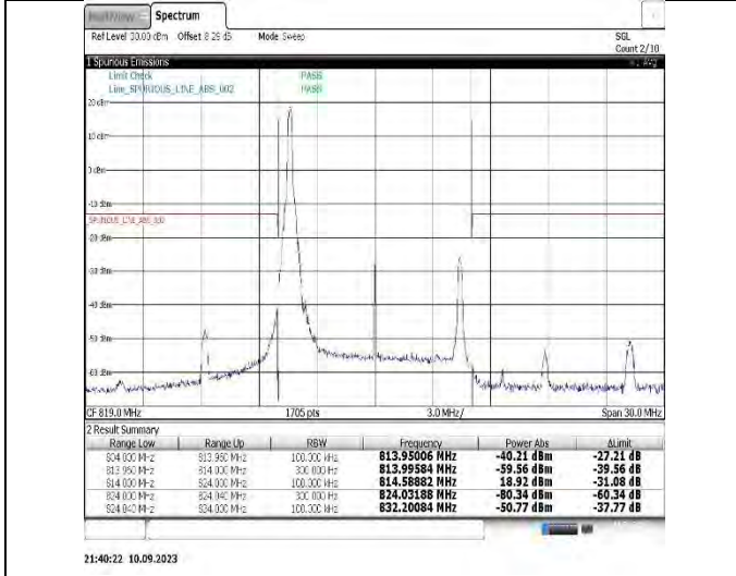
Band26(814-824)-10MHz-QPSK-26740-50RB#0
