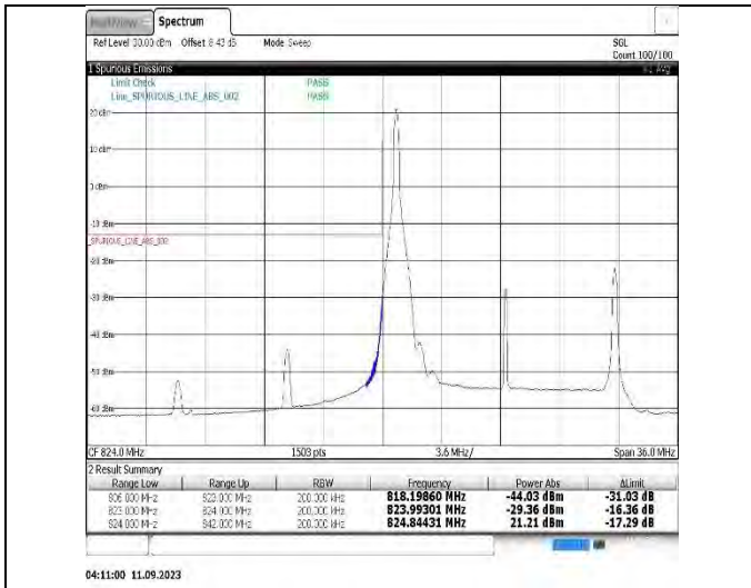
Band26(824-849)-15MHz-QPSK-26965-1RB#74
