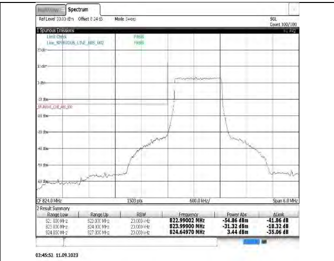
Band26(824-849)-1.4MHz-QPSK-27033-6RB#0
