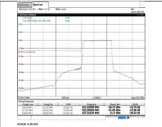
Band26(824-849)-5MHz-16QAM-27015-25RB#0
