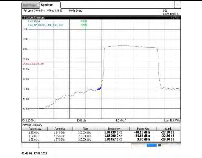
Band25-15MHz-QPSK-26615-75RB#0
