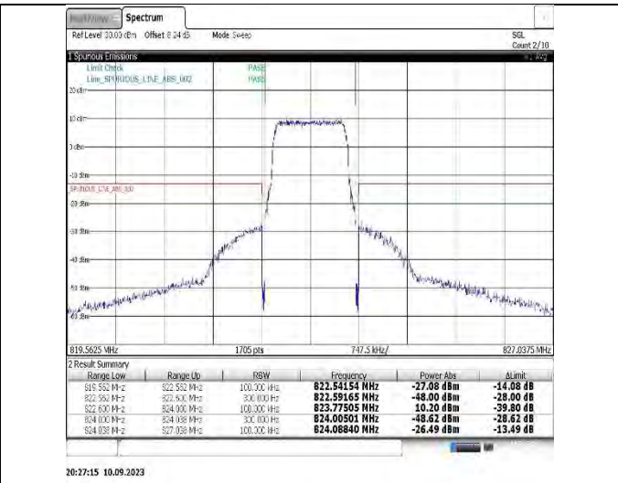
Band26(824-849)-1.4MHz-16QAM-26797-6RB#0
