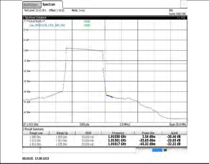
Band25-5MHz-16QAM-26065-25RB#0
