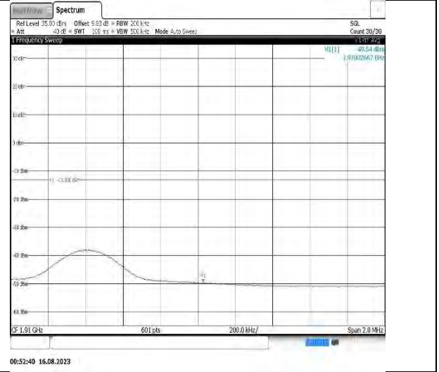
Band2-10MHz-QPSK-19150-50RB#0
