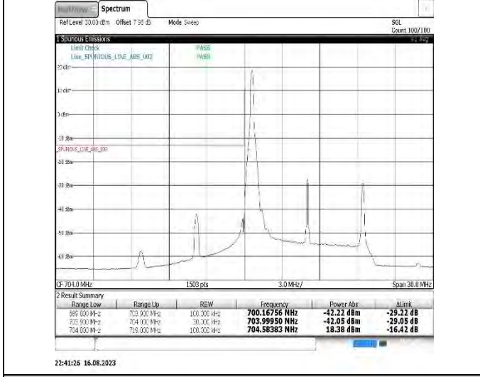
Band17-10MHz-16QAM-23800-1RB#49
