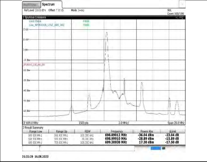
Band12-10MHz-QPSK-23060-1RB#0
