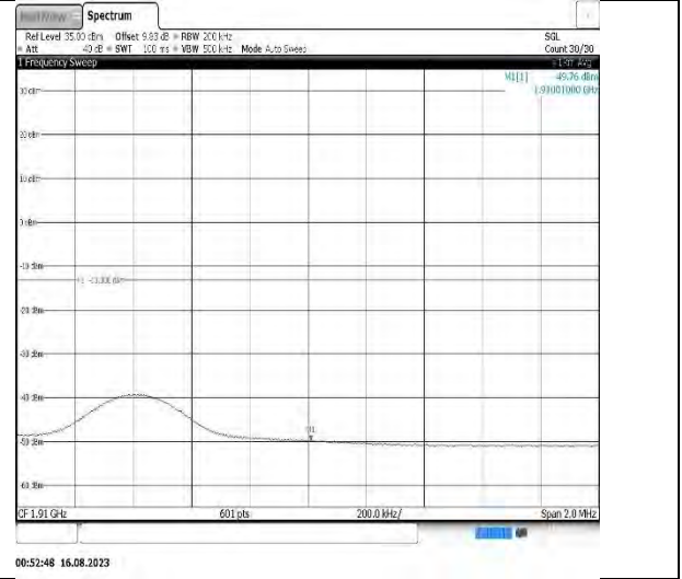
Band2-10MHz-16QAM-19150-50RB#0
