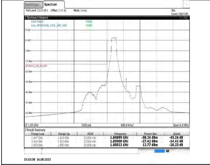
Band25-1.4MHz-QPSK-26683-1RB#5
