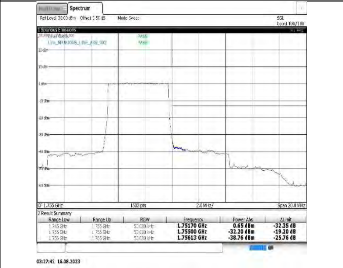
Band4-5MHz-16QAM-19975-25RB#0
