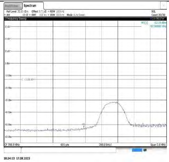
Band14-5MHz-16QAM-23355-1RB#0
