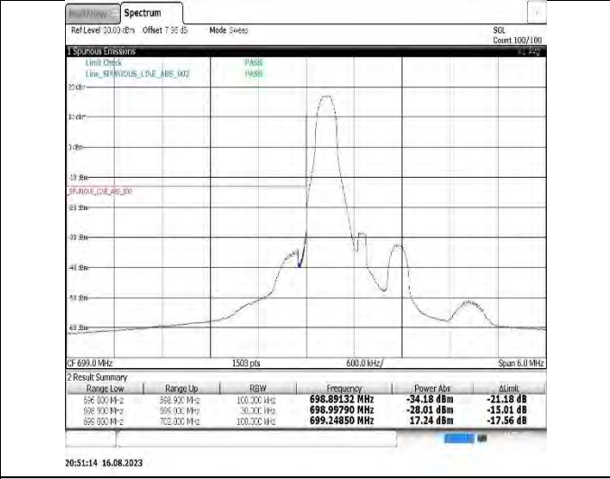
Band12-1.4MHz-16QAM-23017-1RB#5
