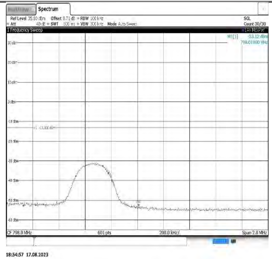
Band14-5MHz-16QAM-23355-25RB#0
