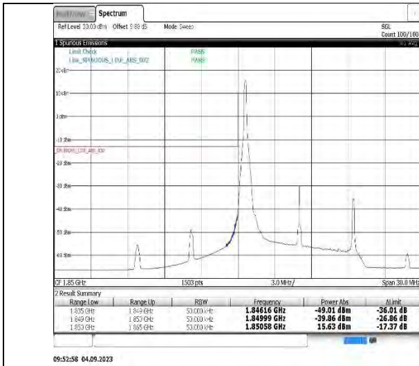
Band2-10MHz-16QAM-18650-50RB#0
