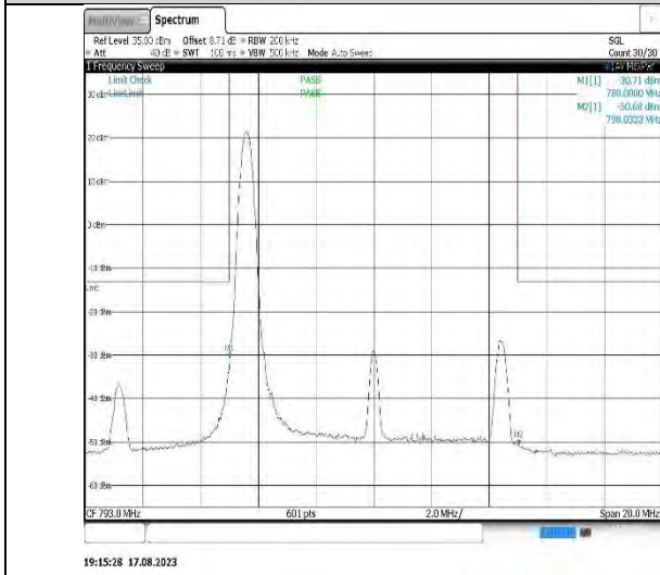
Band14-10MHz-QPSK-23330-50RB#0
