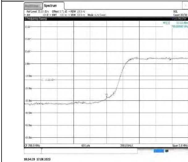
Band14-5MHz-16QAM-23355-1RB#24
