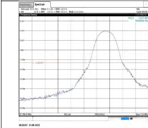
Band14-5MHz-16QAM-23305-25RB#0
