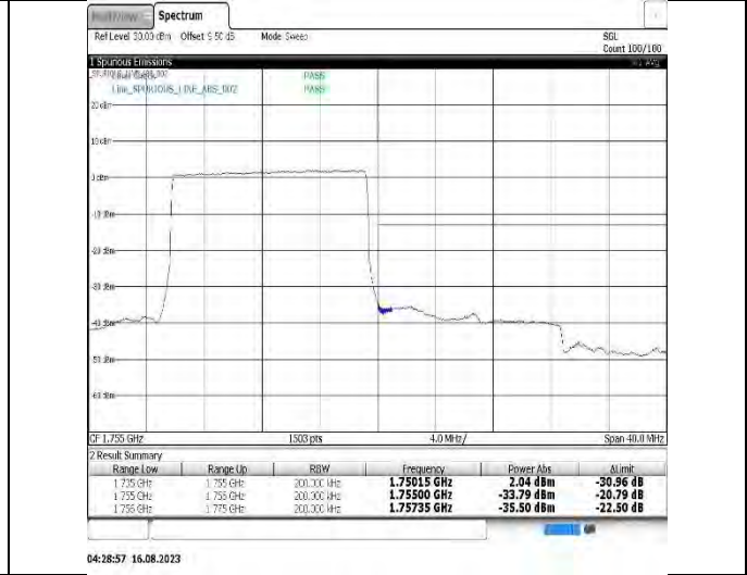
Band4-15MHz-16QAM-20025-75RB#0
