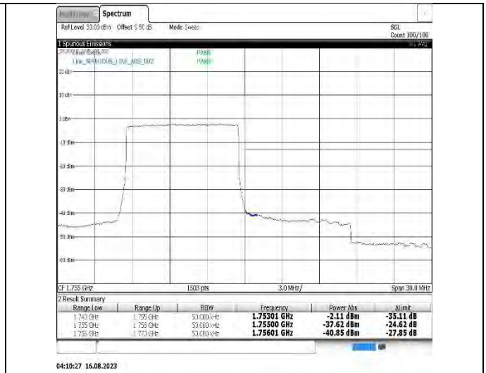
Band4-10MHz-16QAM-20000-50RB#0
