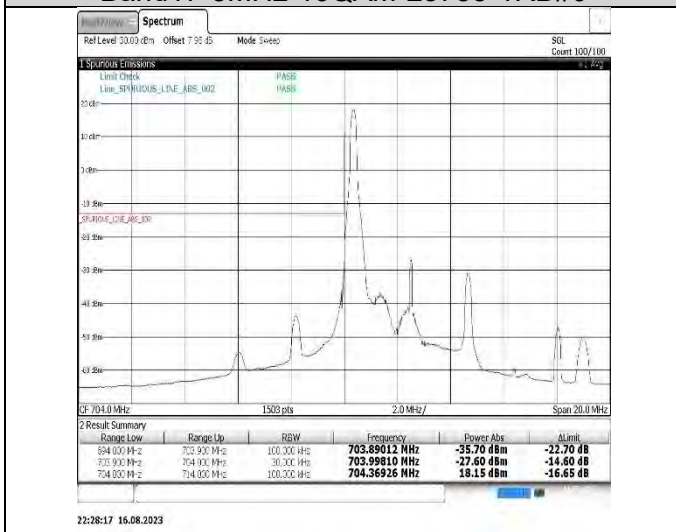
Band17-10MHz-QPSK-23780-1RB#0
