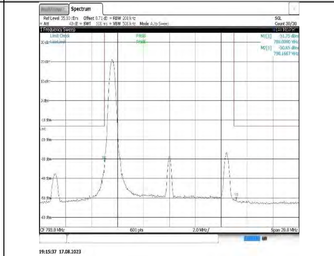
Band14-10MHz-16QAM-23330-50RB#0
