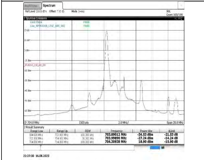
Band17-5MHz-16QAM-23755-1RB#0
