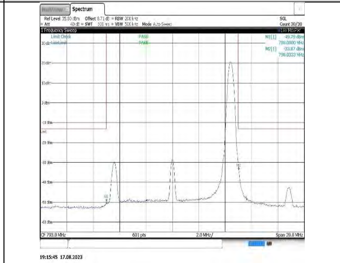
Band14-10MHz-16QAM-23330-1RB#0
