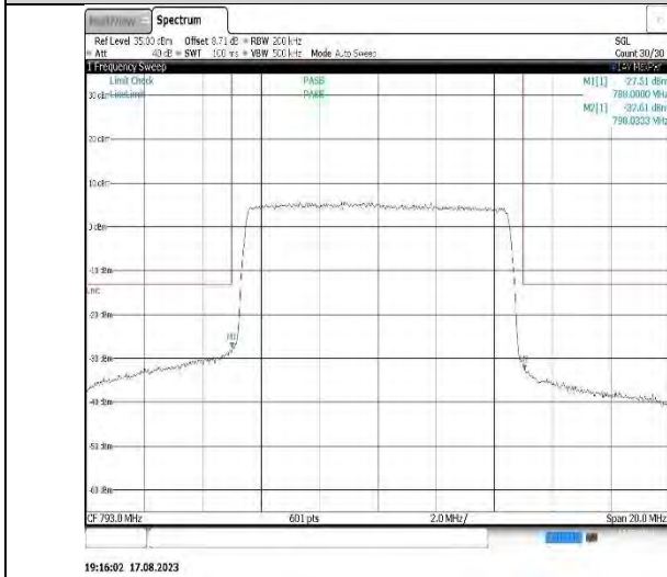
Band14-10MHz-16QAM-23330-1RB#49
