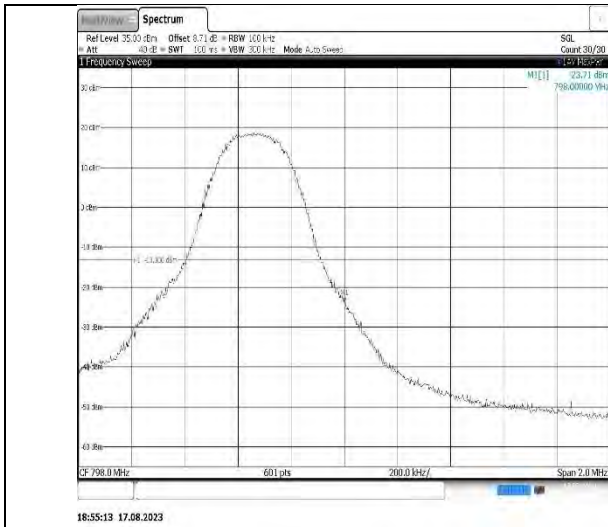
Band14-10MHz-QPSK-23330-1RB#0
