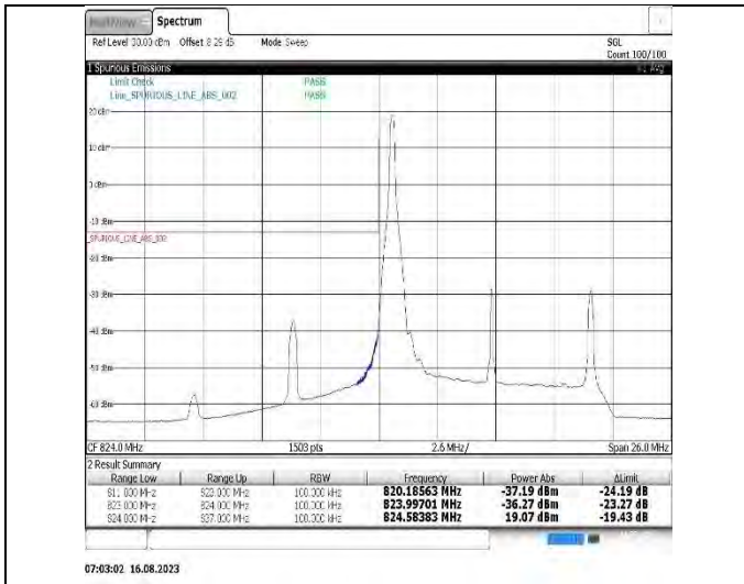
Band5-10MHz-16QAM-20450-1RB#0
