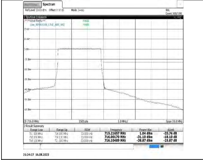
Band12-5MHz-QPSK-23035-25RB#0
