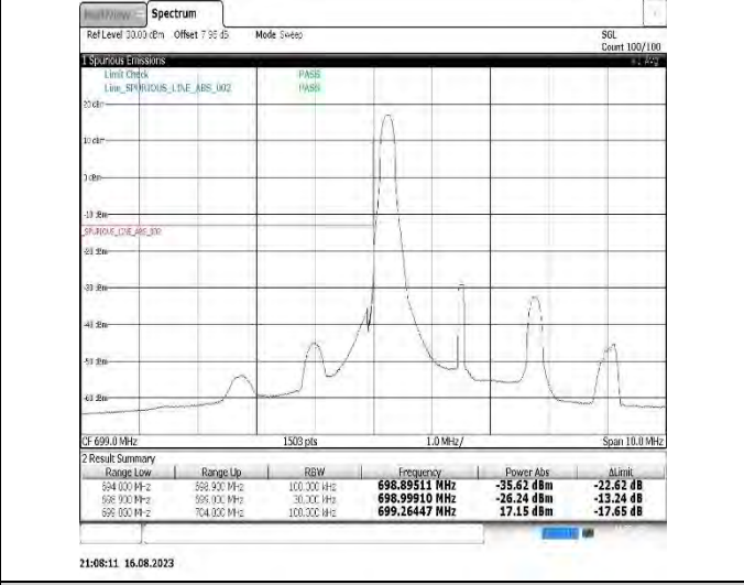
Band12-3MHz-16QAM-23165-1RB#14
