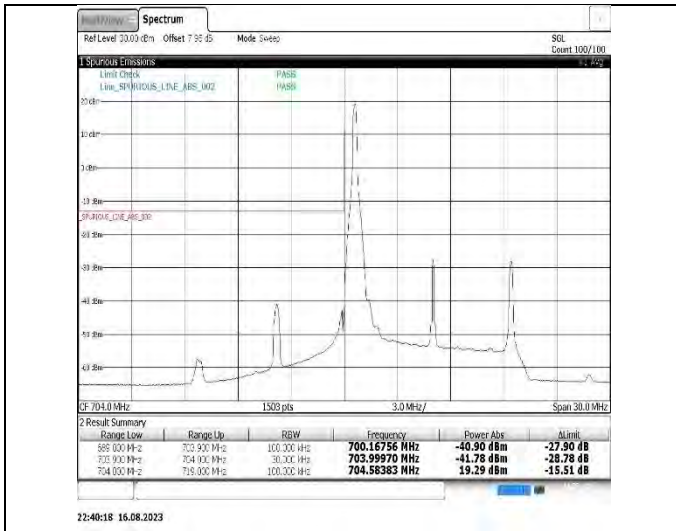
Band17-10MHz-QPSK-23800-1RB#49
