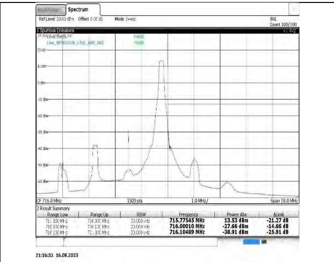
Band12-5MHz-QPSK-23035-1RB#0
