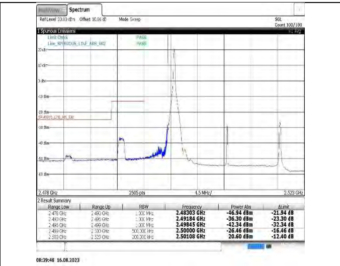
Band7-20MHz-16QAM-21350-1RB#99
