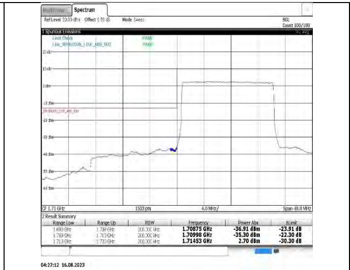
Band4-15MHz-QPSK-20325-75RB#0
